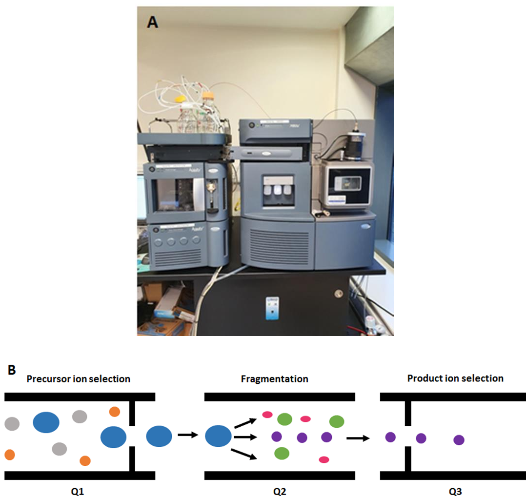
Figure 1.6: Targeted mass spectrometry. Photo A shows a Waters ACQUITY ultra-high performance liquid chromatography coupled to a Xevo triple quadrupole mass spectrometer (UPLC-TQ-MS) used for the targeted experiments describes in this thesis. B shows a schematic of a triple quadrupole mass spectrometer used for targeted analysis and multiple reaction monitoring.
