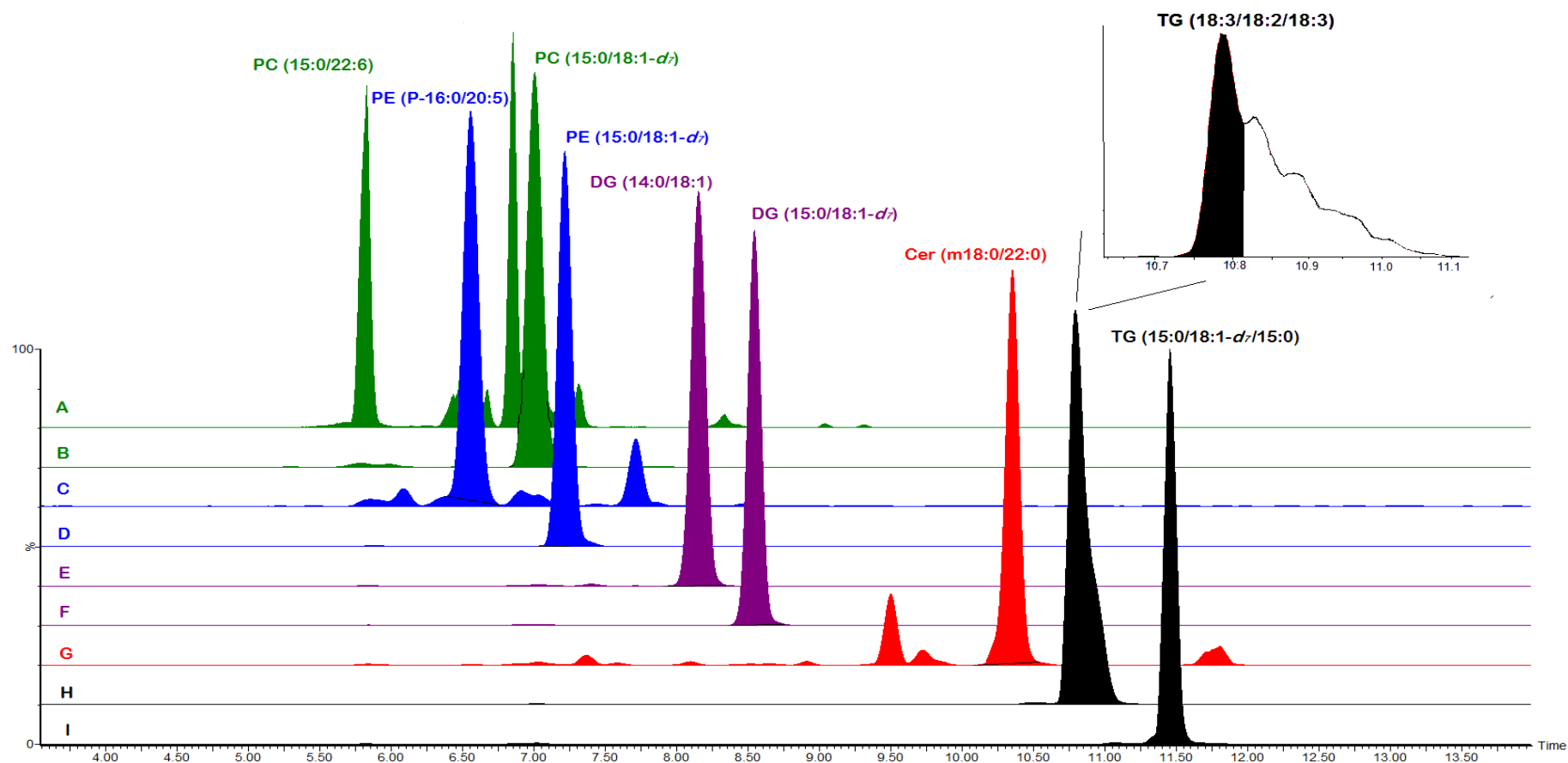
Figure 5.2: Chromatograms of a representative plasma sample. A: Phosphatidylcholine (PC) (15:0/22:6), B: PC (15:0/18:1- d 7 ), C: Phosphatidylethanolamine (PE) (P-16:0/20:5), D: PE (15:0/18:1- d 7 ), E: Diacylglycerol (DG) (14:0/18:1), F: DG (15:0/18:1- d 7 ), G: Ceramide (Cer) (m18:0/22:0) H: Triacylglycerol TG (18/18:2/18:3), I: TG (15:0/18:1- d 7 /15:0)
