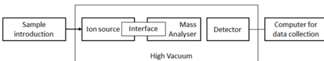
Figure 1.2: Schematic of the main components of a mass spectrometer.
