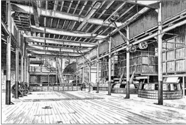
Figure 6.2. The brewhouse at Beamish and Crawford in the late-1880s. The cast-iron superstructure depicted supported the large, shallow coolers located in the loft above. This superstructure survives within the brewhouse today (Barnard 1889-91 vol. 2, 357).
