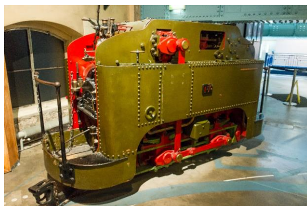
Plate 0.5. Locomotive no. 17, designed by Samuel Geoghan and constructed by Spence's Iron Works of Cork Street, Dublin city, in 1902.
