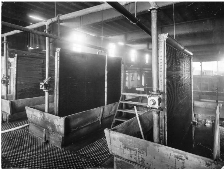
Plate 6.1. Morton's vertical refrigerators at Beamish and Crawford, late-19 th century (courtesy Diarmuid Ó Drisceoil).
