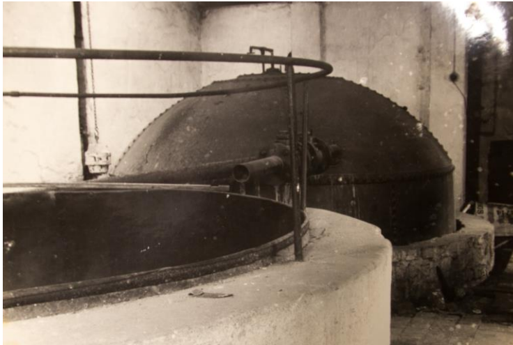
Plate 5.15. Two brewing coppers at the Mill Park Brewery, Enniscorthy in 1957. Note that the copper in the foreground was not lidded, while the one in the background is capped with a domed lid (courtesy D. Lett).
