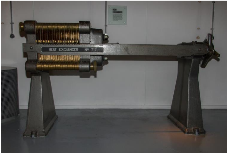
Plate 6.3. Horizontal plate heat exchanger by APV. Guinness Storehouse, Dublin.
