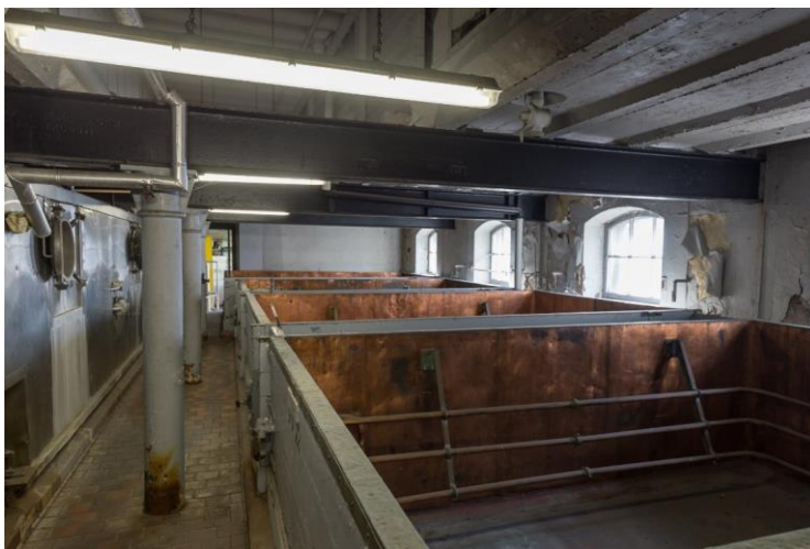
Plate 6.10. Lower floor of the fermenting block at the St. Mary's Brewery, Waterford. Note the cast-iron columns and beams that support the deeper fermenters that penetrate the ceiling from the upper level, visible in the top right.
