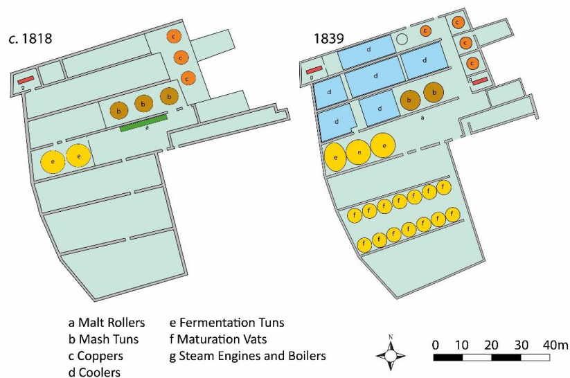
Figure 5.1. Upper-floor surveys of Beamish and Crawford, c. 1818 and 1839, including brewing plant. Source: CCCA/U18/MPD/13, 42. Approx. scale.
