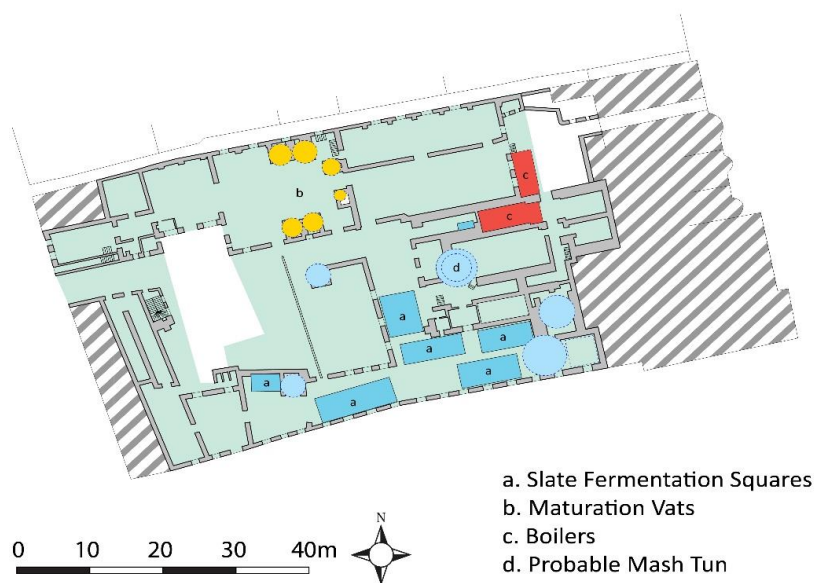
Figure 5.2. Survey of Lane's Southgate Brewery, Cork, dated 1880. The barrel-vaulted spaces, shown in plate 21, project eastwards from the middle of the eastern wall of the brewery. Source: CCCA/U18/MPD/350. Approx. scale
