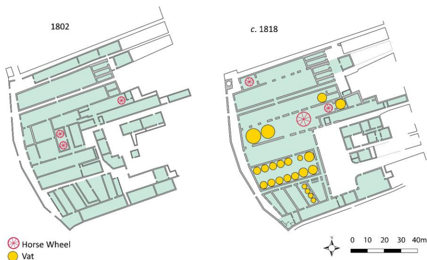
Figure 7.3. Horse wheels at Beamish and Crawford, 1802 and c. 1818. Source: CCA/U18/MPD/337 & 349. Approx. scale.
