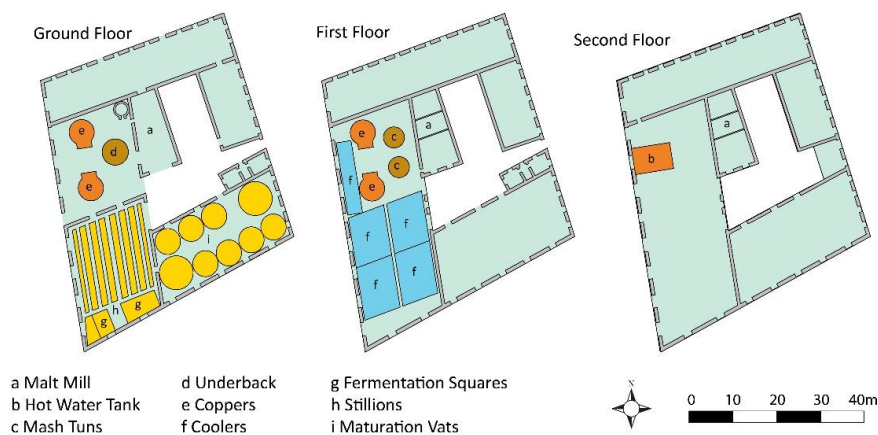
Figure 6.1. Undated surveys of all three floors of the River Lee Porter Brewery, Cork, including all brewing plant. Source: CCA/U18/MPD/6, 7, 10 & 13. Approx. scale.
