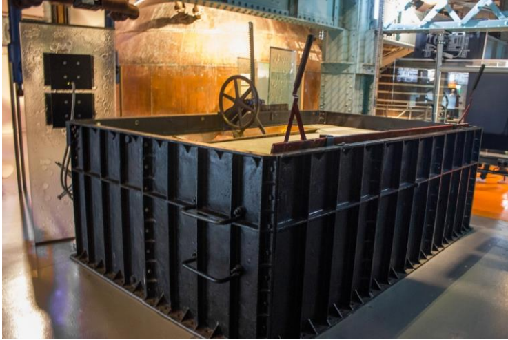
Plate 6.8. Cleansing square with manual yeast skimmer, Guinness Storehouse, Dublin. The cleansing square has been dramatically reduced in length, it was originally constructed to the same dimensions as the square in Plate 6.7.
