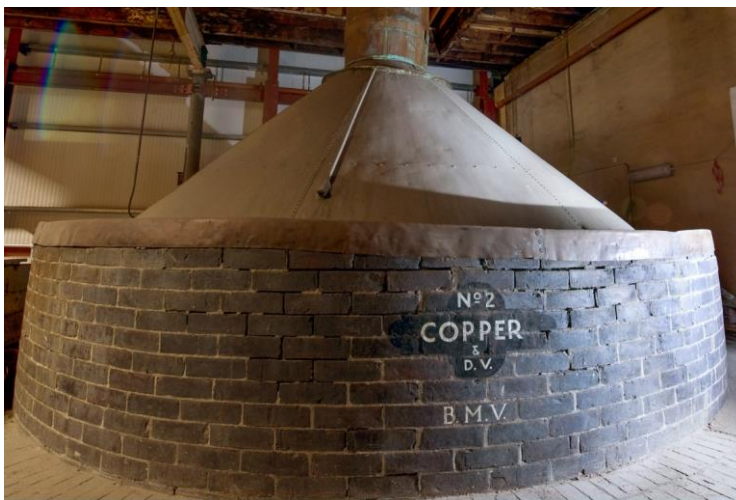
Plate 5.16. Brewing copper with conical cap at Beamish and Crawford, Cork. (courtesy Diarmuid Ó Drisceoil)
