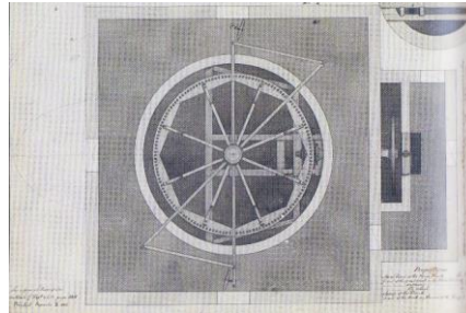
Figure 7.1. Plan of a complex horse engine designed by John Smeaton for the Weevil Brewery in Gosport, Hampshire. (Pearson 2014, 160 fig. 6.10).
