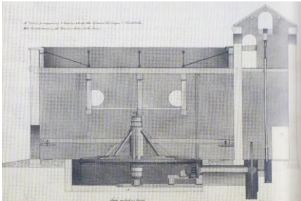
Figure 7.2. Section drawing of a complex horse engine designed by John Smeaton for the Weevil Brewery in Gosport, Hampshire (Pearson 2014, 160 fig. 6.9).
