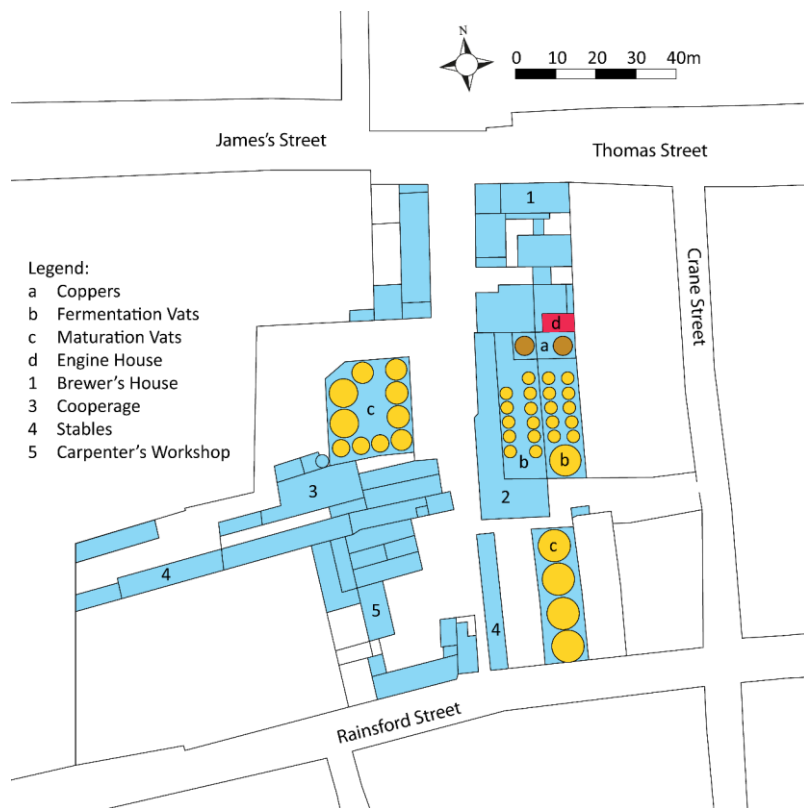
Figure 0.7. Guinness's Brewery in 1820. Approx. scale. Source: James's Gate Brewery, Historical Plans (Guinness Archives, Guinness Storehouse, Dublin).
