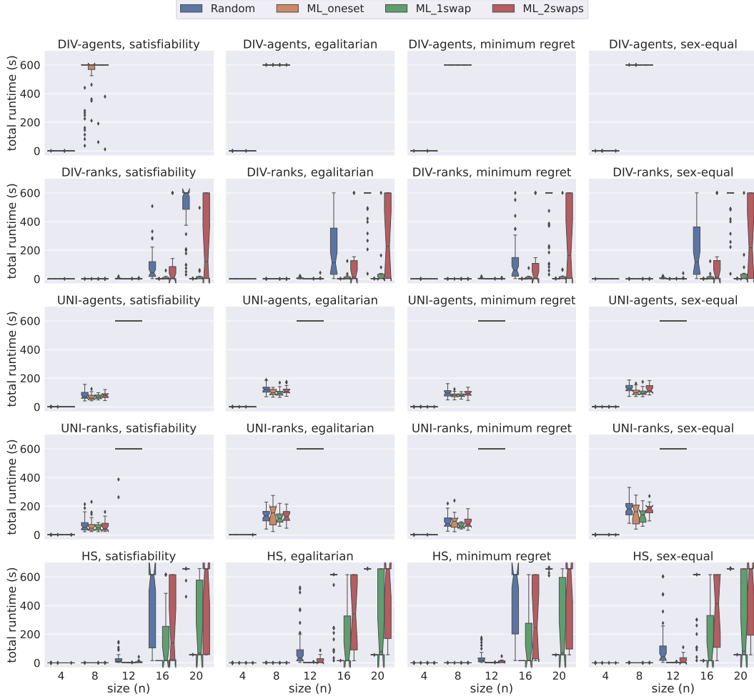
■ Figure 2 A comparison of total time spent by all models under strong stability using Gecode.
