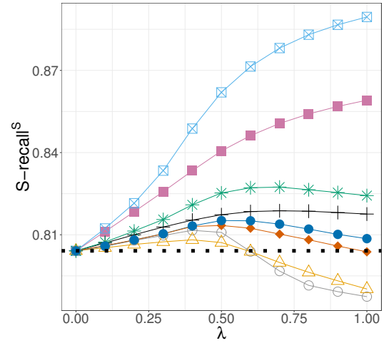
(b) \text{S-recall}^{\mathcal{S}} on ML1M
