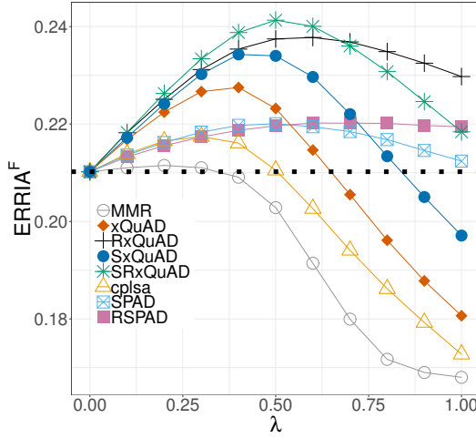
(a) \text{ERR-IA}^{\mathcal{F}} on ML1M
