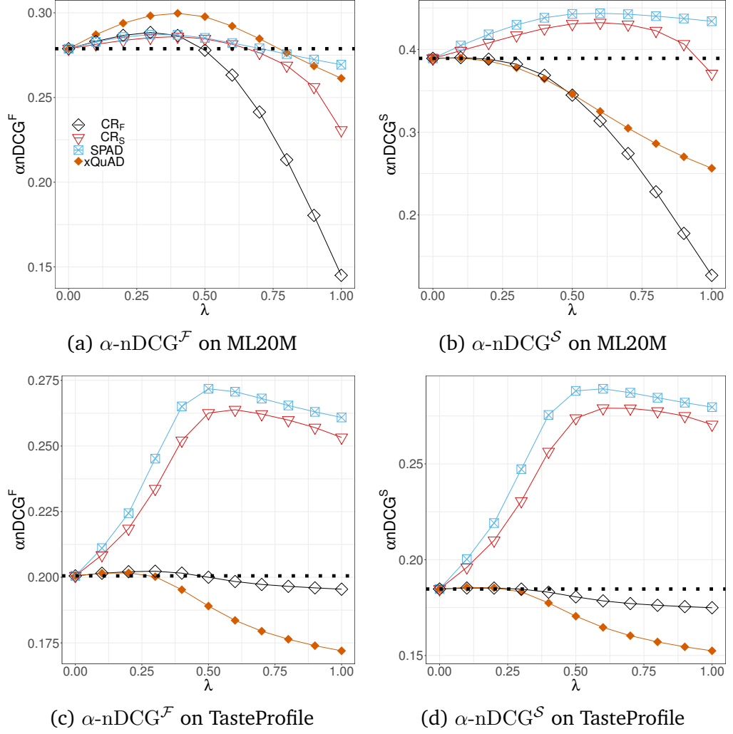
Figure 7.4: ML20M and TasteProfile datasets. \alpha\text{-nDCG} measured using features and subprofiles for different values of \lambda . Values for MF are shown by dotted lines.
