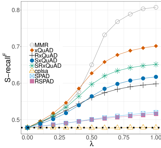
(a) \text{S-recall}^{\mathcal{F}} on ML1M
