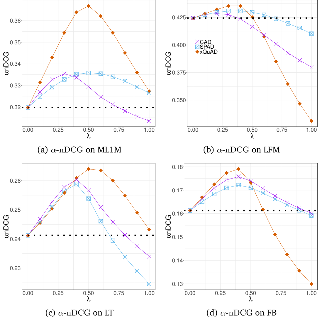
Figure 6.2: ML1M, LFM, LT and FB datasets. \alpha -nDCG values for varying \lambda using MF as baseline. Values for MF are shown by dotted lines.
