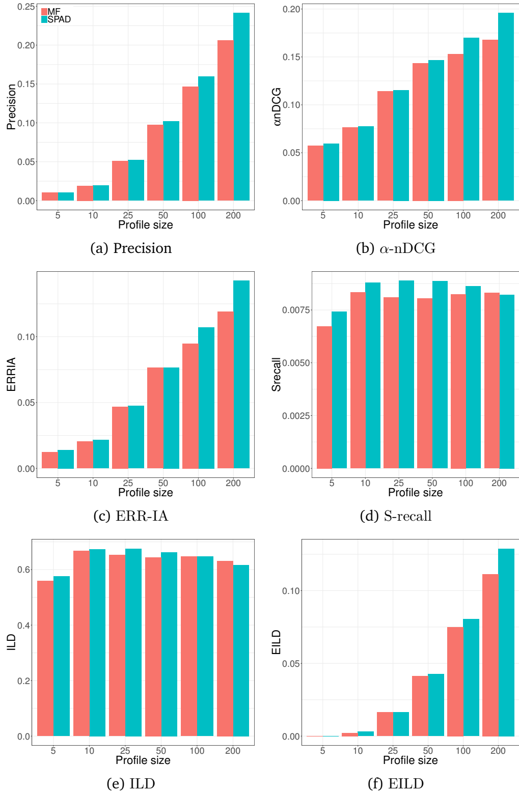
Figure 8.4: Profile length plots.
