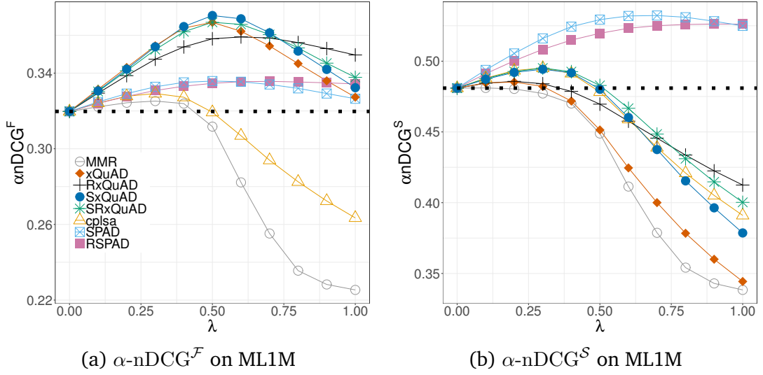
Figure 5.7: ML1M dataset. \alpha\text{-nDCG} measured using features and subprofiles for varying \lambda .
