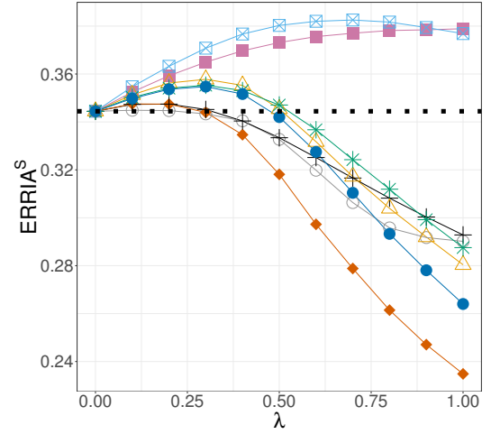
(b) \text{ERR-IA}^{\mathcal{S}} on ML1M
