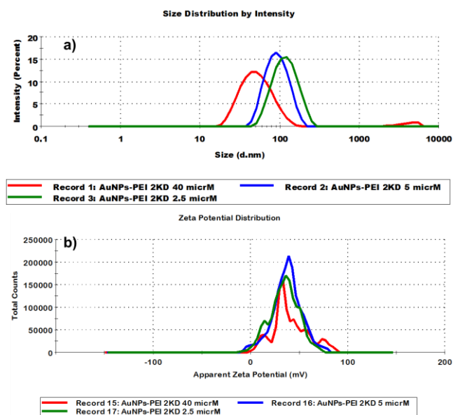
Figure 2: a) size distribution by intensity of AuNP-PEI 2KD from DLS measurements, showing that the size increase from 55 nm to 123 nm when the concentration of PEI 2KD was decrease from 40 \mu M to 2.5 \mu M. (b) zeta potential for the corresponding AuNPs-PEI 2KD showing that all AuNPs-PEI samples were positively charged with a \zeta -potential in the range of 37 \pm 3 mV.
