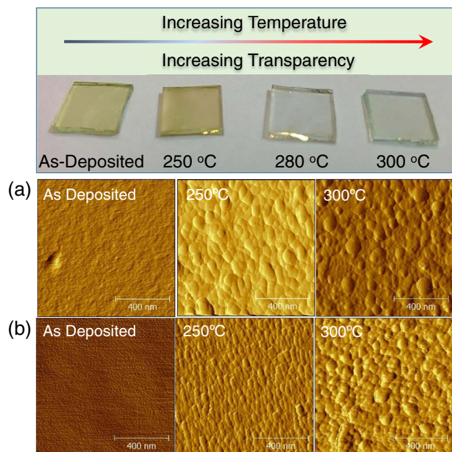
Figure 1. (Top) Optical images of as-deposited \text{V}_2\text{O}_5 thin films on glass, and the optical transparency development on conversion to a quaternary V-O-Na-Si TTF. (Bottom) AFM surface morphology images acquired for (a) \text{V}_2\text{O}_5\text{-H}_2\text{O} and (b) \text{V}_2\text{O}_5\text{-PEG} thin films at different temperatures.
