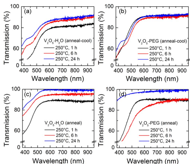
Figure 6. UV-Vis optical transmission spectra for (a,c) \text{V}_2\text{O}_5\text{-H}_2\text{O} and (b,d) \text{V}_2\text{O}_5\text{-PEG} thin films annealed at 250^\circ\text{C} in order to convert to V-O-Na-Si TTF as a function of annealing time. Dip-coated thin films were treated with an anneal-cool (a,b) and a full anneal (c,d) protocol respectively (see Experimental).
