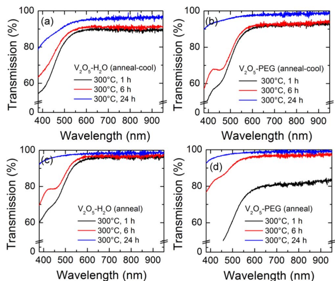
Figure 7. UV-Vis optical transmission spectra for (a, c) \text{V}_2\text{O}_5\text{-H}_2\text{O} and (b, d) \text{V}_2\text{O}_5\text{-PEG} thin films annealed at 300^\circ\text{C} in order to convert to V-O-Na-Si TTF as a function of annealing time. Dip-coated thin films were treated with an anneal-cool and a full anneal protocol respectively (see Experimental).
