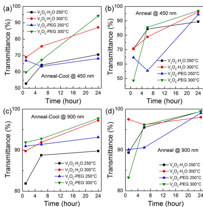
Figure 8. Transparency at 450 nm (a,b) and 900 nm (c,d) for both types of thin films annealed to the V-O-Na-Si TTF at 250^\circ\text{C} and 300^\circ\text{C} for 24 h under anneal-cool (left) and anneal (right) conditions.
