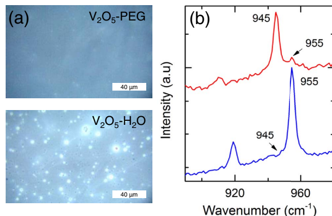
Figure 5. (a) Optical images and (b) corresponding Raman spectra of the resulting annealed films from V 2 O 5 -H 2 O and V 2 O 5 -PEG precursors.
