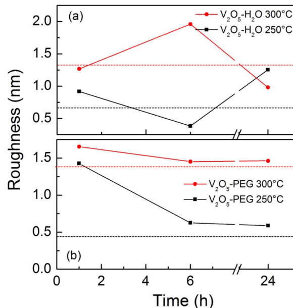
Figure 3. Variation of measured rms roughness as a function of annealing time for (a) \text{V}_2\text{O}_5\text{-H}_2\text{O} and (b) \text{V}_2\text{O}_5\text{-PEG} thin films at 250^\circ\text{C} and 300^\circ\text{C} . The dashed lines indicated the as-deposited rms roughness of the films prior to any annealing treatment.
