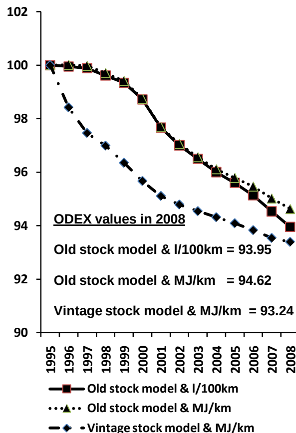
Figure 4 All calculated versions of the Irish private car ODEX
