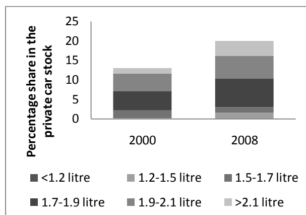
Figure 10 Change in diesel stock composition by engine size
