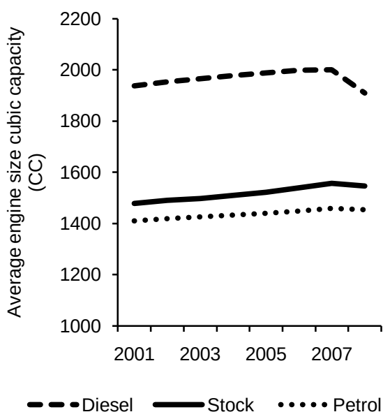
Figure 8 Average engine size of the separate and combined petrol and diesel stock
