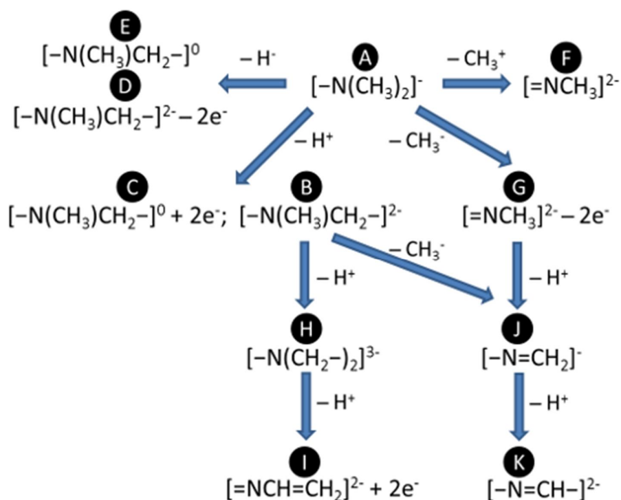
Figure 5-4 Reaction scheme for decomposition of dimethylamido ligand [-\text{N}(\text{CH}_3)_2]^- on metal oxide surfaces (species A-K). Notation: ' -\text{H}^{+/-} ' means dissociation of proton/hydride from ligand to the surface; ' -\text{Me}^{+/-} ' means dissociation of methylum/methanide group from ligand to the surface; ' +2e^- ' means oxidation of ligand by surface (reduction of surface by ligand); ' -2e^- ' means reduction of ligand by surface (oxidation of surface by ligand).
