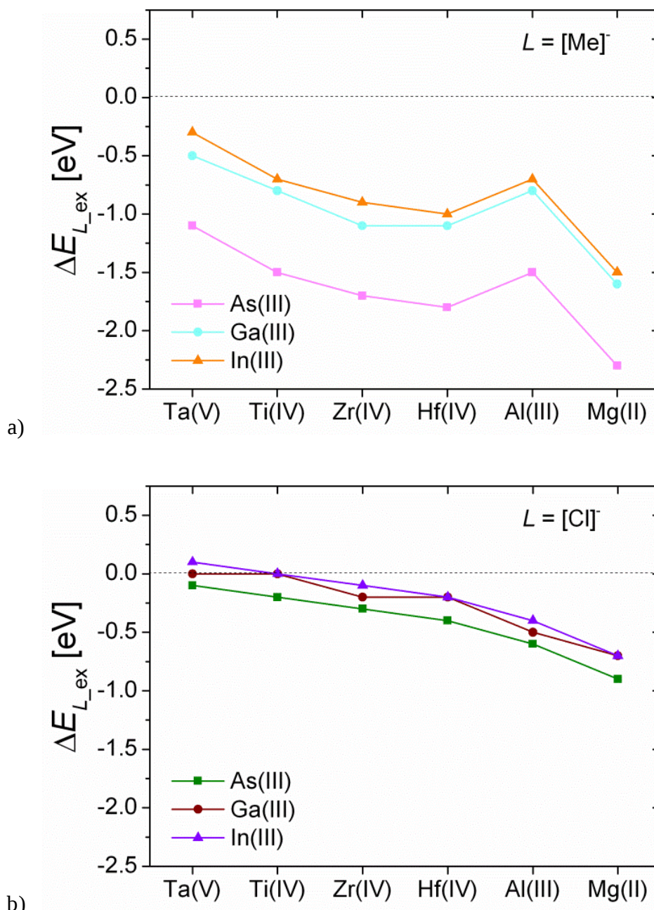
Figure 5-6 Computed energetics for ligand exchange between precursor metal center and bulk III-V oxide: \text{As}_2\text{O}_3 , \text{Ga}_2\text{O}_3 and \text{In}_2\text{O}_3 according to: 1/n \text{ML}_n(\text{g}) + 1/6 (\text{As/Ga/In})_2\text{O}_3(\text{bulk}) \rightarrow 1/2n \text{M}_2\text{O}_n(\text{bulk}) + 1/3 (\text{As/Ga/In})\text{L}_3(\text{g}) for M = \text{Mg(II)} , \text{Al(III)} , \text{Ti(IV)} , \text{Zr(IV)} , \text{Hf(IV)} , \text{Ta(V)} and L = \text{a) } [\text{Me}]^- \text{ b) } [\text{Cl}]^- . Lines are to guide the eye.
