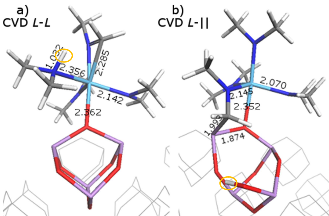
Figure 6-6 Surface models showing products of H elimination mechanism leading to the decomposition of molecularly adsorbed \text{Hf}(\text{NMe}_2)_4 precursor: a) H (highlighted by the orange circle) eliminated from one ligand to another; b) H (highlighted by the orange circle) eliminated from ligand to the \text{As}_2\text{O}_3 surface. Stick representation: purple As, red O, white H, gray C, green Cl, blue N, light blue Hf. Selected bond lengths are given in Å. Thin lines show adjacent substrate atoms.
