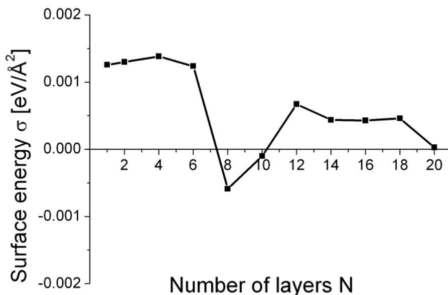
Figure 2-1. Surface formation energies ( \sigma ) for As 2 O 3 (010) as a function of the slab thickness (number of layers N , where a layer is defined as a two molecular units of As 4 O 6 ).
