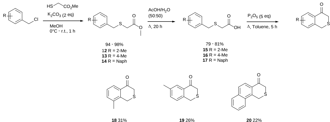
Scheme 5: Cyclisation to the sulfides 18 - 20 .
