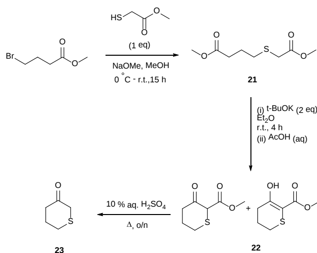
Scheme 6 : Generation of the monocyclic sulfide 23 through cyclisation of the diester 21 followed by hydrolysis and decarboxylation of keto enol mixture 22
