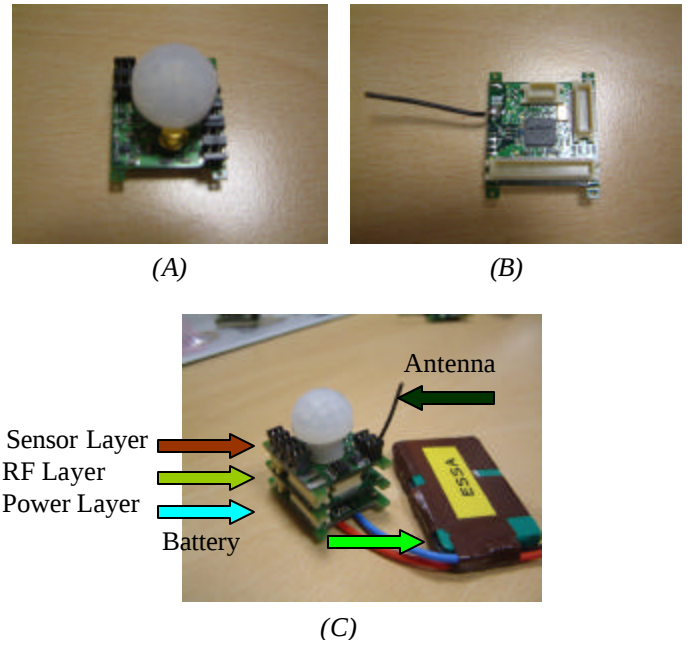
Figure 3: Photos of the (a) Developed sensor layer, (b) Zigbee and processor layer, and (c) The complete 25mm stackable mote
