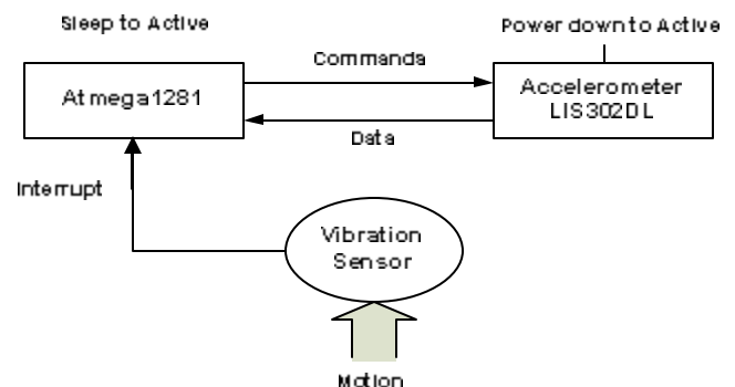
Figure 6: Functional block diagram of e motion sensor design
