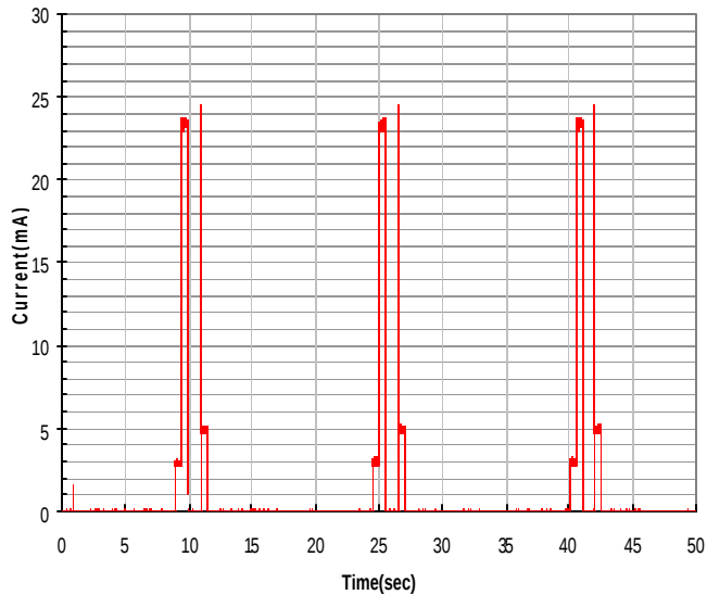
Figure 11: Node current consumption behavior at fixed duty cycle
