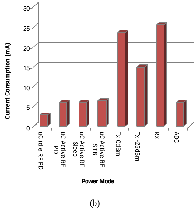
Figure 10: Current consumption at different power modes of both the microcontroller (uC) and transceiver (RF) units. PD and STB refer to Power Down and Standby modes
