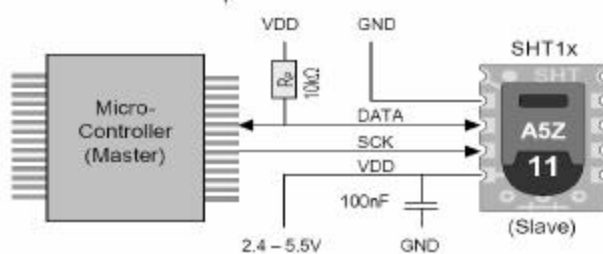
Figure 4: Typical application circuit of the SHT11
