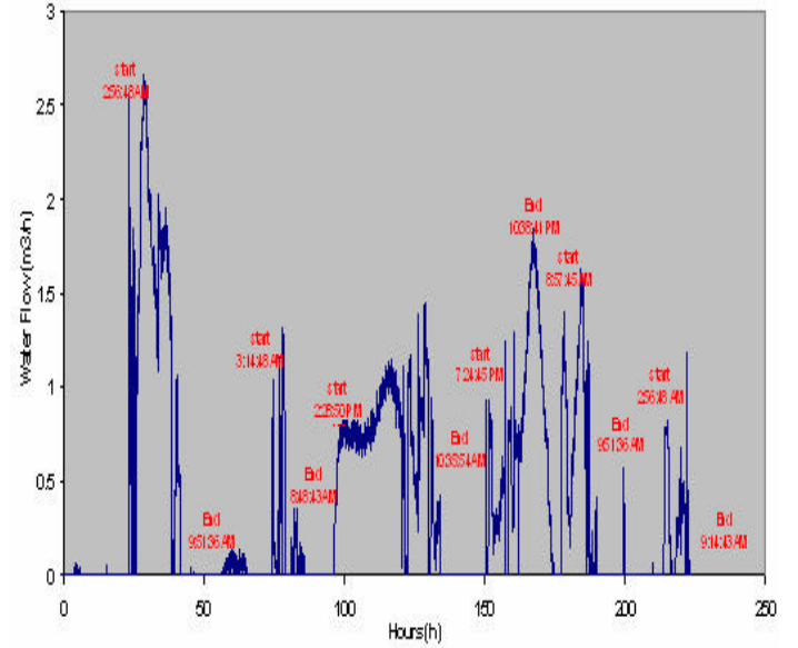
Figure 7: Water flow rate measurements
