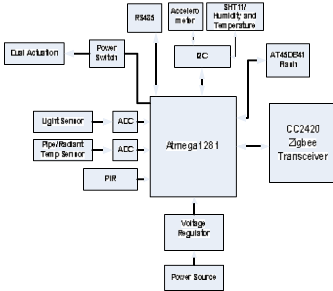
Figure 2: block diagram of the mote functional units
