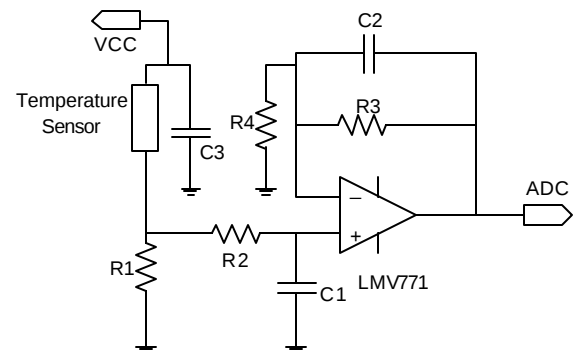
Figure 8: Schematic of the water pipe temperature sensor interface circuitry
