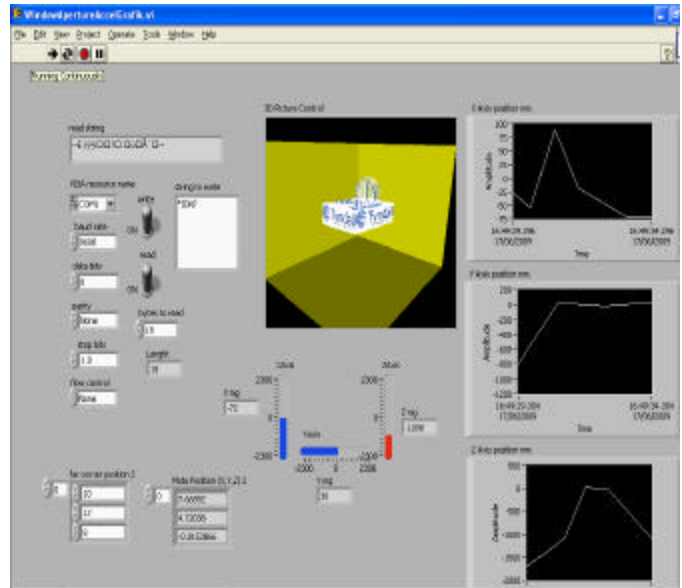
Figure 5: 3-Axis accelerometer LABVIEW GUI
