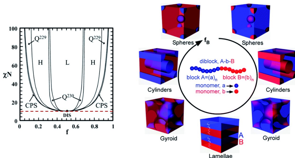
Figure 1-5. Phase diagram of a diblock copolymer by self-consistent field theory with CPS: close packed spheres, H: hexagonally packed cylinder, L: lamellae, Q 229 : body centred spheres, Q 230 : double-gyroid and DIS: disordered. Schematic illustration of microstructures with increased f_B , volume fraction of block B. Adapted from Hu et al. (Soft Matter, 2014) 25
