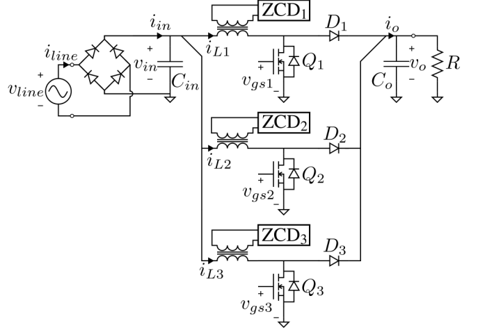
Fig. 1. Three-channel boost converter power stage.
