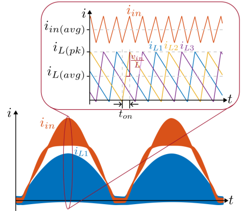
Fig. 2. Typical waveforms of the input current i_{in} and the inductor currents i_{L1}, i_{L2} and i_{L3} over a full-line cycle of the line voltage v_{line} .
