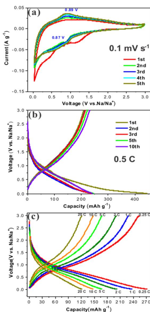
Fig. 6. (a) CV curves at a scan rate of 0.1 mV s -1 , (b) charge-discharge profiles of the first, second, third, fifth and tenth cycle at a current density of 0.5 C, (c) charge-discharge profiles at different rate for the S-TiO 2 /CS composites anode.
