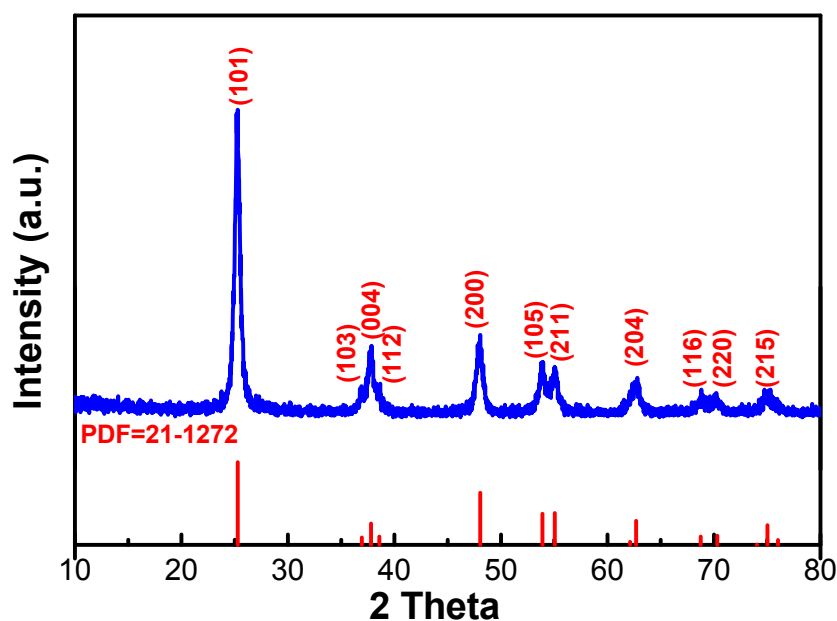
Fig.1. XRD images of the as-prepared S- \text{TiO}_2 /CS composites.
