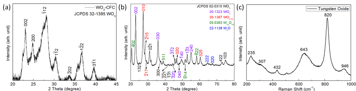
Figure 1. XRD of (a) WO 3 /CFC and (b) WO nanoparticles, (c) Raman spectra of WO nanoparticles.
