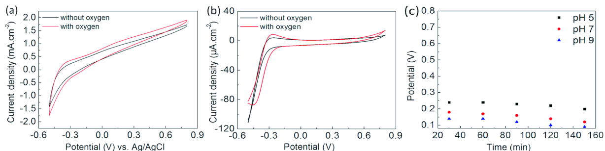
Figure 6. CVs at presence/absence of oxygen of (a) WO 3 /CFC and (b) WO/GCE, (c) Drift of WO/GCE electrode.
