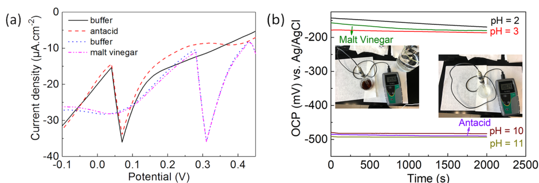
Figure 7. (a) SWV obtained in buffer (pH = 4 and 9) and “real” unbuffered samples for malt vinegar and antacid using WO/GCE; (b) OCP obtained in buffer (pH = 2, 3, 10, 11) and “real” unbuffered samples for malt vinegar and antacid using WO 3 /CFC.
