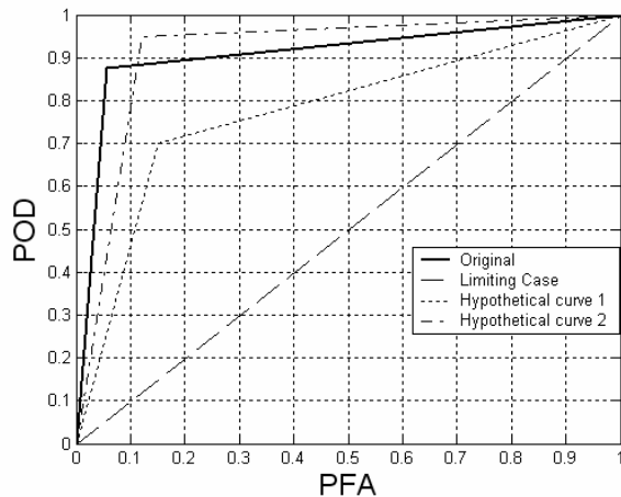
Figure 5 ROC Curves for the Current Problem.
