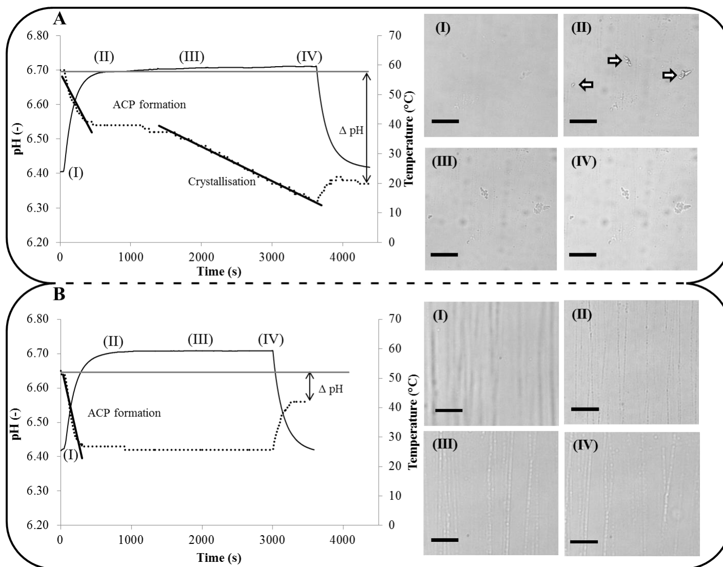
Fig. 6. Changes in pH during incubation of (A) simulated milk ultrafiltrate (SMUF) and (B) \beta -casein concentrate (BCC) in SMUF at \sim 60^\circ C . Images taken by a light microscope during an equivalent heating cycle at corresponding stages (I-IV) are shown. Temperature is shown as a solid curve and pH as a broken curve. A grey horizontal line is shown extending from starting pH to guide the eye for pH hysteresis ( \Delta pH ) calculation. Linear fits are fitted to pH curves to estimate the rate of amorphous calcium phosphate (ACP) formation and crystallisation. Scale bars represent a size of 50 \mu m . Examples of crystals are indicated by an arrow. Data are from a single analysis but are representative of replicate profiles.
