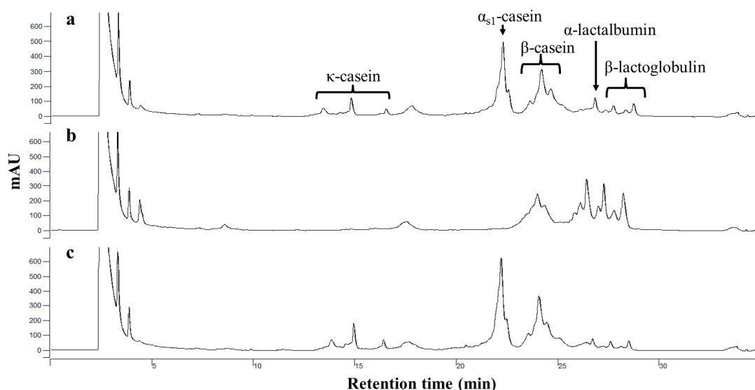
Fig. 4. Chromatograms from reversed-phase high-performance liquid chromatography for (a) feed and (b) permeate and (c) retentate streams from membrane separation of skim milk at 3.4 \pm 0.3^{\circ}\text{C} using a 0.1\ \mu\text{m} pore-size polyvinylidene-difluoride membrane, showing the identification of peaks associated with proteins of interest.
