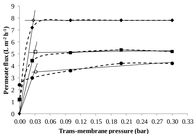
Fig. 1. Permeate flux as a function of trans-membrane pressure during the filtration of reconstituted skim milk at 3.4 \pm 0.3^{\circ}\text{C} in full recirculation mode with a 0.1 \mu\text{m} polyvinylidene-difluoride (■), 0.45 \mu\text{m} polyvinylidene-difluoride (●) or 1000 kDa polyethersulfone (◆) membrane. Critical flux values are indicated by open symbols. Results are from a single trial for each membrane.
