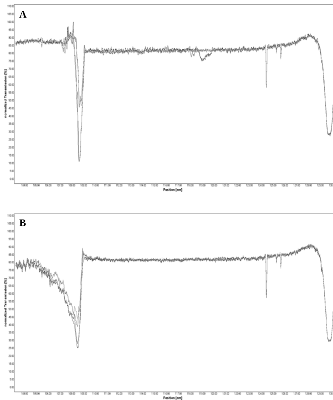
Fig. S3. Profiles showing change in transmission of NIR light through sample suspensions as a function of time and position in the sample cell during centrifugation at 36 \times g for 10 min followed by 168 \times g for 10 min of a milk protein concentrate (MPC) powder (MPC90) rehydrated in 80 mM trisodium citrate for 90 min at 25°C (A) or 50°C (B).
