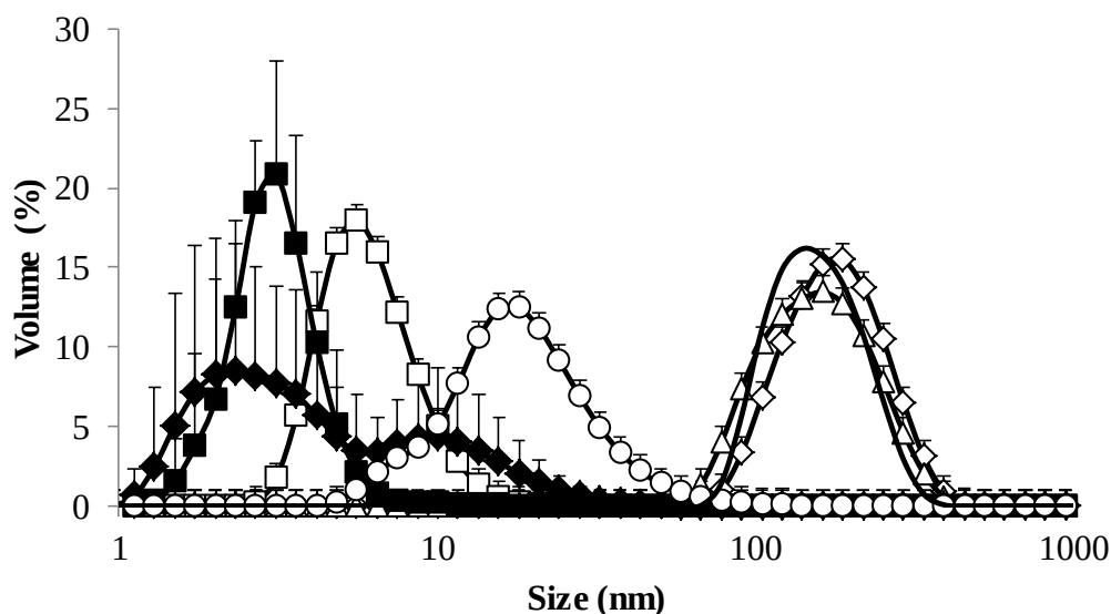
Fig. 2. Particle size distributions of \beta -casein concentrate (BCC) solutions prepared in simulated milk ultrafiltrate (SMUF), and incubated at 4, 20, 26 and 37°C for 30 min analysis at 4°C (□), 20°C (○), 25°C (◇), 35°C (Δ) or 63°C (—), respectively. Solutions were diluted (1:10) and filtered (0.22 \mu m) prior to analysis. Results for BCC/water solutions at 4°C (■) and 25°C (◆) are included for comparison. Data are the means ( \pm standard deviations) of solutions subjected to two separate incubation experiments, prepared and analysed for size in duplicate. The 63°C data was the result of a single analysis on pooled filtrate due to low sample volume.
