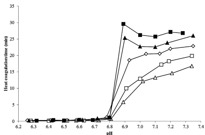
Fig. 3. pH-heat coagulation time (pH-HCT) profiles at 140 °C for a 3.5% (w/w) protein suspension of milk protein concentrate (MPC)80, with urea added at levels of 0 (△), 100 (□), 200 (◇), 300 (▲) or 400 (■) mg L -1 . Values are the means of data from duplicate analysis.
