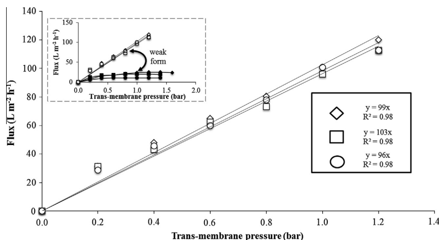
Fig. 2. Main: Permeate flux ( J ) as a function of trans-membrane pressure ( TMP ) during ultrafiltration of deionised water at a cross flow velocity ( V ) of 0.09 ( \circ ), 0.23 ( \square ) or 0.36 ( \diamond ) \text{m s}^{-1} , and a temperature of 15 °C. The inset figure shows a comparison of the TMP – J relationship for deionised water and reconstituted infant milk formula powder (IMF), indicating weak-form critical flux; data for IMF at V values of 0.09 ( \bullet ), 0.23 ( \blacksquare ), and 0.36 ( \blacklozenge ) \text{m s}^{-1} are presented.
