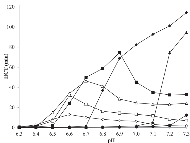
Fig. 1. pH-heat coagulation time (pH–HCT) profiles at 120 °C for MPC35 (◇), MPC50 (□), MPC60 (△), MPC70 (■), MPC80 (◆) and MPC90 (●) reconstituted to 8.5% (w/w) protein. Values are the means of duplicate data from three independent trials.
