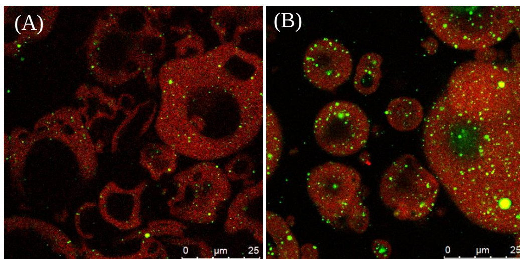
Fig. 1. Representative confocal laser scanning microscopy images of micellar casein concentrate (MCC) powders manufactured by microfiltration at <10°C (A) or 50°C (B), followed by evaporation and spray drying. Green indicates fat and red indicates protein, while black regions within particles are air vacuoles.
