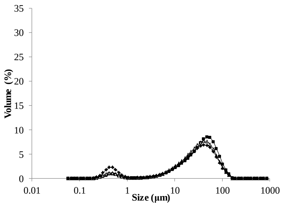
Fig. S2. Particle size distribution (PSD) data for milk protein concentrate (MPC)90 after 24 h rehydration in deionised water with (■) or without (Δ) octanol or in 80 mM KCl (◆) at 25°C. The PSD of MPC90 rehydrated in water was measured with and without octanol in the dispersing line of the Mastersizer to assess the potential influence of entrained gas bubbles on light scattering. Note: ranges of values shown in axes match those of PSD profiles in main manuscript.
