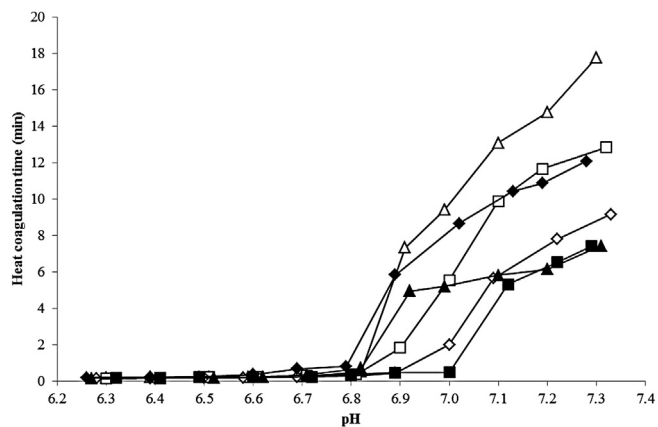
Fig. 4. pH-heat coagulation time (pH-HCT) profiles at 140 °C for a 3.5% (w/w) protein suspension of milk protein concentrate (MPC)80 with added lactose concentrations (% w/w) of 0.00 (△), 0.72 (□), 1.72 (◇), 2.72 (■) or 4.62 (▲) or with 4.62% (w/w) added maltodextrin (◆). Values are the means of data from duplicate analysis.
