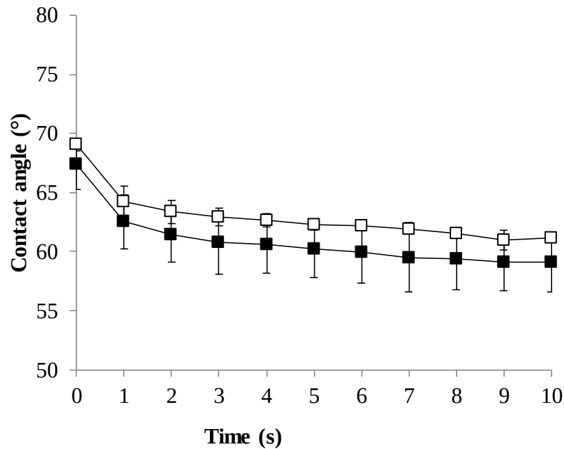
Fig. 2. Contact angle values over time for a droplet of deionised water deposited on compressed discs of micellar casein concentrate (MCC) powder manufactured by microfiltration at <10°C (□) or 50°C (■) followed by evaporation and spray drying. Data points are the mean \pm standard deviation of replicate experiments ( n = 3 ).
