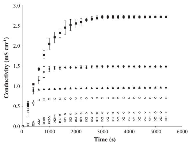
Fig. 3. Conductivity of suspension during the rehydration of milk protein concentrate (MPC) 35 (■), MPC50 (◆), MPC60 (▲), MPC70 (○), MPC85 (□) and MPC90 (△) in deionised water measured dynamically over 90 min at 25 °C. Values are presented as mean \pm standard deviation of data from three independent trials. Every 100th profile is shown.
