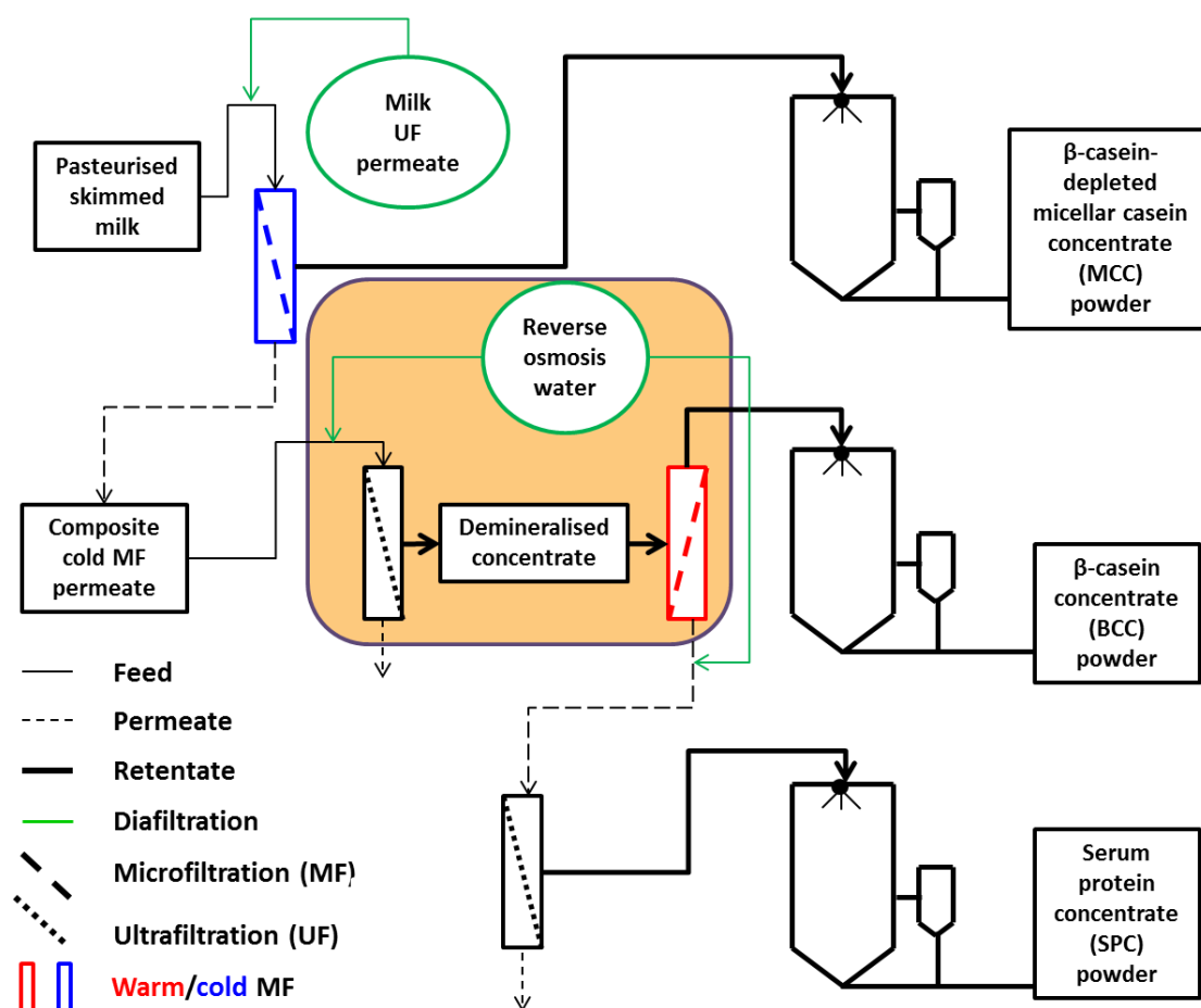
Fig. 3. Process flow diagram for manufacture of \beta -casein concentrate using ‘cold-then-warm’ microfiltration. The orange area indicates where the process was optimised through fractionation of \beta -casein from serum proteins using warm MF (without concentration) at a controlled ionic strength of \sim 32 mM.
