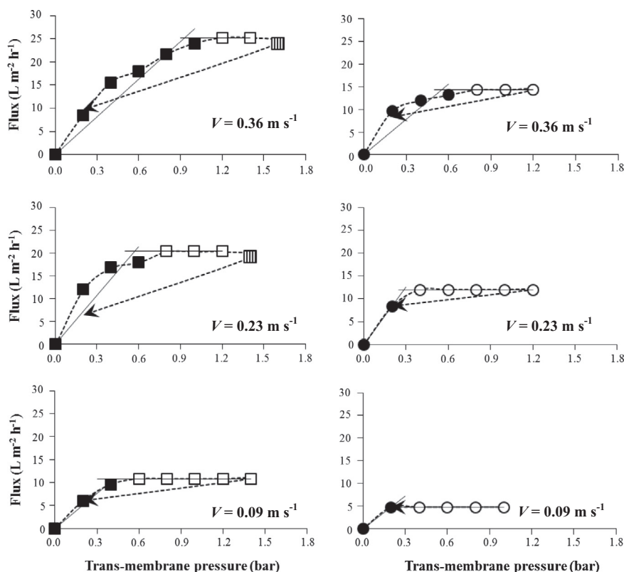
Fig. 1. Permeate flux as a function of trans-membrane pressure (TMP) and cross-flow velocity ( V ) at 15 °C for reconstituted skim milk powder (SMP; circles) and reconstituted infant milk formula powder (IMF; squares). Regions where flux ( J ) is pressure-dependant and pressure-independent are denoted by closed and open symbols, respectively; linear fits were applied to both of these regions, and critical flux was determined as being the last point in the pressure-dependant region. The broken line is a plot through all the data points, where the arrow indicates whether hysteresis of J occurred due to membrane fouling when TMP was returned to 0.2 bar. Symbols with vertical lines inset indicate that limiting flux has been exceeded.
