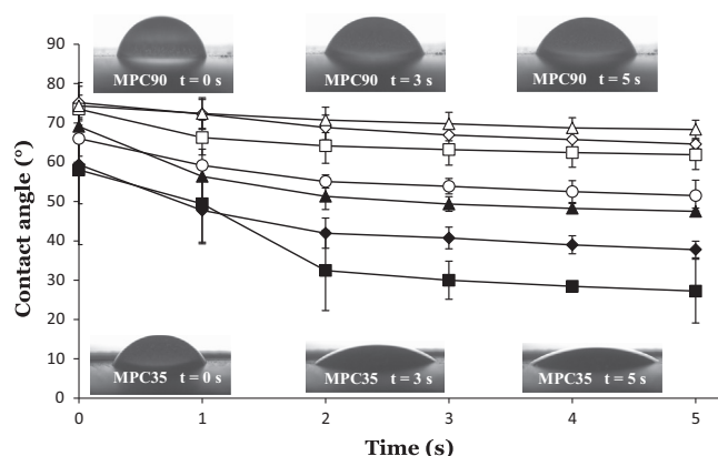
Fig. 2. Contact angle developed between a deposited drop of deionised water and the surface of a compressed disc of milk protein concentrate (MPC) 35 (■), MPC50 (◆), MPC60 (▲), MPC70 (○), MPC85 (□) and MPC90 (△) powder over time. Values are presented as mean \pm standard deviation of data from three independent trials. Representative images of droplets on MPC35 and MPC90 after 0, 3 or 5 s of analysis are shown in inset.
