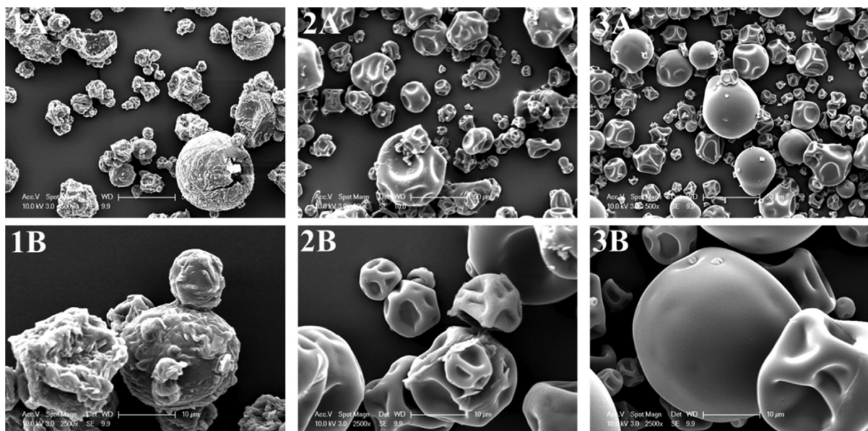
Fig. 8. Cryo-SEM micrographs of dry (1) MPC35, (2) MPC70 and (3) MPC90 at magnifications of (A) 500× and (B) 2500×, with scale bars of 50 and 10 μm, respectively, for the magnifications.
