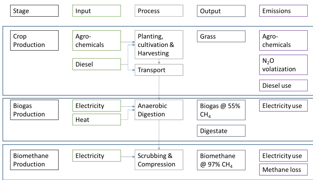
Figure 3-1 Grass biomethane system - Adapted from Smyth et al. 2009
