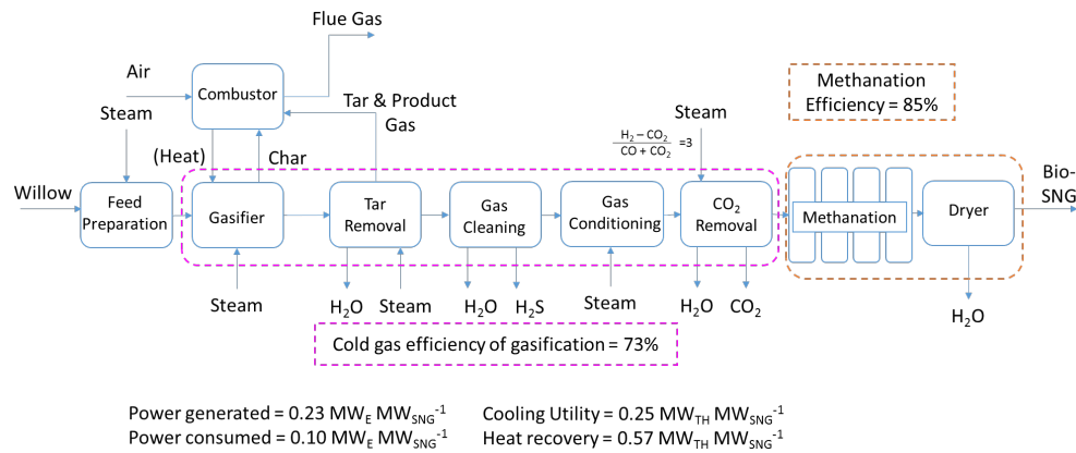
Figure 4-1 Biomass to Bio-SNG process adapted from Singlitico et al., 2019 [29]
