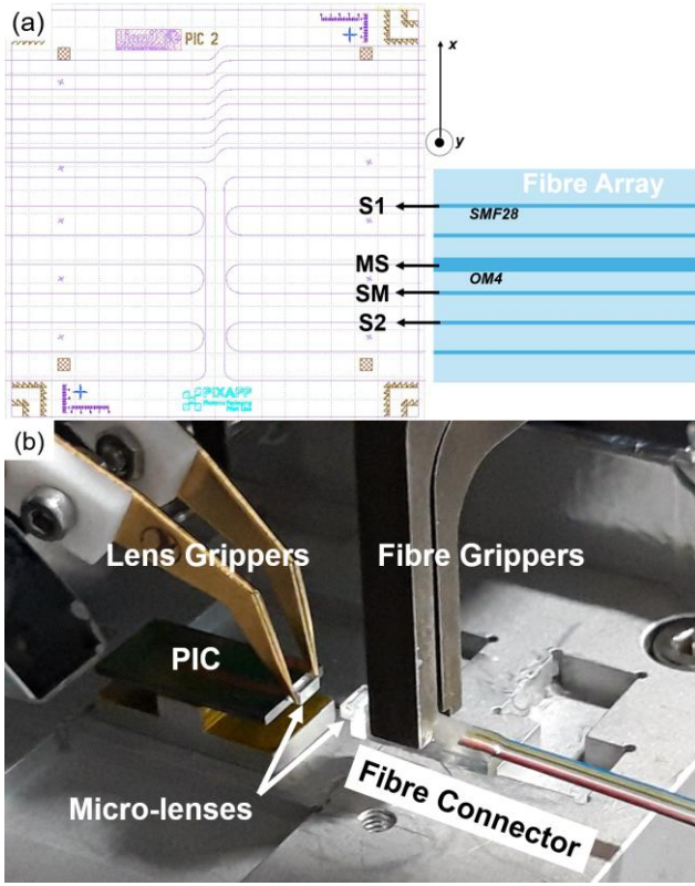
Fig. 1 (a) Schematic of the reference PIC and the fiber array design. (b) Photograph of the lens alignment procedure.
