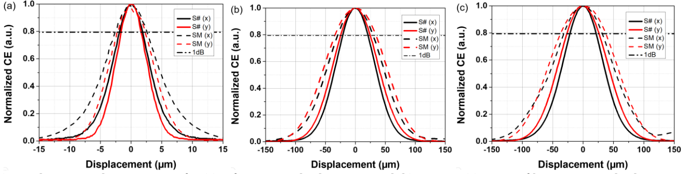
Fig. 2 Alignment tolerance curves for (a) reference FA displacement, and (b) Lens A, (c) Lens B fiber connector displacements. Black curves correspond to x-axis, red – to y-axis. Solid lines are recorded on one of the S-channels, while dashed line represents the SM channel. Horizontal line shows 1dB tolerance cut-off level.
