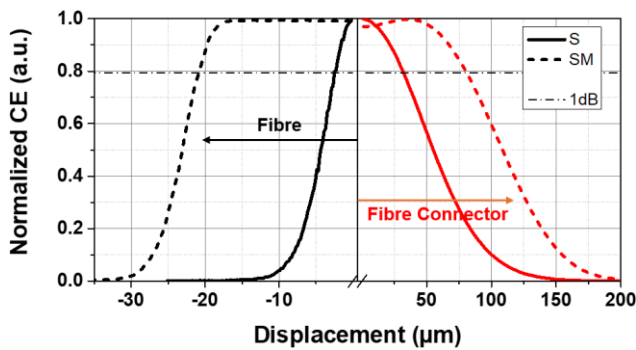
Fig. 3 Displacement tolerance curves in fiber-to-fiber (black, left-hand side) and lensed-fiber to lensed-fiber (red, right-hand side) experiments. Solid line represents SMF to SMF injection and the dashed – SMF to MMF. The horizontal line shows 1dB tolerance cut-off.
