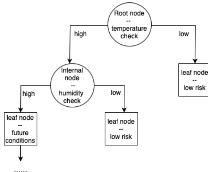
Figure 3.4: Decision Tree
