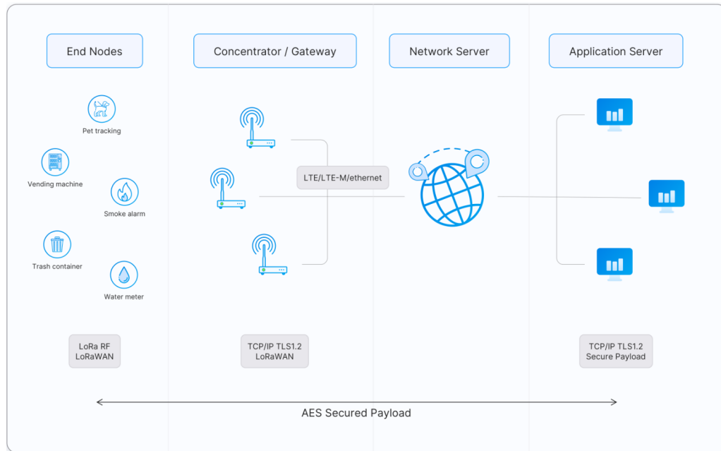
Figure 3.2: LoRaWAN Network Architecture [95]
