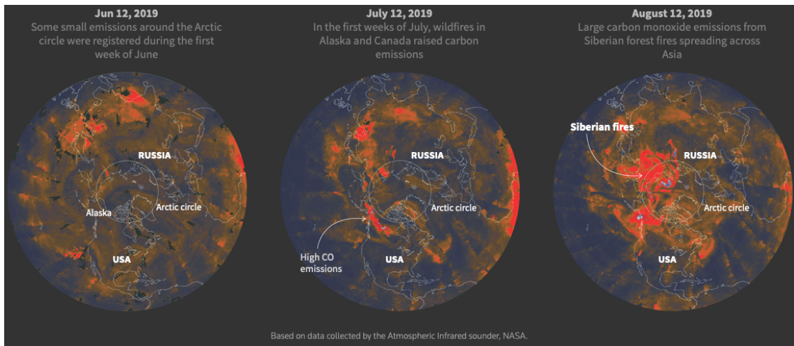
Figure 1.6: Wildfires release vast reserves of carbon stored in trees and soil, based on data collected by the Atmospheric Infrared sounder, NASA [20]
