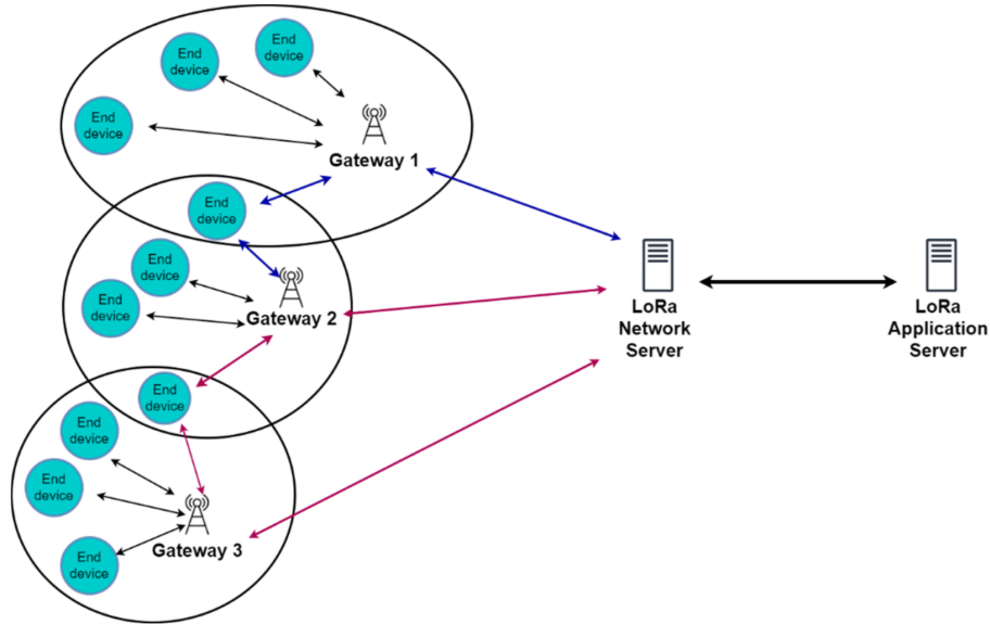
Figure 2.1: Star-of-stars LoRaWAN topology [37]
