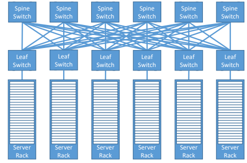
Fig. 8: Logical Diagram of Original Spine-Leaf DCN
