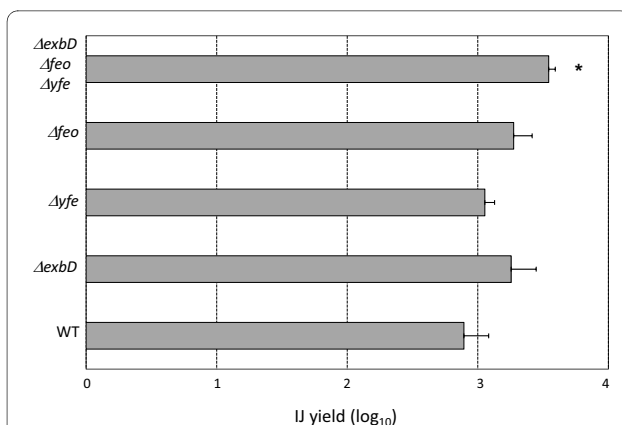
Figure 5 The IJ yield after growth on P. luminescens . The different bacterial strains were inoculated onto lipid agar plates, incubated for 3-4 days at 30°C and 40 surface-sterilised H. bacteriophora IJs were added to the biomass. The plates were incubated for 21 days at 25°C and the IJ yields were determined (i.e. total number of IJs/50). For each experiment 5 plates were analyzed for each strain and the experiment was repeated 3 times. Therefore the data shown is the mean \pm standard deviation of n = 15 plates for each strain. Statistical significance was determined using a T-test and IJ yields significantly different ( P < 0.01 ) to those obtained using TT01 are indicated with an asterisk.
