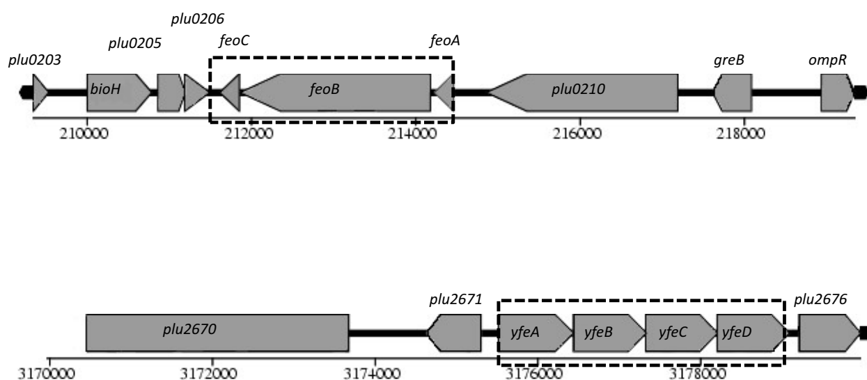
Figure 2 The feoABC and yfeABCD loci in P. luminescens TT01. The genetic loci predicted to encode the FeoABC permease and YfeABCD transporter (taken from Colibase at http://xbase.bham.ac.uk/colibase ). The genes deleted in this study are highlighted with the dashed line boxes.
