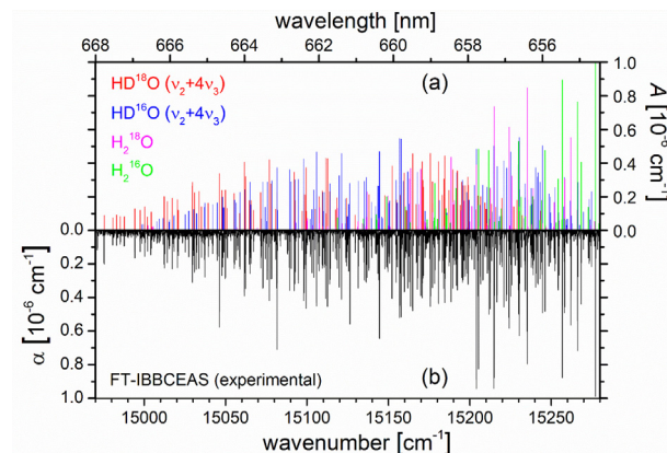
Fig. 2. (a) Upper panel: Stick spectrum of the ro-vibrational line absorption coefficient, A = S_{\text{Tomsk}} [\text{cm}/\text{molecule}] / \text{FWHM} [\text{cm}^{-1}] (natural relative abundance) \times n [molecule \text{cm}^{-3} ], of the \nu_2+4\nu_3 bands of \text{HD}^{16}\text{O} (blue trace) and \text{HD}^{18}\text{O} (red trace) from the Tomsk database [35] between 14970 and 15280 \text{cm}^{-1} , that best matches the measured spectrum. The magenta and green traces show the corresponding stick spectra of \text{H}_2^{18}\text{O} and \text{H}_2^{16}\text{O} in that region. Values of (natural relative abundance) \times n : \text{HD}^{16}\text{O} ( 3.10693 \times 10^{-4} ) \times 6.7 \times 10^{16} \text{ cm}^{-3} , \text{HD}^{18}\text{O} ( 6.23003 \times 10^{-7} ) \times 5.5 \times 10^{16} \text{ cm}^{-3} , \text{H}_2^{16}\text{O} ( 0.997317 ) \times 3.8 \times 10^{16} \text{ cm}^{-3} , \text{H}_2^{18}\text{O} ( 1.99983 \times 10^{-3} ) \times 3.1 \times 10^{16} \text{ cm}^{-3} ; FWHM = 0.1 \text{cm}^{-1} . The wavenumber scale of line intensities of \text{HD}^{16}\text{O} was shifted by -0.361 \text{ cm}^{-1} and the wavenumber scale of \text{H}_2^{18}\text{O} was shifted by -0.305 \text{ cm}^{-1} . (b) Lower panel: main measured spectrum (absorption coefficient \alpha , black trace) using FT-IBBCEAS. (For interpretation of the references to colour in this figure legend, the reader is referred to the web version of this article.)
