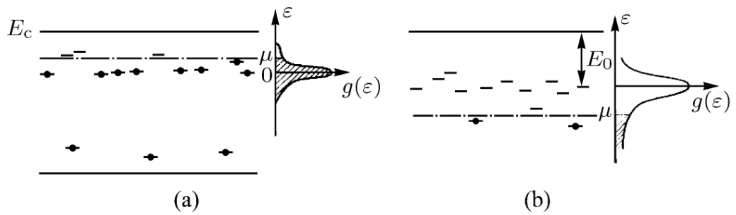
Figure 3.10: Impurity bands
