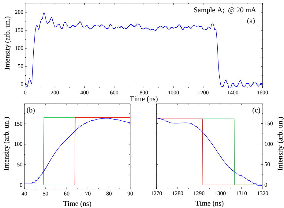
Figure 5.5: Switching transients (1/3)
