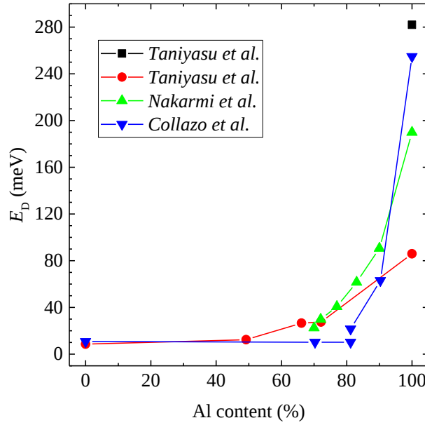
Figure 3.12: AlGaIn activation energy
