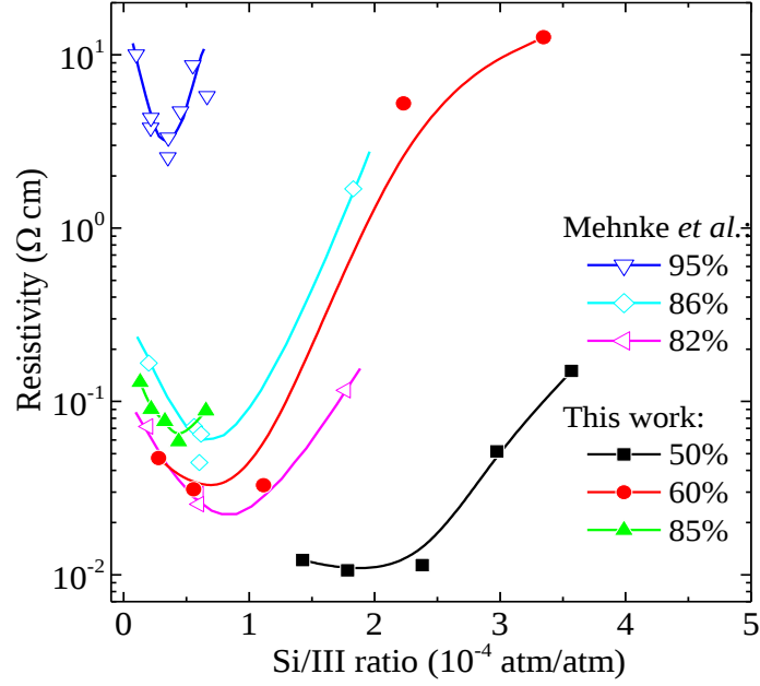
Figure 3.18: Doping optimization in AlGaIn
