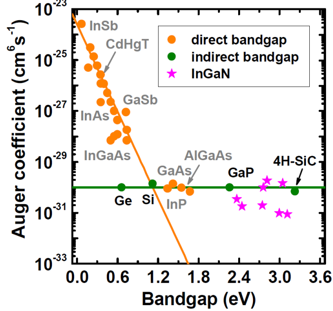
Figure 2.1: Auger Coefficient
