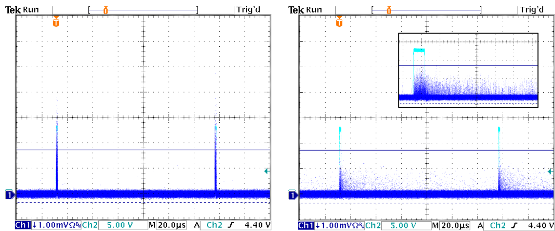
Figure 5.8: Oscilloscope screenshots
