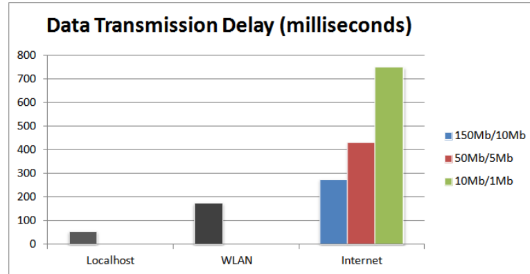
Figure 7.9: Data transmission delay with various networks
