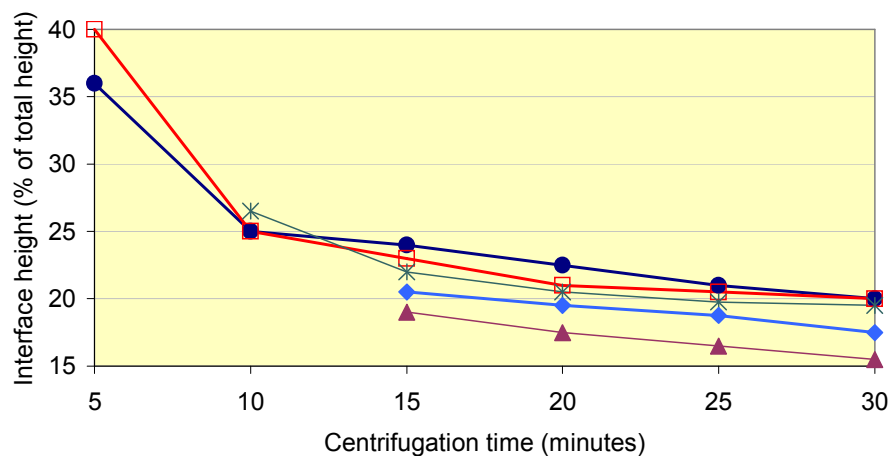
Figure 5.6 Rate of laboratory centrifugal settling of protein precipitate
