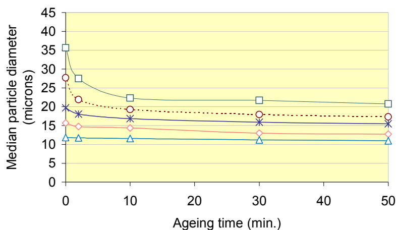
Figure 4.17 Effect of impeller shear-rate on median precipitate size in a 1.4 L agitation vessel for an ageing period of up to 3000 seconds at 1124 s -1 (high) following various acid addition impeller shear-rates (squares 398 s -1 (low); circles 580 s -1 (med-low); crosses 783 s -1 (med); diamonds 1006 s -1 (med-high); triangles 1247 s -1 (high)).
