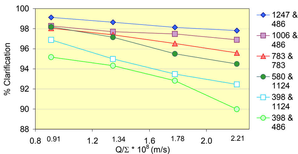
Figure 6.6 Disk stack centrifuge clarification curves for whey protein aggregates previously subject to various impeller shear-rates during acid addition and ageing in a 27 L batch agitation vessel (key displays shear-rates ( \text{s}^{-1} ) during acid addition (180 s) and ageing (3000 s) respectively).
