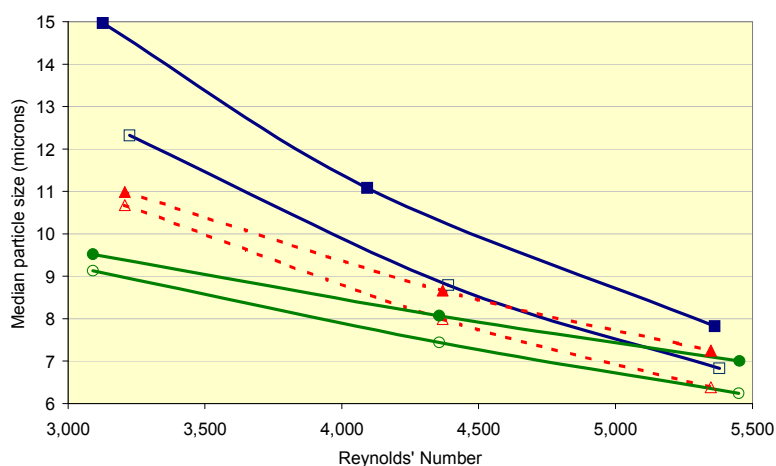
Figure 4.22 Effect of ageing time and capillary shear on median diameter of aggregates with various shear histories (squares represent an acid addition impeller shear-rate of 398 \text{ s}^{-1} (low), triangles are 783 \text{ s}^{-1} (med), circles are 1247 \text{ s}^{-1} (high); open symbols represent a subsequent ageing time of 600 s; closed symbols represent an ageing time of 3,000 s). Ageing impeller shear-rate is 486 \text{ s}^{-1} (low) throughout.
