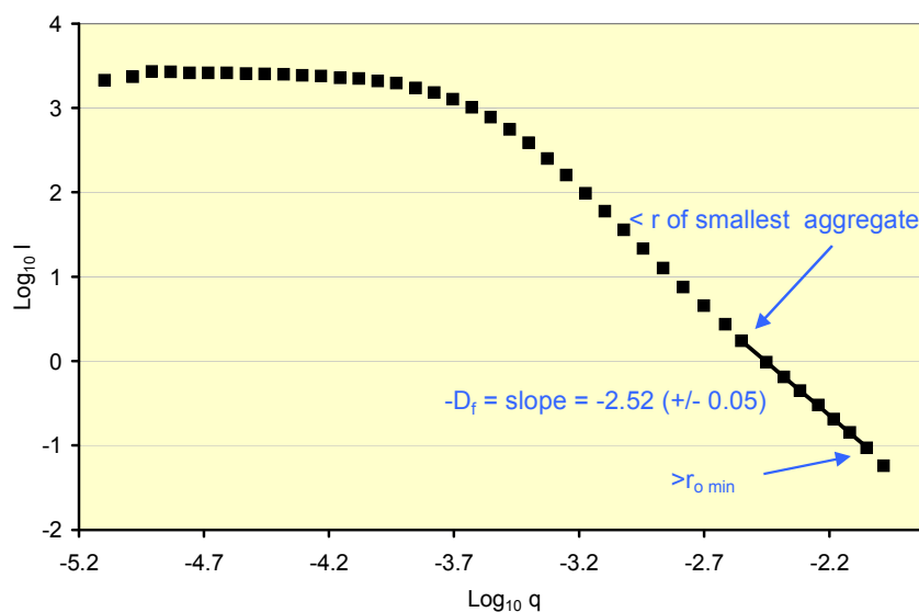
Figure 5.1 Log-log plot constructed to estimate fractal dimension using laser scattering data for precipitates subject to impeller shear-rate during acid addition of 783\text{s}^{-1} (med) followed by 3000 seconds of ageing at 486\text{s}^{-1} (low) in a 1.4L batch agitation vessel.
