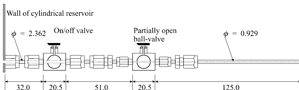
Figure 4.9 Ball-valve shearing rig and dimensions.
