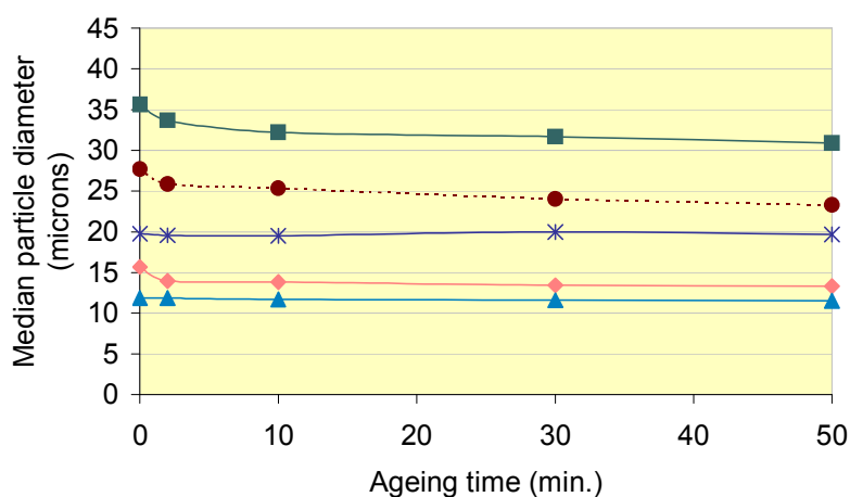
Figure 4.16 Effect of impeller shear-rate on median precipitate size in a 1.4 L agitation vessel for an ageing period of up to 3000 seconds at 486 s -1 (low) following various acid addition impeller shear-rates (squares 398 s -1 (low); circles 580 s -1 (med-low); crosses 783 s -1 (med); diamonds 1006 s -1 (med-high); triangles 1247 s -1 (high)).
