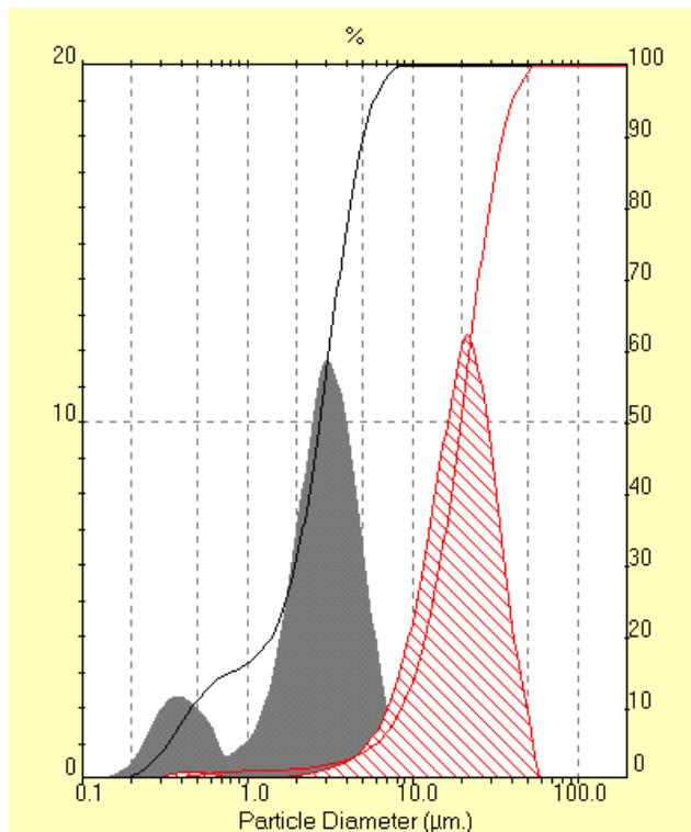
Figure 4.24 Effect of ball-valve shear on PSD of aggregates previously subject to an agitation vessel acid addition shear-rate of 398 \text{ s}^{-1} (low) followed by 3000 seconds ageing at 1124 \text{ s}^{-1} (high) (hatched represents pre-shear PSD, filled is post-shear).
