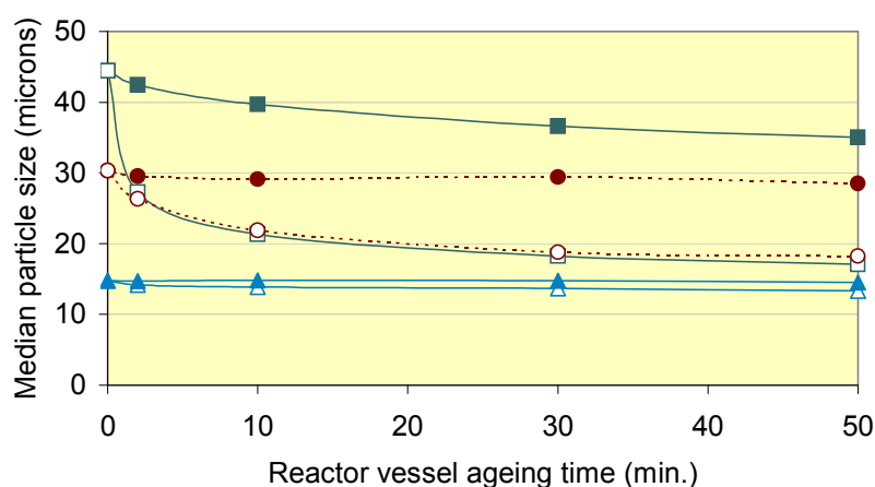
Figure 6.2 Effect of impeller shear-rate during acid addition and during ageing on median particle size in a 27 L agitation vessel (squares represent an acid addition impeller shear-rate of 398\text{ s}^{-1} (low), circles are 580\text{ s}^{-1} (med), triangles are 1247\text{ s}^{-1} (high); filled symbols represent an ageing impeller shear-rate of 486\text{ s}^{-1} (low), open symbols represent an ageing impeller shear-rate of 1124\text{ s}^{-1} (high)).
