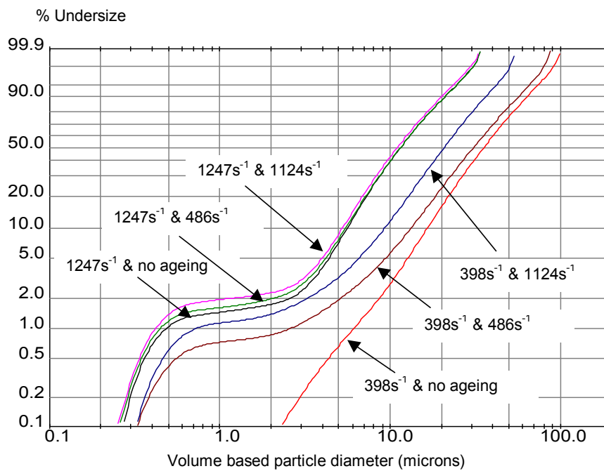
Figure 4.14 Effect of impeller shear-rates of 398\text{s}^{-1} (low) and 1247\text{s}^{-1} (high) on PSD of whey protein precipitates after 170 seconds of acid addition followed by various ageing regimes; none, 486\text{s}^{-1} (low) for 3000 seconds and 1124\text{s}^{-1} (high) for 3000 seconds.
