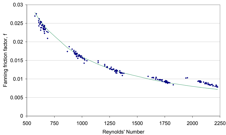
Figure 4.6 Actual Fanning friction factors and Reynolds' numbers for Newtonian 1% protein aggregate solution pumped through a 0.929 mm diameter pipe (curve represents relationship between Re and f for ideal laminar flow; f = 16/Re ).
