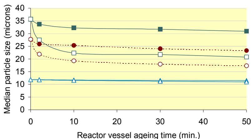
Figure 4.15 Effect of impeller shear-rate during acid addition and during ageing on median particle size in a 1.4 L agitation vessel (squares represent an acid addition impeller shear-rate of 398\text{s}^{-1} (low), circles are 580\text{s}^{-1} (med-low), triangles are 1247\text{s}^{-1} (high); filled symbols represent an ageing impeller shear-rate of 486\text{s}^{-1} (low), open symbols represent an ageing impeller shear-rate of 1124\text{s}^{-1} (high)).
