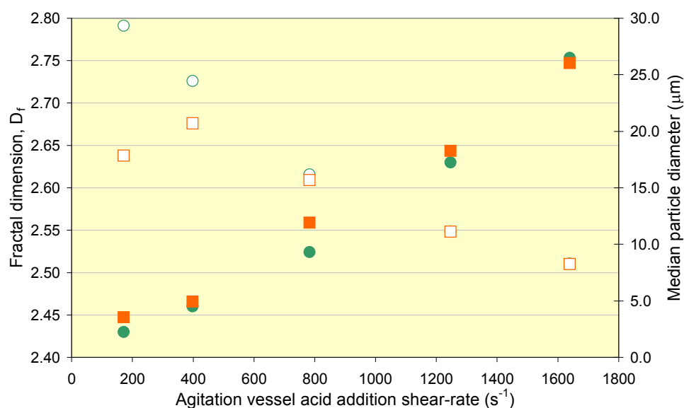
Figure 5.2 Fractal dimension (filled symbols) and size (open symbols) of aggregates formed by precipitation in a 1.4L batch agitation vessel subject to various impeller acid addition shear-rates followed by ageing at 486s^{-1} (low) (circles) and 1124s^{-1} (high)(squares) respectively for 3000 seconds.
