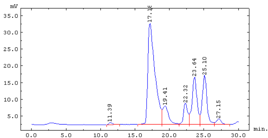
Figure 4.18 Typical HPLC profile of supernatant after 50 minutes ageing in agitation vessel.
