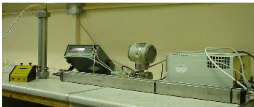
Figure 4.5 Capillary shearing rig (including pressure transducer and monitor) with timer.
