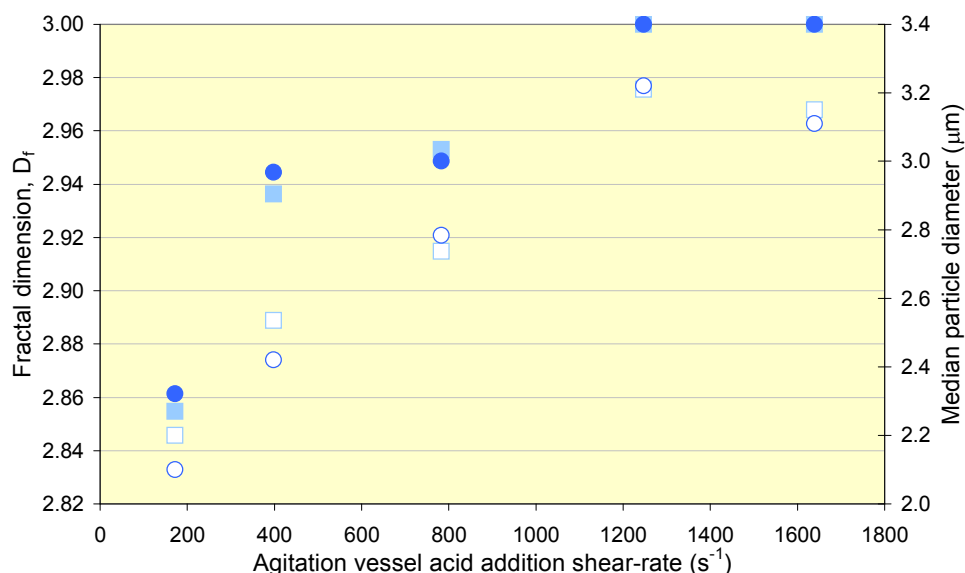
Figure 5.4 Fractal dimension (filled symbols) and size (open symbols) of aggregates subject to turbulent processing in a ball-valve rig after 1.4L batch agitation vessel precipitation at various acid addition impeller shear-rates followed by ageing at 486s^{-1} (low) (circles) and 1124s^{-1} (high) (squares) respectively for 3000 seconds.
