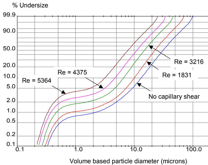
Figure 4.21 Effect of capillary shear on PSD of aggregates formed at agitator vessel shear-rate of 398\text{s}^{-1} (low) during acid addition followed by 3000 seconds of ageing at 486\text{s}^{-1} (low).
