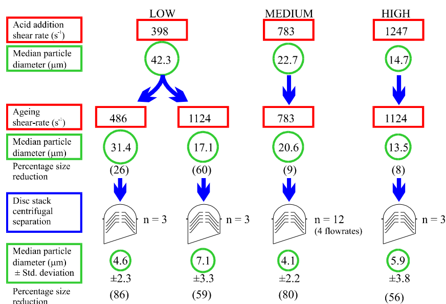
Figure 6.7 Effect of disc stack centrifuge processing on particle size on whey protein precipitates subject to various impeller shear-rates during acid addition and ageing in a 27 L batch agitation vessel.
