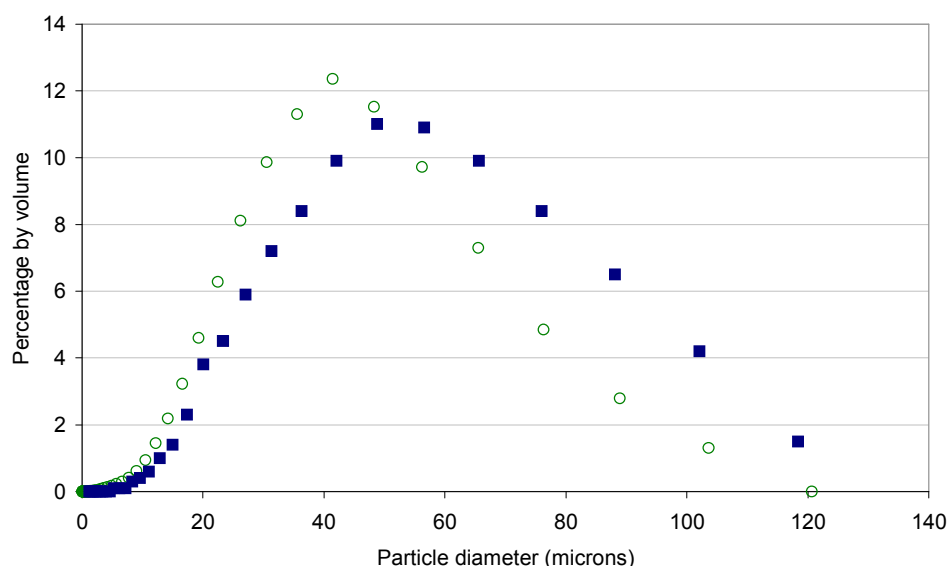
Figure 6.5 PSD curves for whey protein aggregates subject to average agitation vessel shear-rates of 398 \text{ s}^{-1} (low) during acid addition in 1.4 L (open) and 27 L (fill) standard configuration vessels.
