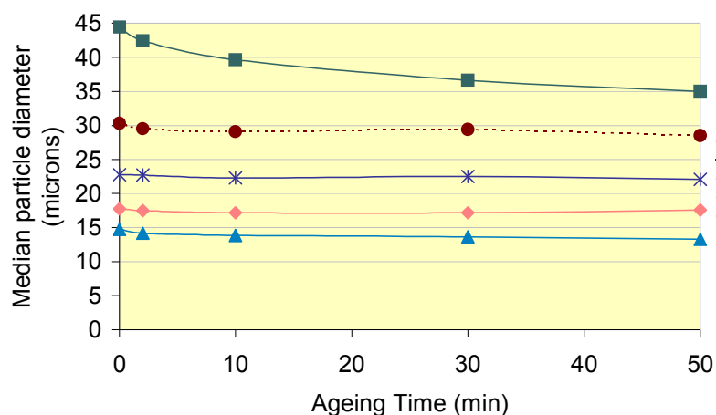
Figure 6.3 Effect of impeller shear-rate on median precipitate size in a 27 L agitation vessel for an ageing period of up to 3000 seconds at 486 s -1 (low) following various acid addition impeller shear-rates (squares 398 s -1 (low); circles 580 s -1 (med-low); crosses 783 s -1 (med); diamonds 1006 s -1 (med-high); triangles 1247 s -1 (high)).
