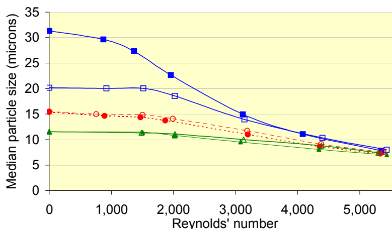
Figure 4.20 Effect of capillary shear on median particle size of aggregates with various shear histories aged for 3000 s (squares represent an acid addition impeller shear-rate of 398\text{s}^{-1} (low), circles are 783\text{s}^{-1} (med), triangles are 1247\text{s}^{-1} (high); closed symbols represent an ageing impeller shear-rate of 486\text{s}^{-1} (low), open symbols represent an ageing impeller shear-rate of 1124\text{s}^{-1} (high)).
