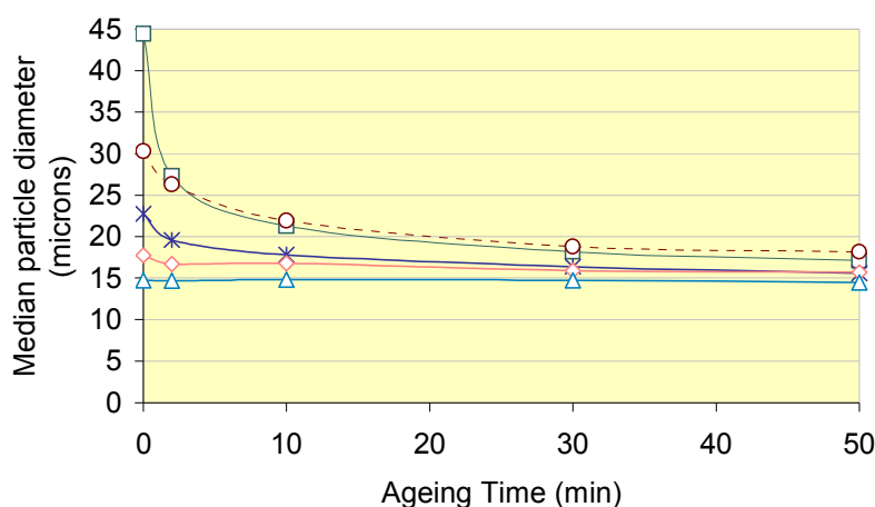
Figure 6.4 Effect of impeller shear-rate on median precipitate size in a 27 L agitation vessel for an ageing period of up to 3000 seconds at 1124 \text{ s}^{-1} (high) following various acid addition impeller shear-rates (squares 398 \text{ s}^{-1} (low); circles 580 \text{ s}^{-1} (med-low); crosses 783 \text{ s}^{-1} (med); diamonds 1006 \text{ s}^{-1} (med-high); triangles 1247 \text{ s}^{-1} (high)).
