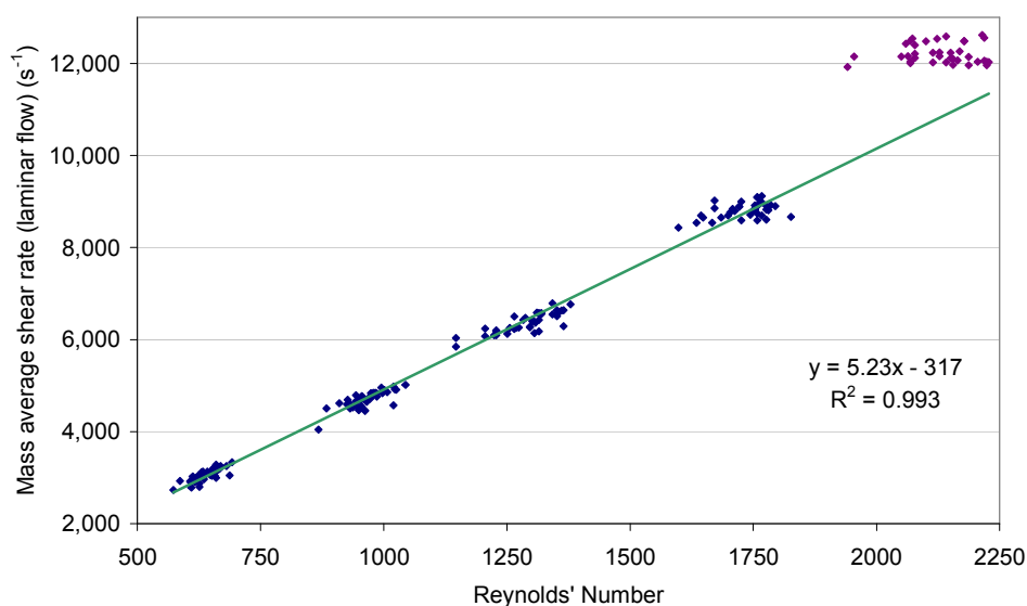
Figure 4.7 Predicted mass average shear-rate for laminar flow of a Newtonian 1% protein aggregate solution pumped through a 0.929 mm diameter pipe versus Reynolds' number.
