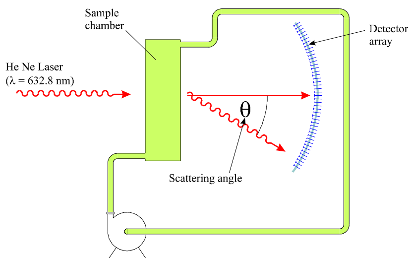
Figure 5.10 Schematic representation of light scattering and detection by Malvern.
