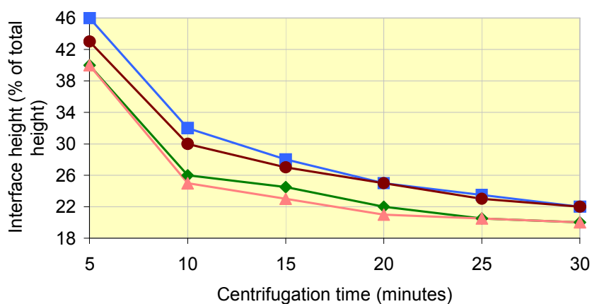
Figure 5.5 Rate of laboratory centrifugal settling of protein precipitate phase for aggregate solutions which have been subject to agitation vessel acid addition and ageing shear-rate of 523 \text{ s}^{-1} for various ageing times: squares 120 s; circles 600 s; diamonds 1800 s; triangles 3000 s.
