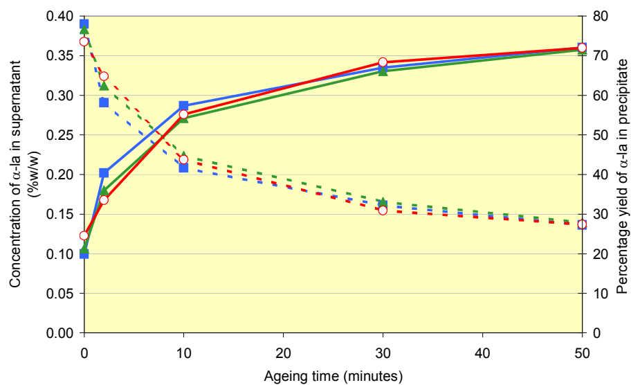
Figure 4.19 Absolute concentration (broken line) and percentage yield (filled line) of \alpha -lactalbumin in supernatant and precipitate phases respectively during ageing at impeller shear-rate 486\text{s}^{-1} (low) following acid addition at impeller shear-rates 398\text{s}^{-1} (low) (squares), 783\text{s}^{-1} (med) (triangles) and 1247\text{s}^{-1} (high) (open circles).
