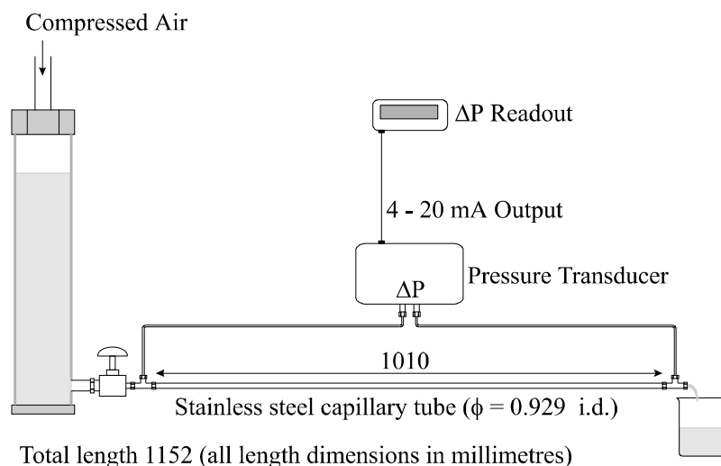
Figure 4.4 Capillary shearing rig and dimensions.
