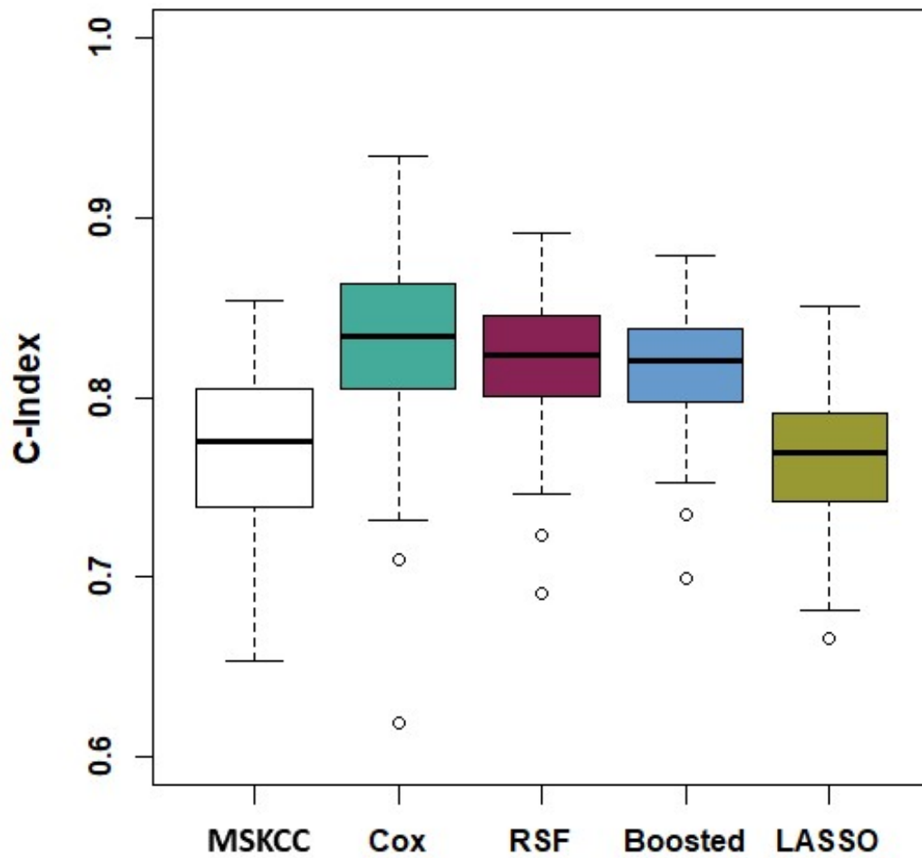
Figure 3.1: Bootstrap C-Index distributions of the MSKCC nomogram and the most competitive model pipelines using mRNA data. From left to right ; MSKCC, Cox model with clinical variables and correlation prefiltered mRNA variables, RSF model with clinical variables and correlation prefiltered and univariate Cox feature selected mRNA, Boosted Cox model with clinical variables and correlation prefiltered mRNA variables, LASSO Cox model with clinical variables and univariate Cox feature selected mRNA.
