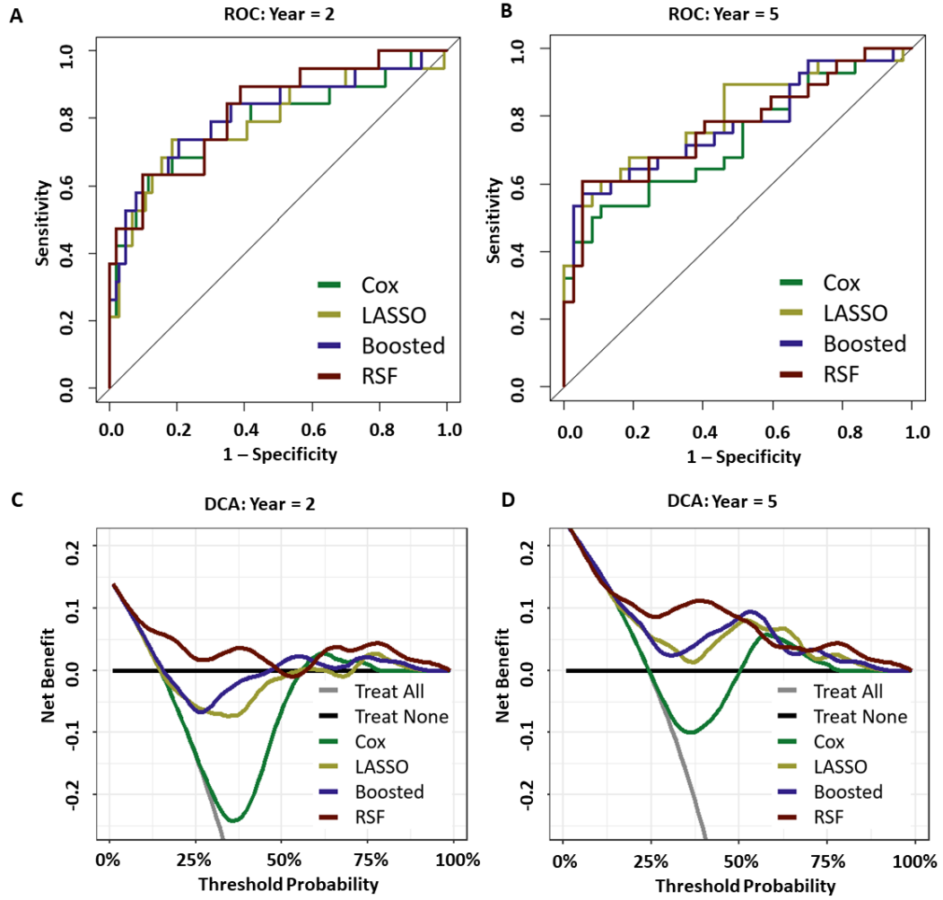
Figure 3.3: (A,B): ROC for 2-year (A) and 5-year (B) horizons. (C,D): DCA curves at the same horizons.
