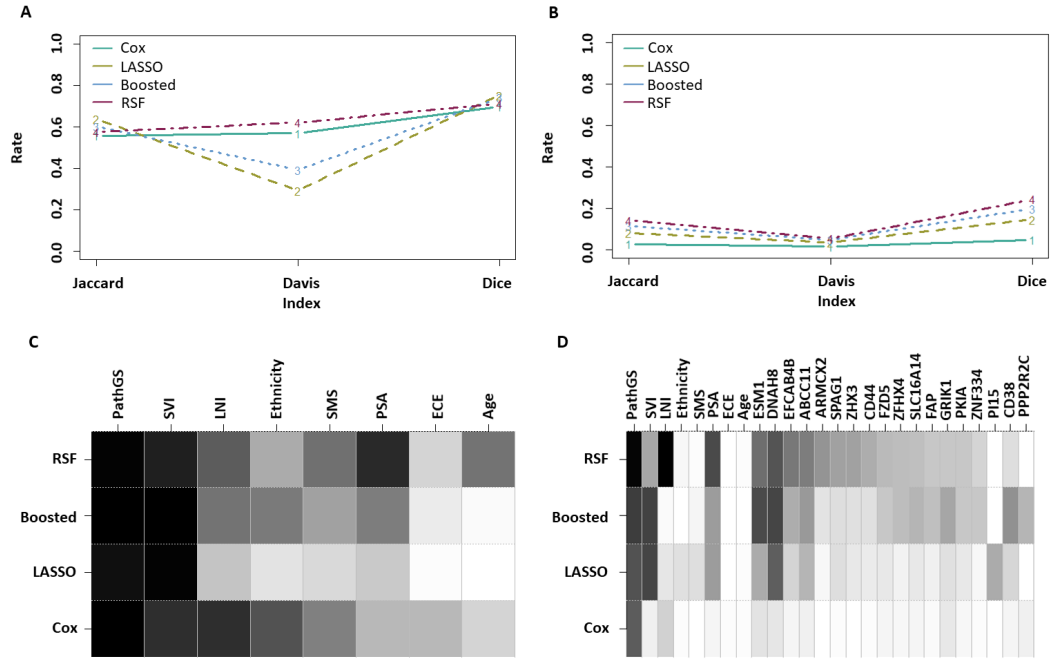
Figure 3.4: (A) Stability indices of the clinical-only models. (B) Stability indices of the top mRNA-inclusive pipelines. (C) Feature selection rates in clinical-only models (a darker shade indicates a higher rate). (D) Feature selection rates in the best-performing mRNA-inclusive pipelines, for features with a selection rate \geq 0.2 in at least one of these top pipelines. For comparative purposes, the shade of grey used for ESM1 in RSF corresponds to a 50% selection rate.
