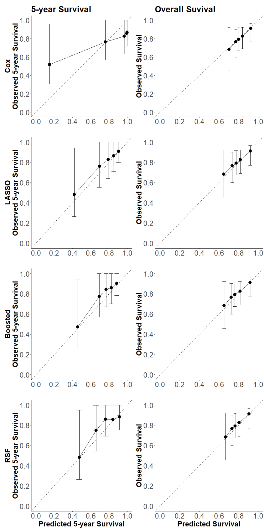
Figure 4.2: Model calibration curves. Model calibration curves at the 5-year horizon (left) and overall (right) BCR-free survival for the Cox, LASSO Cox, boosted Cox and RSF models from top to bottom, respectively with 95% confidence intervals.
