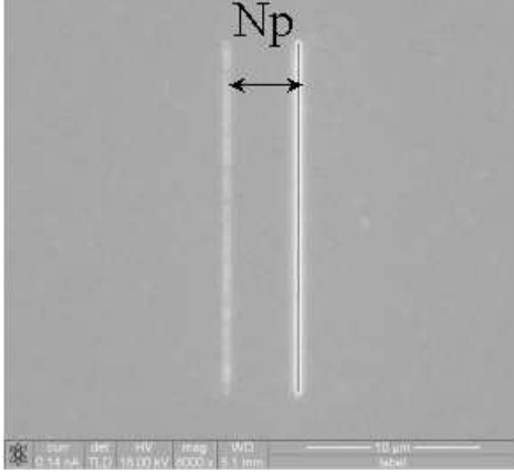
Figure 6. Scanning electron microscope (SEM) image of one of the series of single-slit, single-groove structures FIB milled into a 400 nm thick silver layer deposited on flat quartz microscope slides 1 mm thick. The width of both the slit and the groove is 100 nm, the height 20\mu\text{m} and the groove depth \sim 100 nm. The distance Np is the pitch increment p = 104\text{ nm} multiplied by the number of increments N .
