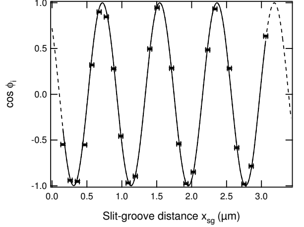
Figure 13. Wide-groove structures: Plot of the phase k_{cd}x_{sg} + \varphi_o as a function of x_{sg} with the detector rotated to \theta = 0 on a line perpendicular to the structure plane. Extrapolation of the phase as x_{sg} approaches zero, yields \varphi_0 = 0.24\pi \pm 0.01\pi .
