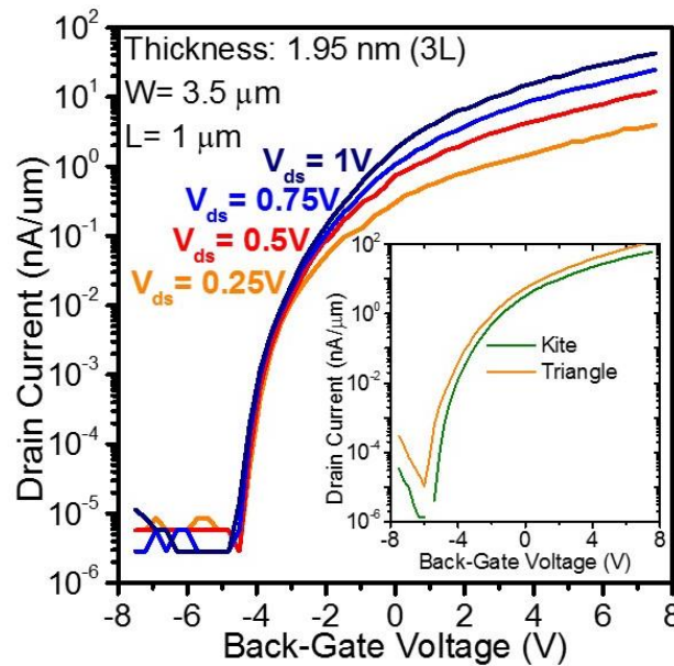
Figure 2: Transfer characteristics of the Trapezium at different drain-source voltages. Inset: transfer characteristics of the Kite and the Triangle at V_{ds}=1\text{V} .
