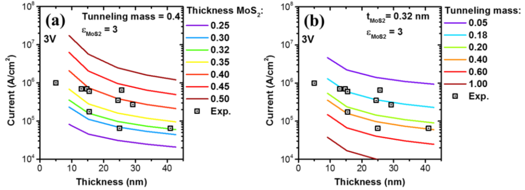
Figure 6: Current density at 3V for different thickness considering a variation of: (a) MoS 2 thickness with a fixed tunneling mass of 0.4, and (b) tunneling mass with a fixed thickness for the MoS 2 layer of 0.32 nm.
