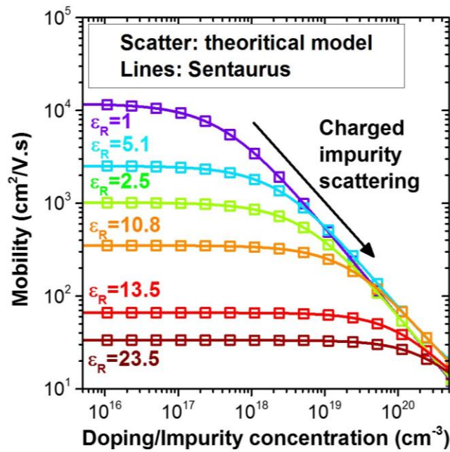
Figure 4: (a) Mobility versus impurity concentration considering different parameters implemented using the Arora mobility model. The theoretical model is based on DFT calculations for MoS 2 , 92 while the lines are the results obtained with the TCAD model.
