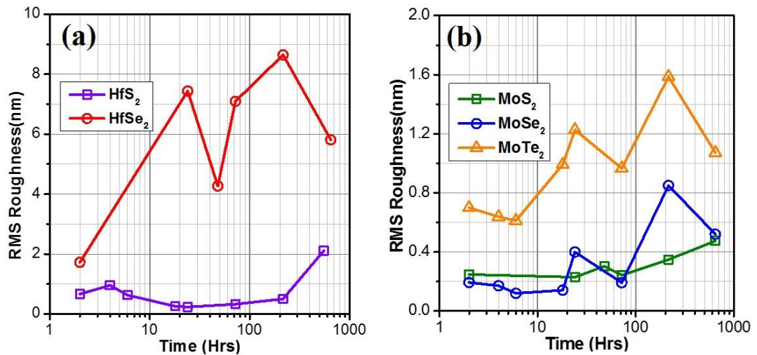
Figure 2: RMS surface roughness trends for (a) Hf-based and (b) Mo-based TMDs. Note the difference in the y-axis scales.
