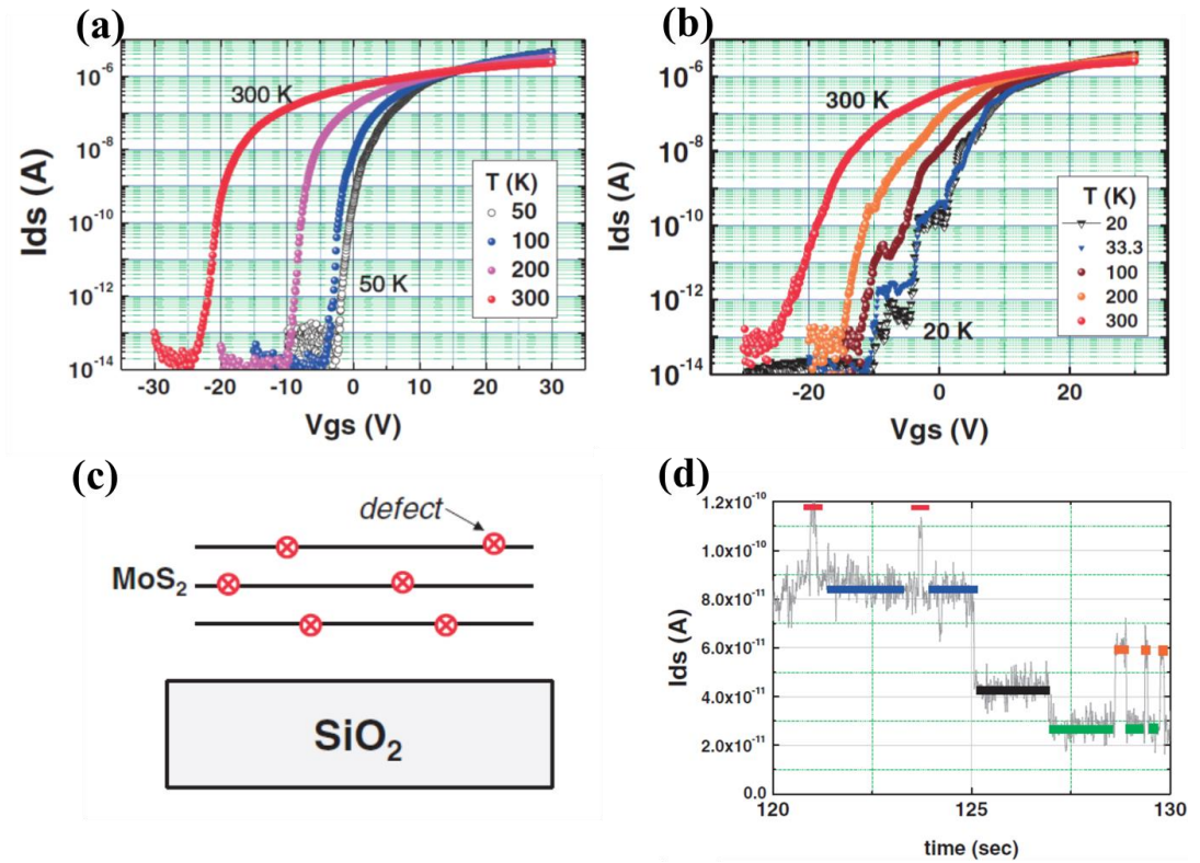
Figure 8: Subthreshold characteristics of (a) multilayer and (b) monolayer MoS 2 at different temperature. The monolayer device clearly shows the presence of active defects, on the contrary of the multilayer device (c) Schematic illustration of the multilayer device to show the difference between the multi- and mono-layer device, as in a multilayer device a defect can be screened by carrier in the adjacent layers. (d) Example of temporal characteristic of monolayer MoS 2 at 20K showing several current levels. 118
