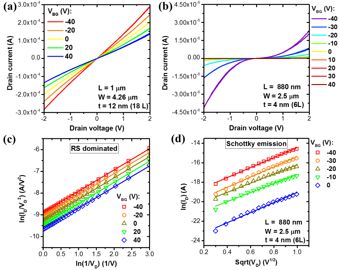
Figure 6: Output characteristics of the (a) 12 nm thick device and (b) 4 nm thick device. The output characteristic of the 12 nm thick device can be modelled considering direct tunnelling, which means that the behaviour is dominated by the resistance of the semiconductor (RS). Instead, the 4 nm thick sample can be modelled considering the Richardson-Schottky equation, pointing to a Schottky emission behaviour.
