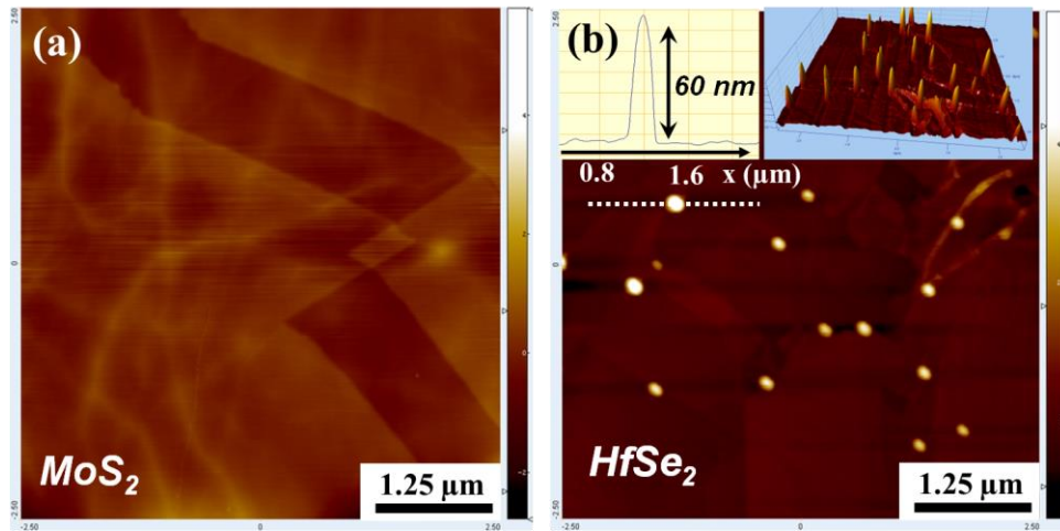
Figure 1: (a) Representative \text{MoS}_2 AFM image taken 24 hours after exfoliation. (b) Representative \text{HfSe}_2 AFM image taken 24 hours after exfoliation. The insets show cross-section of the tallest protrusion found on \text{HfSe}_2 of approximately 60 nm (white line scan in the main Figure), and a 3D representation of the data.
