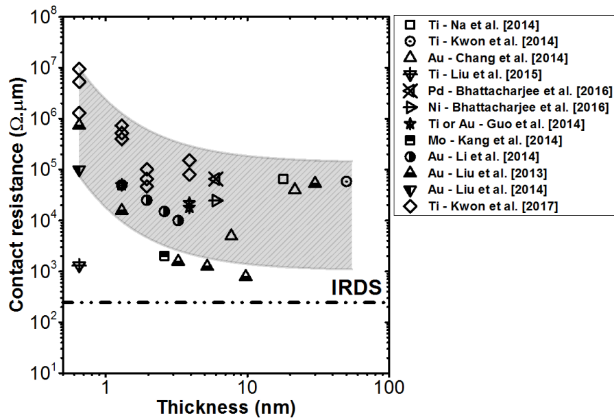
Figure 9: Summary of contact resistance values found in literature considering as-exfoliated devices. The gray area shows the general trend of contact resistance, characterized by high variability and excessive high values.
