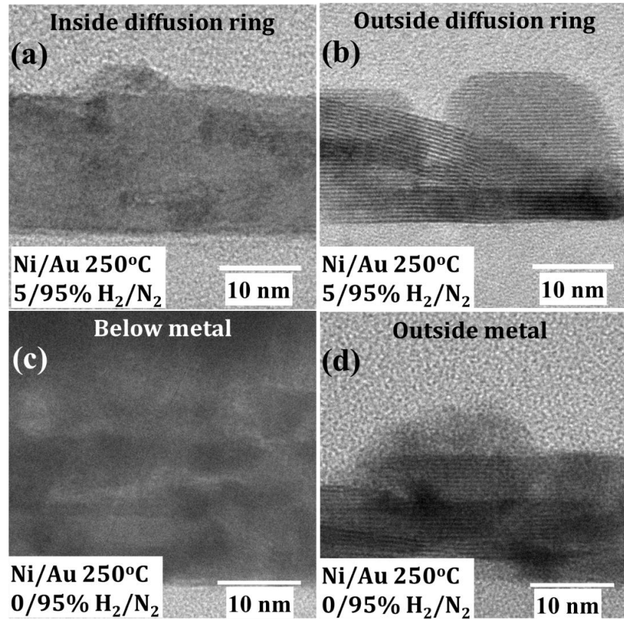
Figure 4: Representative cross-section TEM images of the PtSe 2 contacted with Ni/Au. (a) and (b) show the PtSe 2 after annealing in forming gas at 250 °C inside and outside the diffusion ring respectively. (c) and (d) show the PtSe 2 after annealing in inert environment at 250 °C below the metal contact and outside the metal contact respectively.
