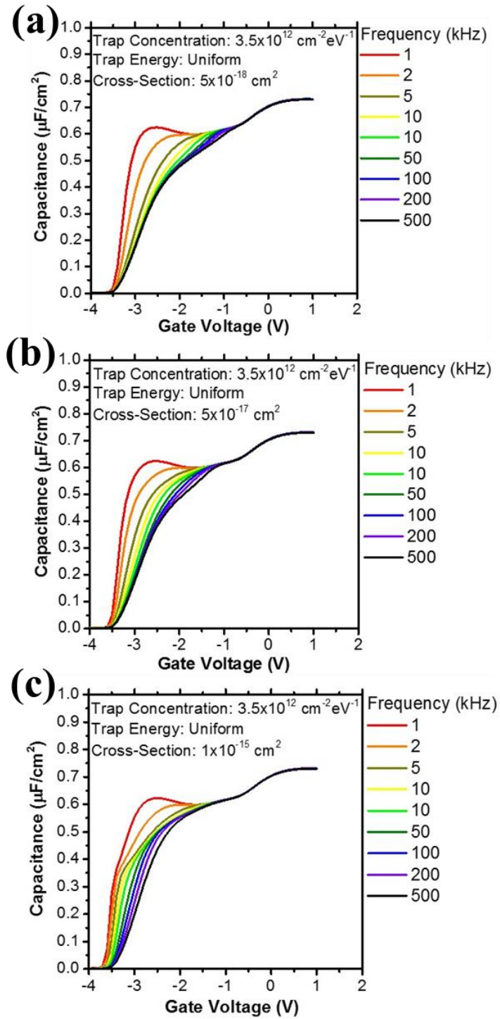
Figure 12: Simulated CV response of the single energy level traps at 0.925 eV in addition to the uniform trap, which cross-section: (a) 5 \times 10^{-18} \text{ cm}^2 , (b) 5 \times 10^{-17} \text{ cm}^2 and (c) 10^{-15} \text{ cm}^2 .
