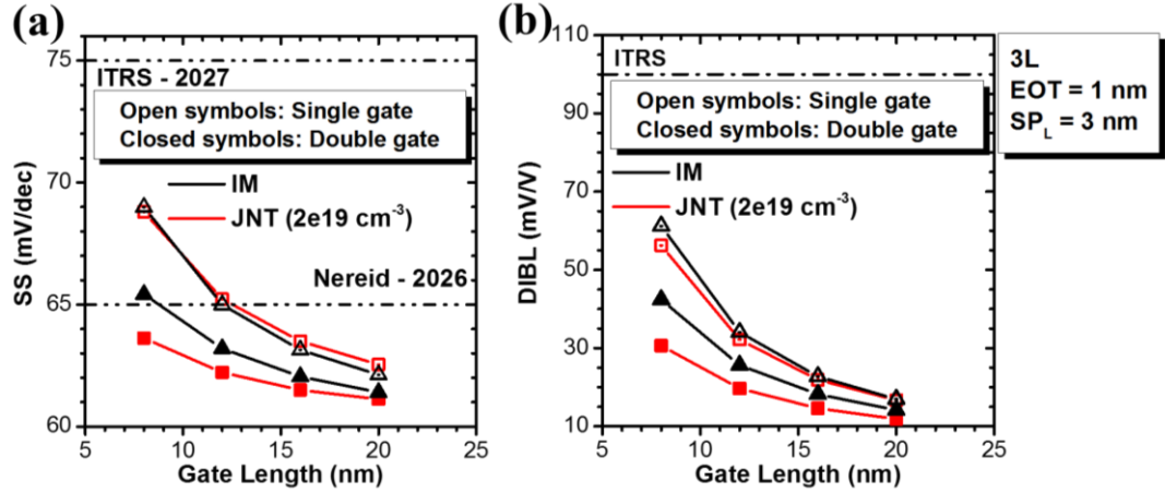
Figure 9: Comparison of JNT and IM in a single and double gate architecture considering (a) subthreshold slope and (b) DIBL. Same legend applied to both plots.
