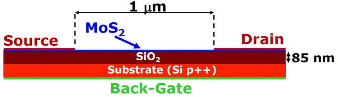
Figure 3: Schematic of a typical back-gated device structure implemented in Sentaurus device
