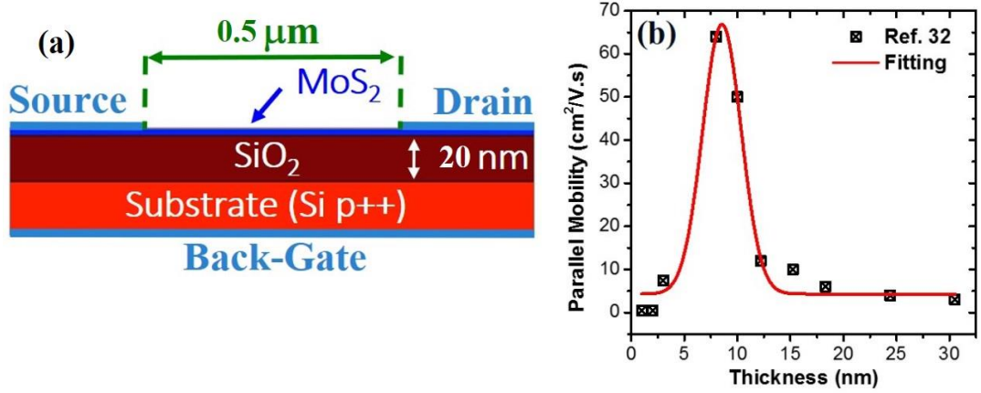
Figure 4: (a) Schematic of the device structure implemented in Sentaurus device. (b) Layer dependent parallel mobility used for both structures. 284
