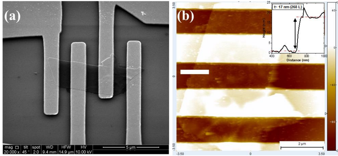
Figure 1: (a) SEM image of a typical contacted flake. (b) Representative AFM image of the same flake in (a). The white bar denotes where the cross-section was taken from. Inset: cross-section of the flake with its thickness ( \sim 17 nm).
