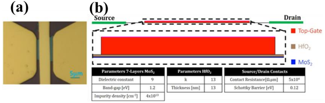
Figure 8: (a) Optical view of the top-gated MoS 2 flake. 273, 274 Ti/Au contacts are deposited under High Vacuum using photolithography and lift-off. HfO 2 was deposited by Atomic Layer deposition. Cr/Au was deposited as the metal gate. (b) Schematic of the structure implemented in the Sentaurus physics-based device simulator. The tables show the parameters selected for MoS 2 , HfO 2 and the Ti/MoS 2 contacts.
