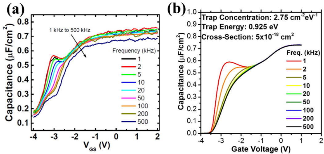
Figure 11: (a) Experimental 274 and (b) simulated CV response. The simulated CV response consider the trap at energy 0.925 eV, with concentration 2.75 \times 10^{12} \text{ cm}^{-2} and a cross-section value of 5 \times 10^{-18} \text{ cm}^2 .
