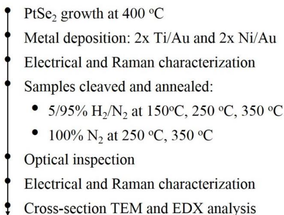
Figure 1: Experimental steps taken during this work.
