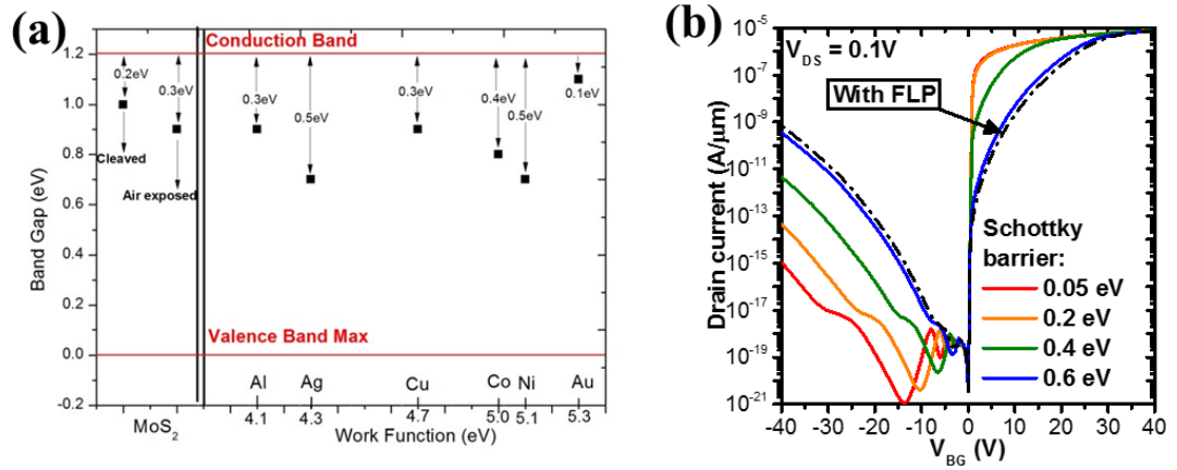
Figure 6: (a) High energy XPS measurements conducted on MoS 2 crystals with different metals. (b) Simulated transfer characteristics varying the Schottky barrier at the source and drain contacts. The structure of the simulated device is as reported in Figure 2: 1L of MoS 2 with 1 \mu m of channel length.
