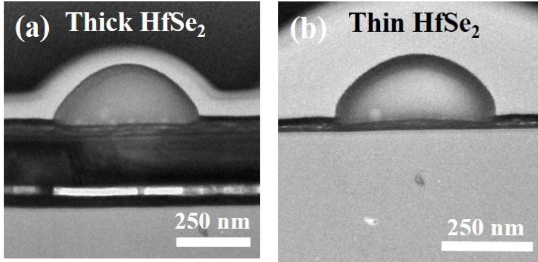
Figure 6: Representative TEM images of HfSe 2 after 5 months from exfoliation. Hemispherical shaped surface features appear amorphous in nature and are of similar dimensional size on both the (a) thick and (b) thin flakes.
