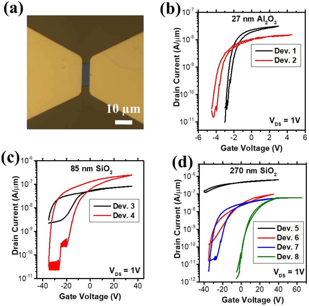
Figure 6: (a) Optical picture of a typical back-gated device structure. Transfer characteristics for the devices (dev.) exfoliated on (b) 27 nm of \text{Al}_2\text{O}_3 , (c) 85 nm of dry thermal \text{SiO}_2 and (d) on 270 nm wet thermal \text{SiO}_2 at a drain voltage of 1V. The devices were numbered to distinguish them.
