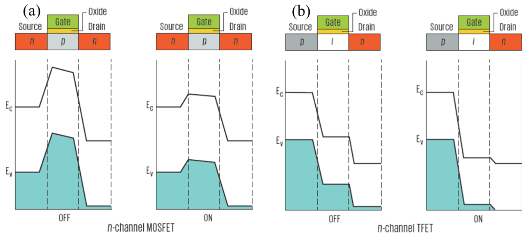
Figure 5: Comparison of band diagrams of (a) a n-channel MOSFET and (b) a n-channel TFET during off and on operation, showing the main difference between their working principle. The terms E_c and E_v refer to the minimum energy of the conduction band and maximum energy of the valence band, respectively. Adapted from 78
