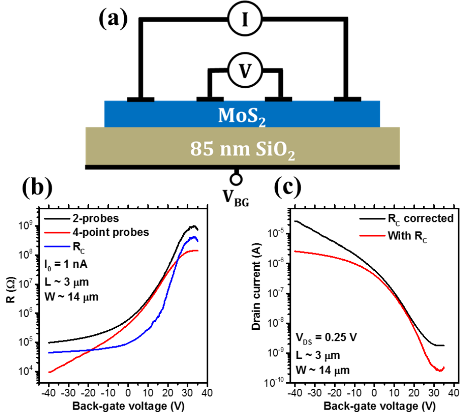
Figure 2: (a) Schematic of the device architecture used in this work. The external metal contacts are used to force a current in the device. Considering then the voltage drop across the two inner contacts, the resistance of the contact is extracted. (b) Example of 2-probe measurements (across the two inner pads), 4-point probe measurements and the extracted contact resistance. (c) Transfer characteristic of the same device from 2-point probe measurement (with R_c ) and without the effect of R_c .
