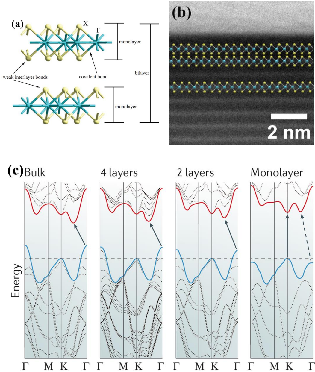
Figure 4: (a) Typical crystal structure of a TMD. 13 (b) Transmission electron microscopy cross section of a MoTe 2 exfoliated flake. Superimposed the crystal structure to emphasize the layered nature of these materials. (c) Bandgap evolution with respect of number of layers of MoS 2 , from monolayer to bulk. 17
