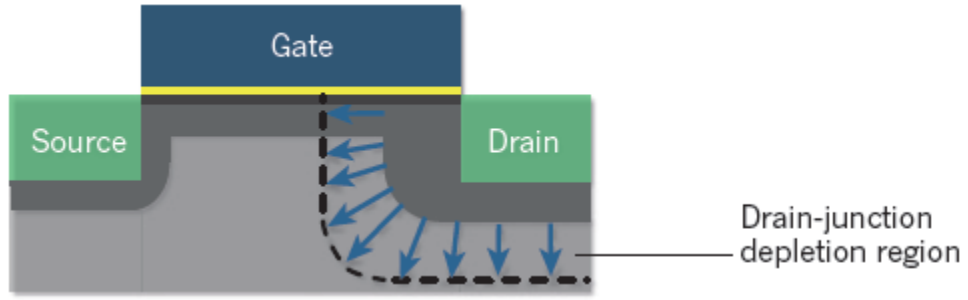
Figure 2: example of drain-junction depletion region, responsible for short-channel effects. 5
