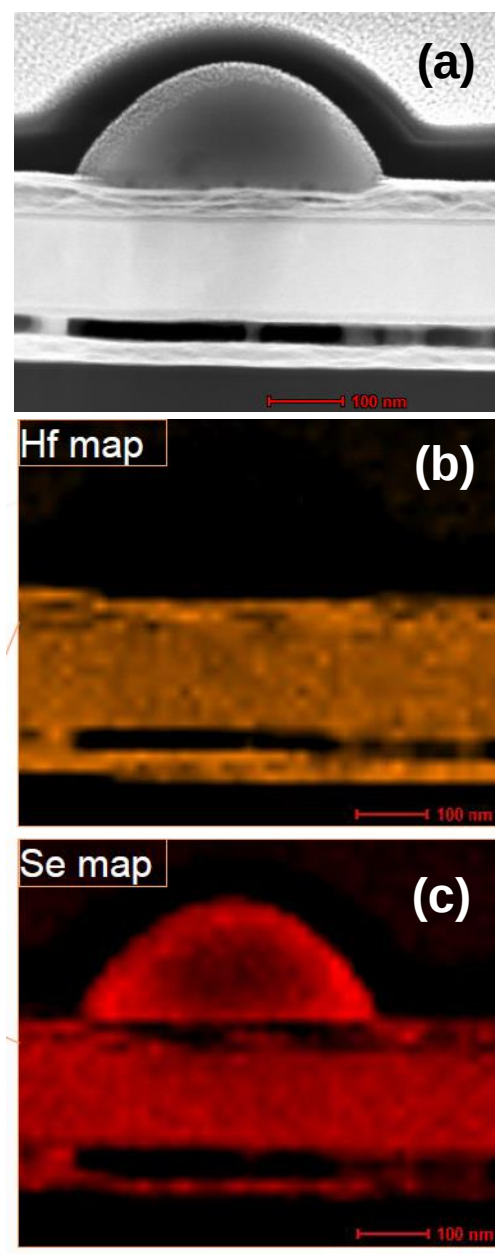
Figure 8: EDX data showing (a) the region mapped, (b) the Hf map, and (c) the Se map within the HfSe 2 flake and surface blister. The blister is Se-rich with little or no Hf present. The regions below the blister are depleted of Se.
