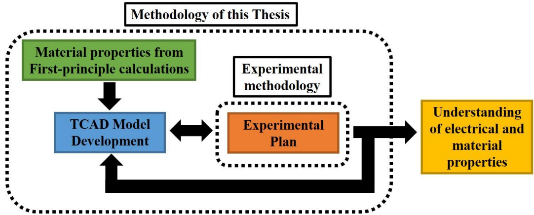
Figure 11: Schematic of the methodology used in this thesis in order to develop a TCAD model for MoS 2 based on both first-principle calculations and experimental data.
