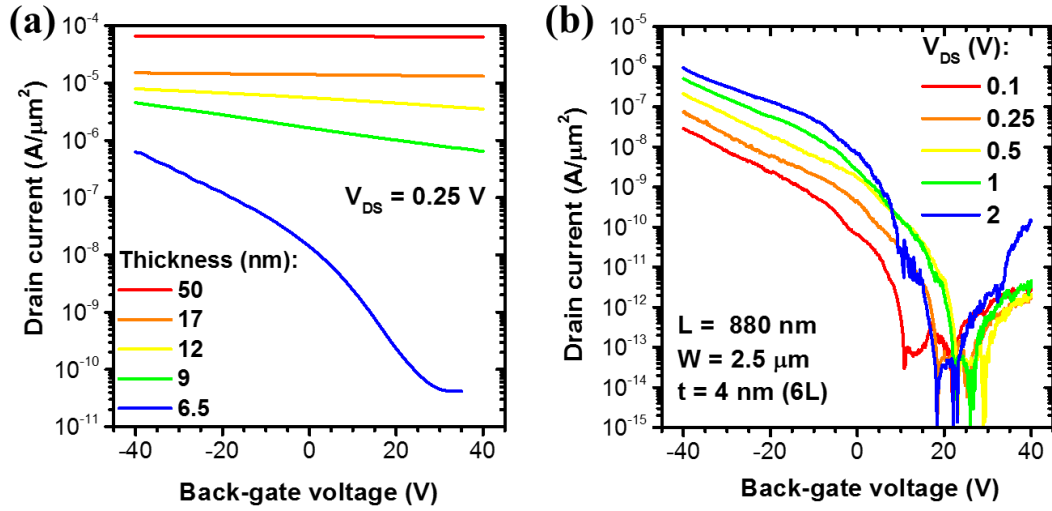
Figure 5: (a) Transfer characteristics of each device studied in this work. There is a clear dependence of the I_{ON}/I_{OFF} ratio with thickness because of the high doping concentration and the inability to completely deplete the channel. (b) Transfer characteristic of a thinner Nb-doped MoS 2 , showing much higher defective behaviour.
