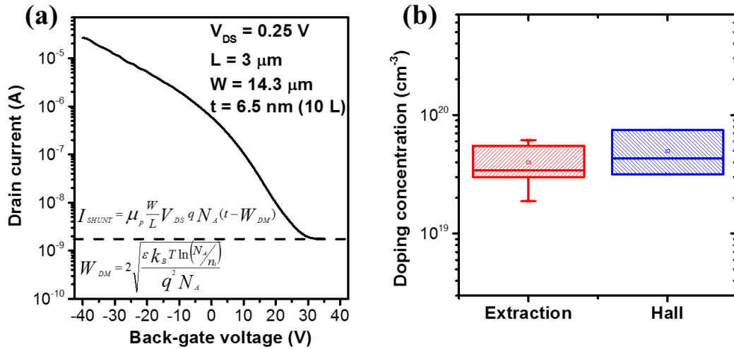
Figure 3: (a) Transfer characteristics of the 6.5 nm thick device showing the shunt current level, the equation for the shunt current and the equation for the maximum depletion width. (b) Average doping concentration from the extraction process using the transfer characteristics and the Hall measurements.
