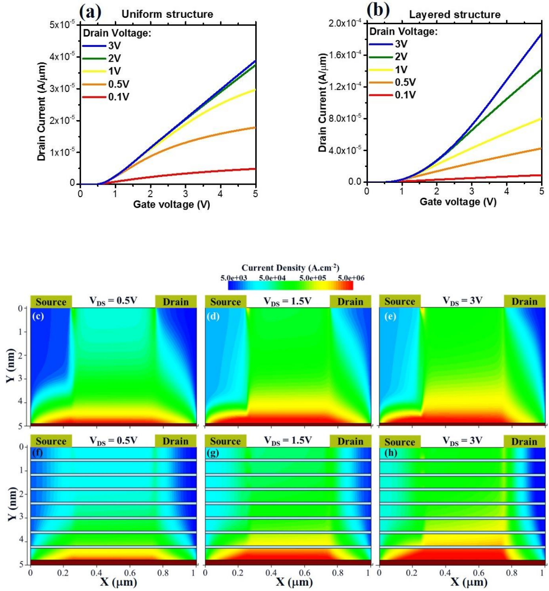
Figure 5: Transfer characteristic for the (a) uniform and (b) layered structure varying the drain voltage from 0.1 to 3V. Current density contour plot varying the drain voltage from 0.5 to 3V for the (c-e) uniform and (f-h) layered structure. Gate voltage is 5V ( V_{GS}-V_T \cong 3V ).
