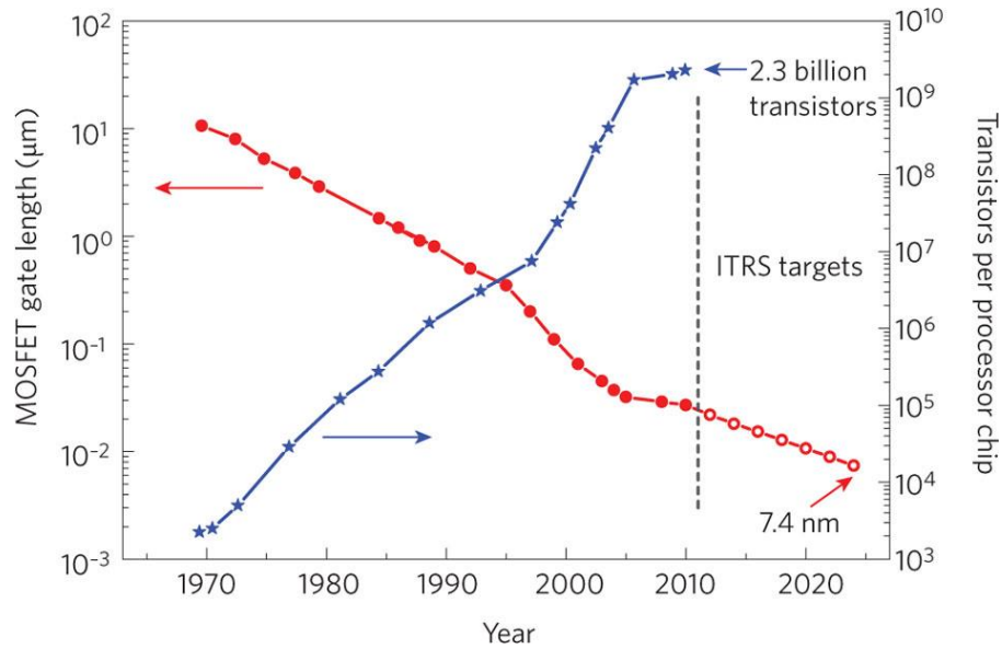
Figure 1: Trend of gate length and number of transistors per processor chip per year. 4
