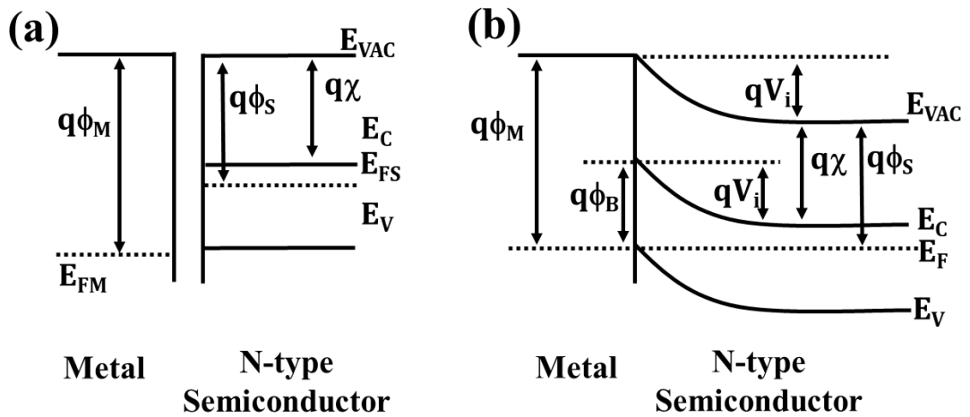
Figure 10: Schematic of the energy band diagram of metal and n-type semiconductor (a) before and (b) after making contact.
