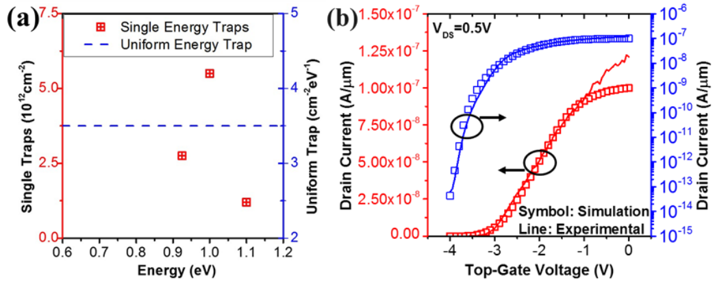
Figure 9: (a) Trap distribution with respect to the valence band edge of MoS 2 . The traps span from the mid-gap (0.6 eV) to the lowest energy in the MoS 2 conduction band. (b) Transfer characteristics of the experimental and the simulated devices in log (blue) and linear (red) scales. The fit of the simulated response to the experimental transfer characteristic is obtained using the interface trap distribution shown in Figure 6a.
