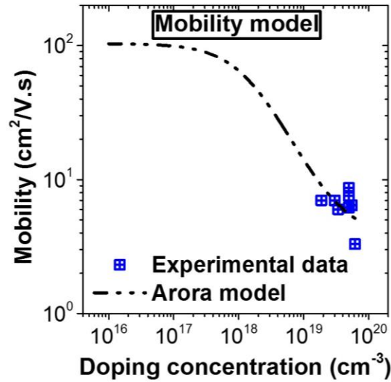
Figure 8: Mobility model used for the electrical simulations. The Arora model was tuned assuming a mobility value of \sim 100 \text{ cm}^2/\text{V.s} for a doping concentration of 10^{17} \text{ cm}^{-3} and the experimental data from Chapter 4 for the high-doping region.
