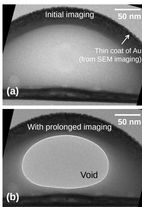
Figure 7: TEM imaging of the blisters on the thin HfSe 2 flake shows that (a) during initial imaging the blister is continuous and that (b) after a few minutes of electron irradiation a void is formed in the middle.
