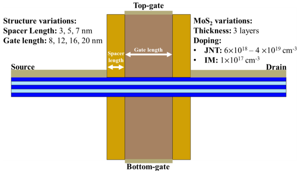
Figure 7: Double gate device structure considered for the TCAD simulations. For the IM architecture the source and drain regions will be considered metallic, while the channel will be uniformly doped for the JNT structure. values. 109
