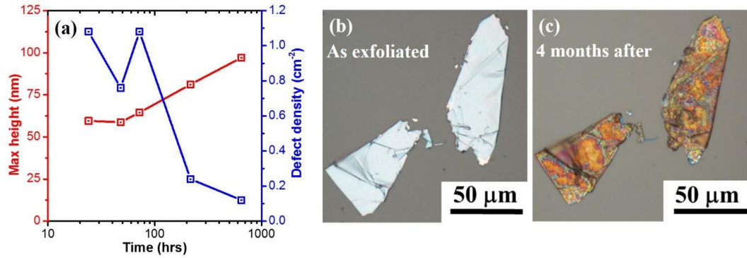
Figure 3: (a) Maximum height of the blister and defect density found for \text{HfSe}_2 . Optical pictures of \text{HfSe}_2 (b) as exfoliated and (c) 4 months after.
