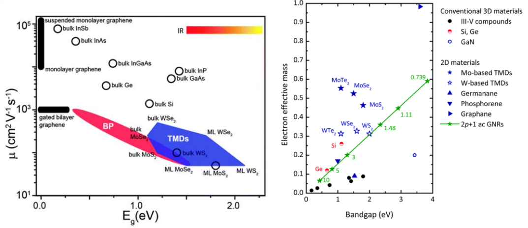
Figure 6: (a) Plot of mobilities versus band gap for TMDs, Si, Ge and III-Vs. The color scale represents the energy range of visible and infrared light with respect to the band gap energy. 100 (b) Electron effective mass versus bandgap. III-V data are InSb, InAs, \text{In}_{0.53}\text{Ga}_{0.47}\text{As} , InP, GaAs, \text{Al}_{0.3}\text{Ga}_{0.7}\text{As} from left to right. 88
