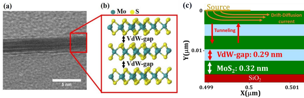
Figure 1: (a) Representative TEM image showing the layered structure of MoS 2 . (b) Representation of the structure of MoS 2 showing the Van-der Waals gaps between the layers. 277 (c) Schematic of the layered structure implemented in the Sentaurus physics based device simulator.
