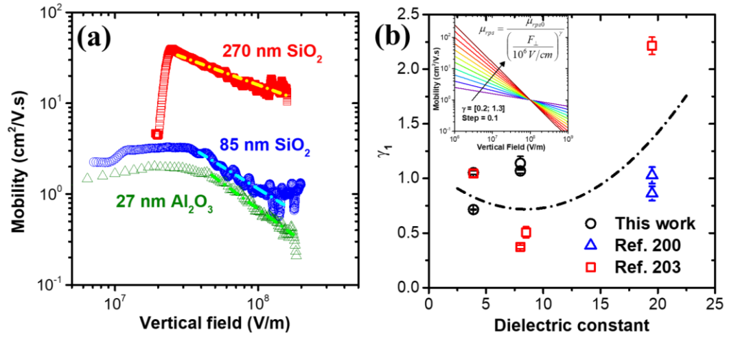
Figure 8: (a) Mobility extracted from experimental devices considering different substrates. The dotted line refers to the fitting with Equation 4. (b) Trend of \gamma_1 with respect of the dielectric constant of the gate dielectric. Inset: mobility degradation at high vertical field for increasing value of \gamma_1 .
