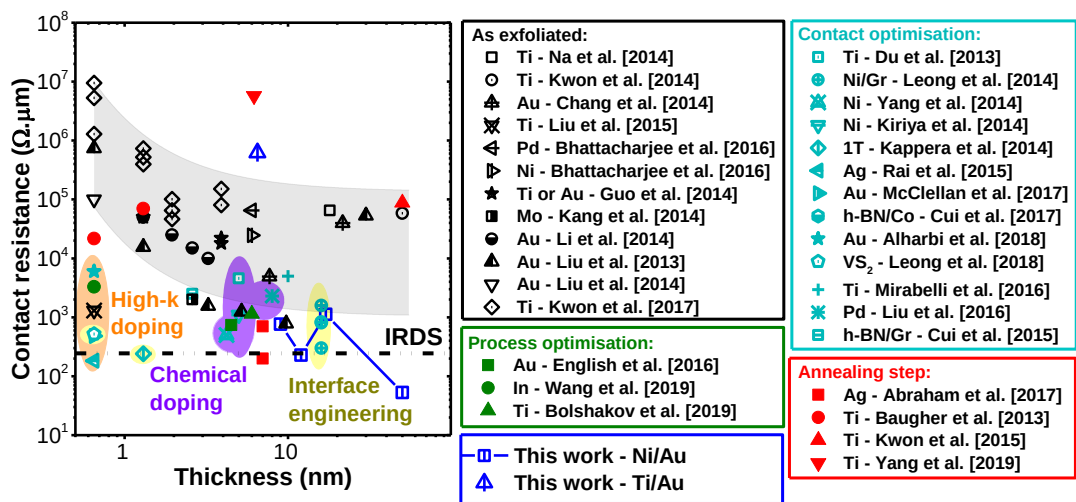
Figure 4: Contact resistance versus thickness of MoS 2 considering Ti/Au and Ni/Au contacts (Blue). The data are compared with other techniques to reduce contact resistance: high-k doping, chemical doping and interface engineering.
