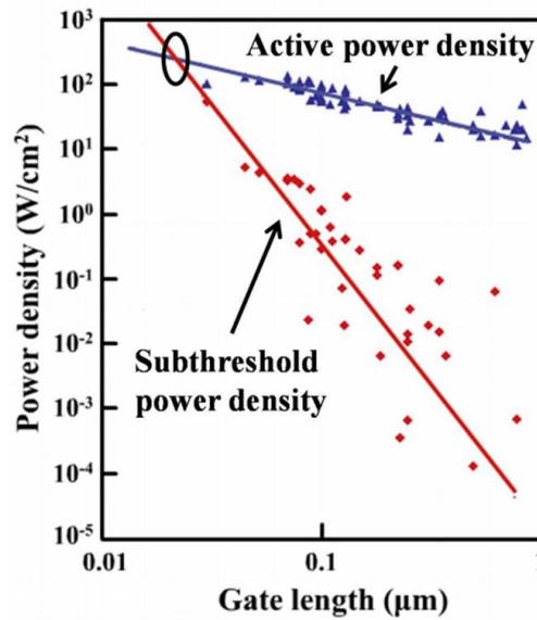
Figure 3: Active and subthreshold power densities for Si MOSFETs with respect of gate length. The cross-over point at 20-nm gate length indicates where subthreshold power density surpasses active power density. 10
