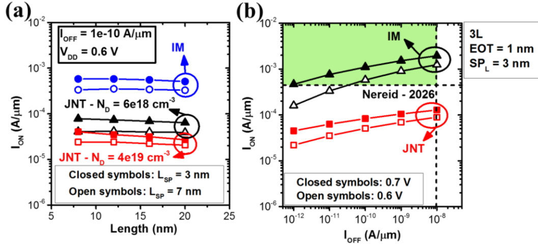
Figure 10: (a) I_{\text{ON}} scaling versus length at V_{\text{DD}} = 0.6 \text{ V} for an I_{\text{OFF}} of 1\text{e-}10 \text{ A}/\mu\text{m} and varying the spacer length between 3 and 7 nm. The IM architecture can drive a current almost one order of magnitude higher with respect of the JNT architecture. (b) I_{\text{ON}} versus I_{\text{OFF}} comparison at a V_{\text{DD}} of 0.6 and 0.7 V for the IM and JNT architecture at a channel length of 8 nm. The green box shows the I_{\text{ON}}/I_{\text{OFF}} region where the condition set by the IRDS is respected.
