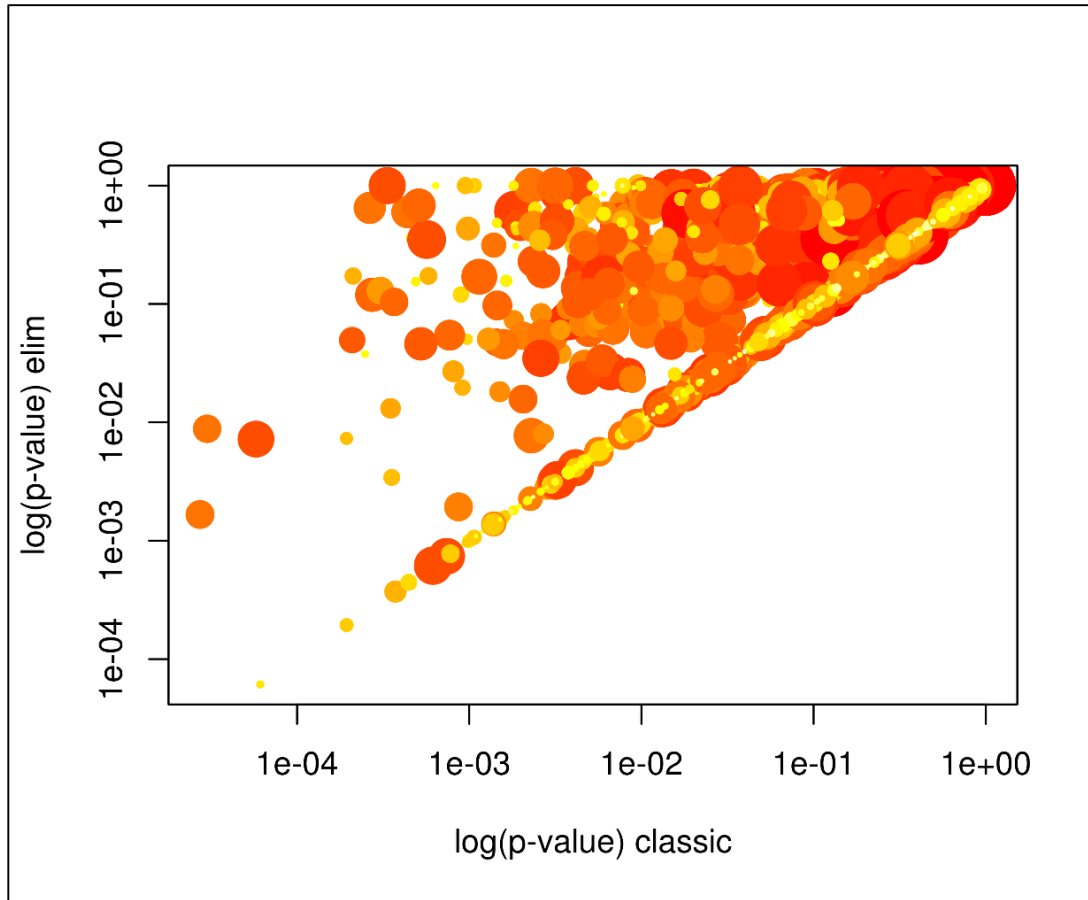
Figure 6.19: Scatter plot for significantly enriched GO terms predicted to be associated with differentially expressed miRNAs. The horizontal axis shows Fisher test results and the vertical axis shows the results by the Elim method. Values along the diagonal are consistent between both methods. The size of the dot is proportional to the number of genes mapping to that GO term and the colouring represents the number of significantly expressed genes corresponding to that term with dark red representing more terms and yellow representing fewer.
