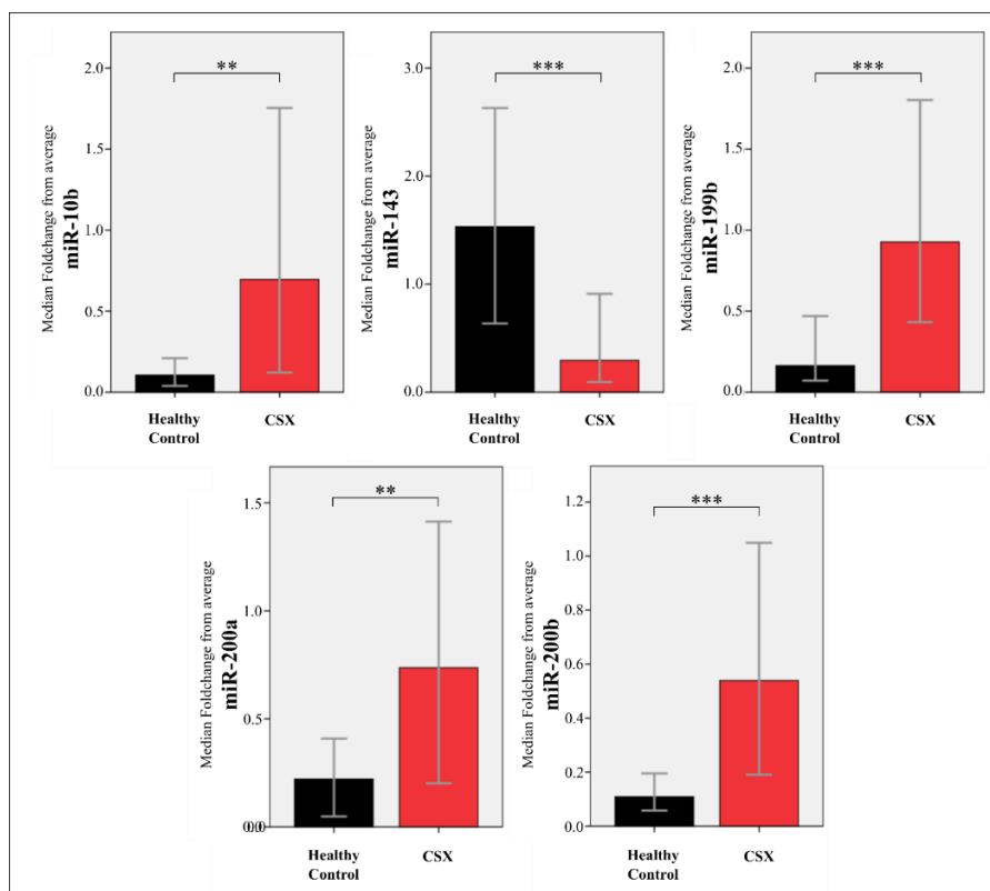
Figure 6.18: PCR Results. Bar charts of the median foldchange in expression when compared to the average expression level
