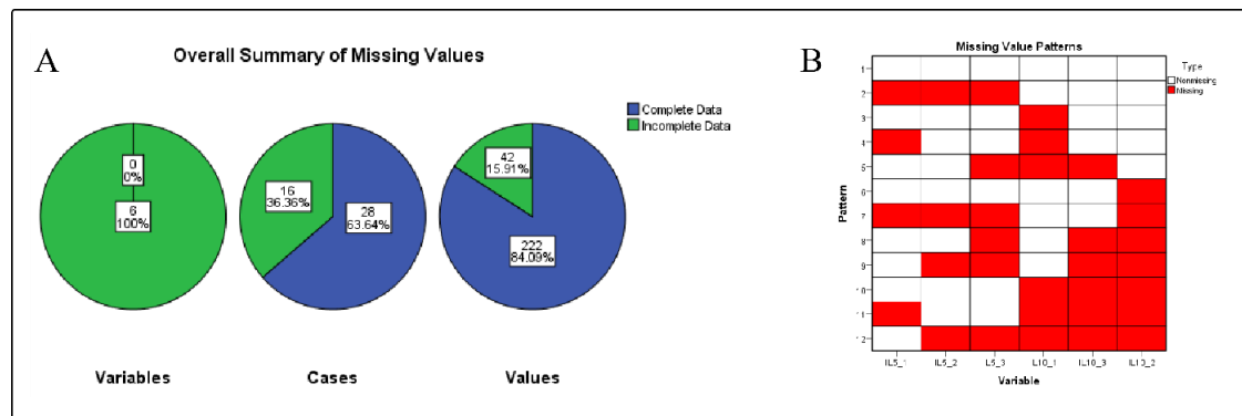
Figure 4.2: Missing Data Analysis prior to multiple imputation. A. Pie charts showing the number of cases with at least one missing value and also the overall number of missing values. B. Missing Value Pattern grid showing no monotonic pattern in our dataset.
