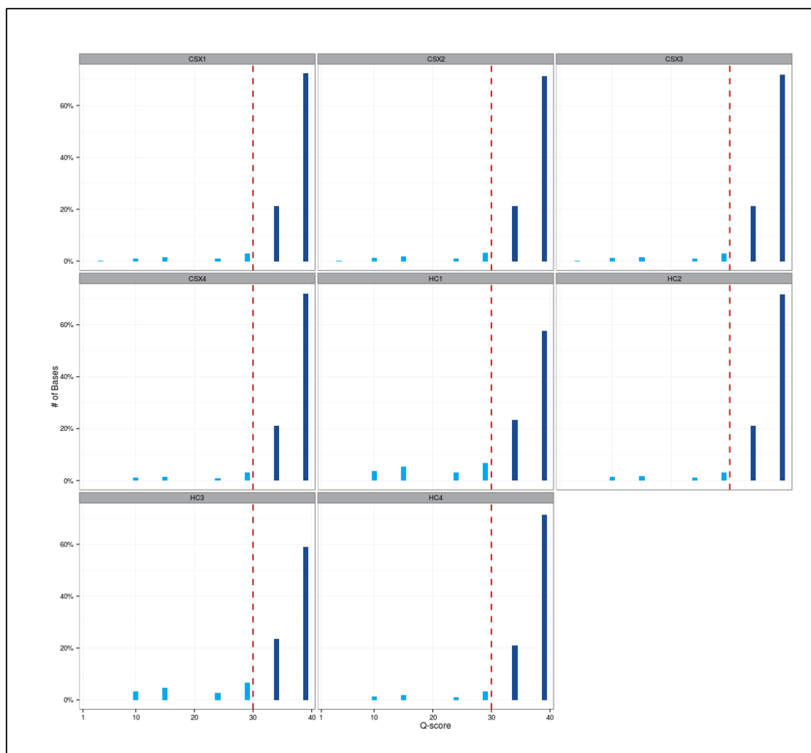
Figure 6.11: Q-scores of the various base samples in each subject. The vertical dotted lines delineate a Q-score of 30. The vast majority of data had a Q-score in excess of 30 indicating good quality data.
