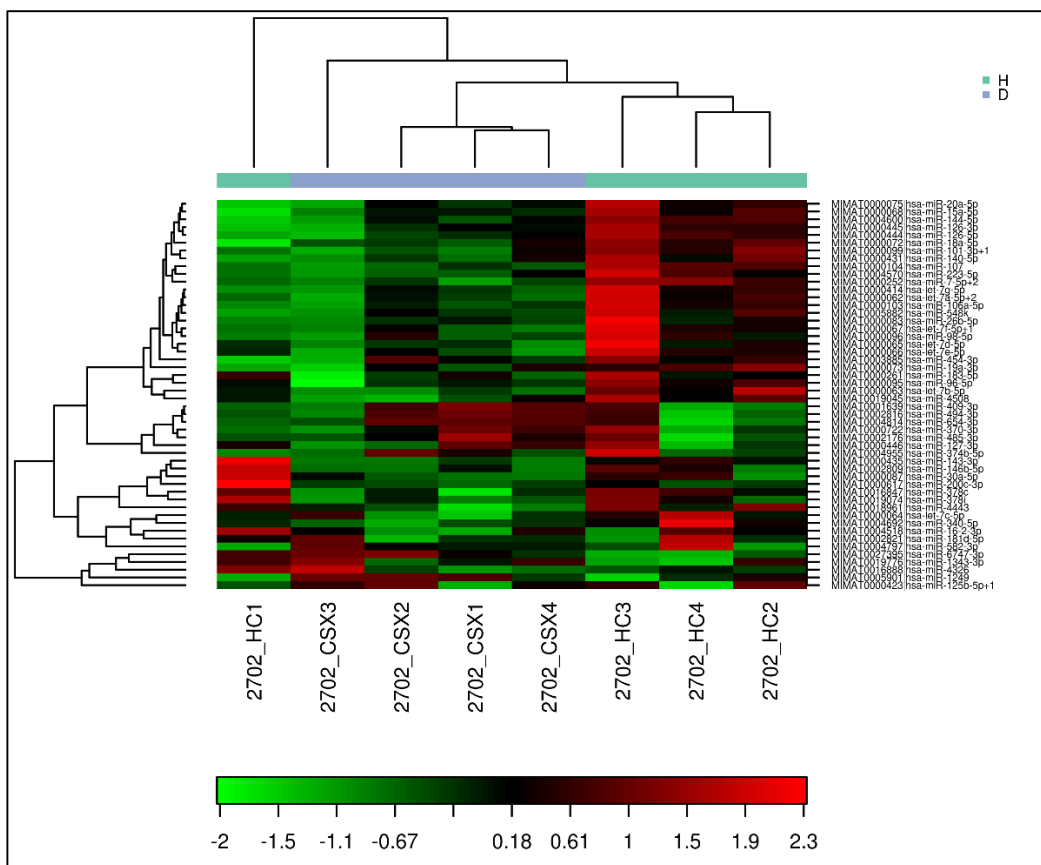
Figure 6.15: Heat Map and unsupervised hierarchical clustering by sample and microRNA. The clustering was performed on all samples, and on the top 50 microRNAs with highest %CV based on TPM normalized reads. There appears to be a clear differential expression of miRNAs between the CSX patients (2702_CSX1-4) and the control participants (2702_HC1-4).
