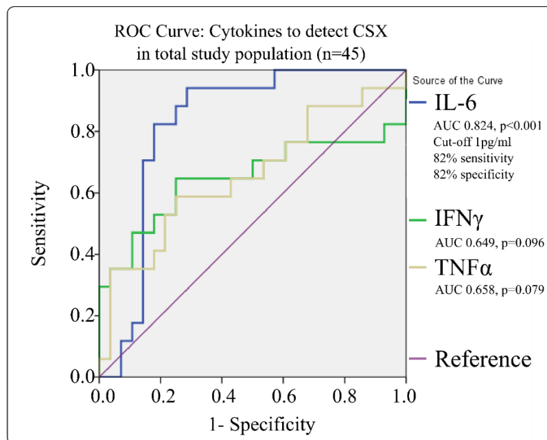
Figure 4.9: ROC curves for IL-6, IFN and TNF \alpha to identify CSX patients from overall study population.
