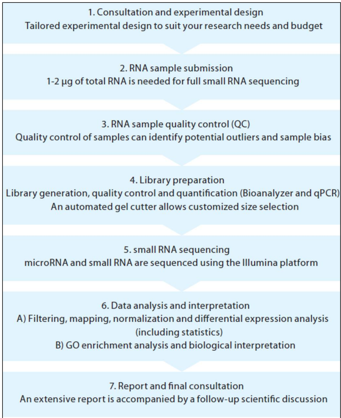
Figure 6.8: Work flow of Next-generation Sequencing by Exiqon Inc. (taken with permission from the Exiqon report)
