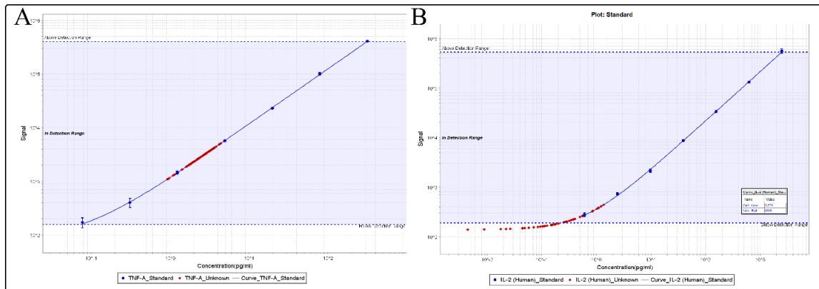
Figure 4.1: A. Plot showing the Standard Curve (blue) and sample signals (red dots) for TNF \alpha on the Pro-Inflammatory Plate. Note that all of the samples fall on the linear part of the calibration curve in the detection range. B. Similar plot for IL-2 on the TH1/TH2 Plate. Note that most samples fall below the LLOD or do not fall on the linear part of the standard curve.
