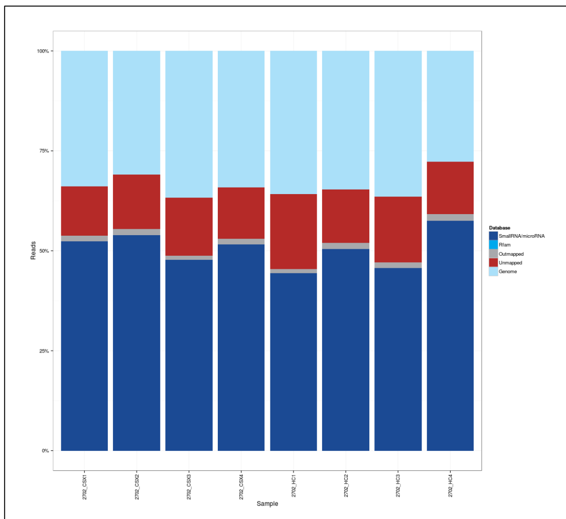
Figure 6.13 Mapping of NGS reads. Note the dark blue represents reads that map to miRNA's and accounts for approximately 50% of all reads.
