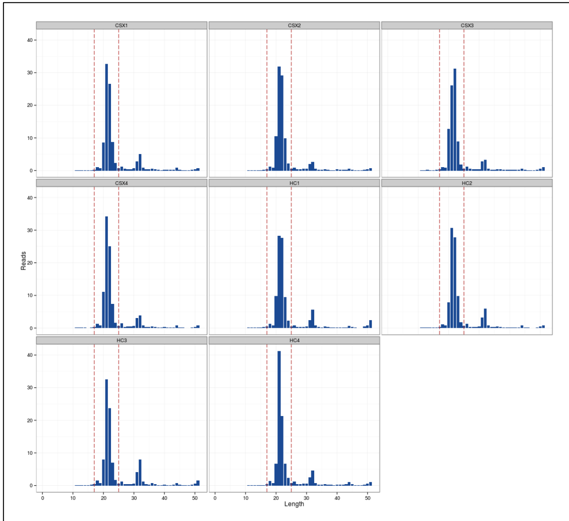
Figure 6.12 Read lengths. Note the spikes in the 18-22nt length, corresponding to detection of the miRNAs in the samples.
