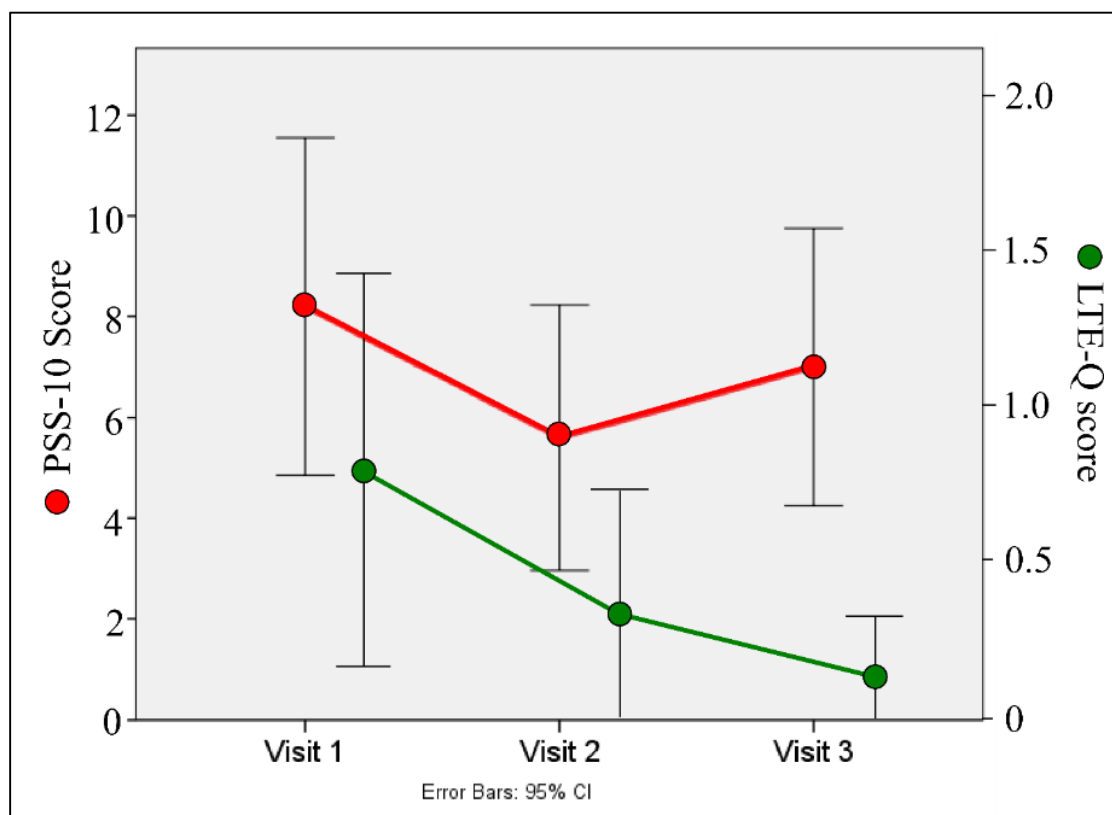
Figure 2.13 Mean PSS-10 and LTE-Q scores over the three visits.
