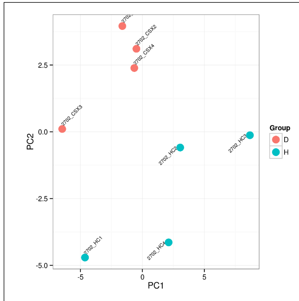
Figure 6.14: Principal Component Analysis plot with rescaling to be zero-centered and to have unit variance (i.e. the variance across samples is scaled to 1). D- Disease (CSX), H- Healthy. PC- Principal component.
