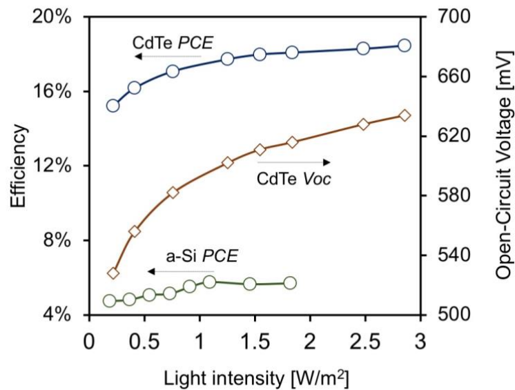
Figure 3: The CdTe PV cell efficiency and Open-Circuit Voltage under low intensity LED irradiance that is equivalent to ~200-2000 lux.
