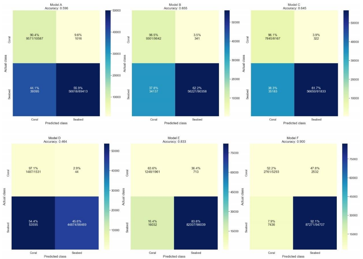
Figure 2.5: Confusion matrices representing the MGC classification results for each dense cloud reconstruction. Confusion matrices show the accuracy score and the relationship between the referenced data and the classification. The “Actual class” on the y-axis refers to the manually annotated data, whereas the “Predicted class” on the x-axis relates to the classification output. The main diagonal of the matrices lists the correctly classified percentage of points per class. The colour scale bar on the right of each confusion matrix represents the number of points.
