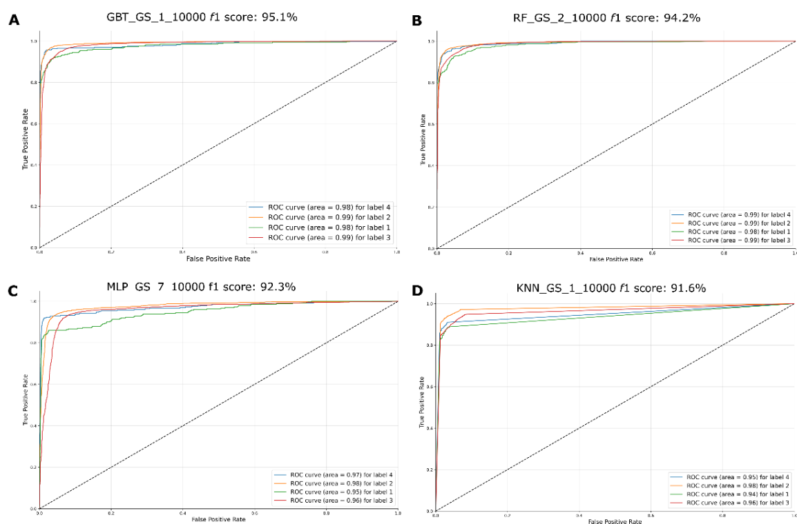
Figure 3.6: ROC curves of the four best-performing classifiers ( f1 > 90\% ). The name of the classifiers and their f1 score obtained on the first accuracy assessment were placed on the top of their respective graph. The AUC score for each label is placed on the lower right side of each graph. Label 1 = LCV, label 2 = SD, label 3 = DCF, label 4 = CR. (A) ROC curve of GBT classifier GBT_GS_1_10000, f1 score: 95.1% (B) ROC curve of the RF classifier RF_GS_2_10000, f1 score: 94.2% (C) ROC curve of the output of the MLP classifier MLP_GS_7_10000, f1 score: 92.3% (D) ROC curve of the KNN classifier KNN_GS_1_10000, f1 score: 91.6%.
