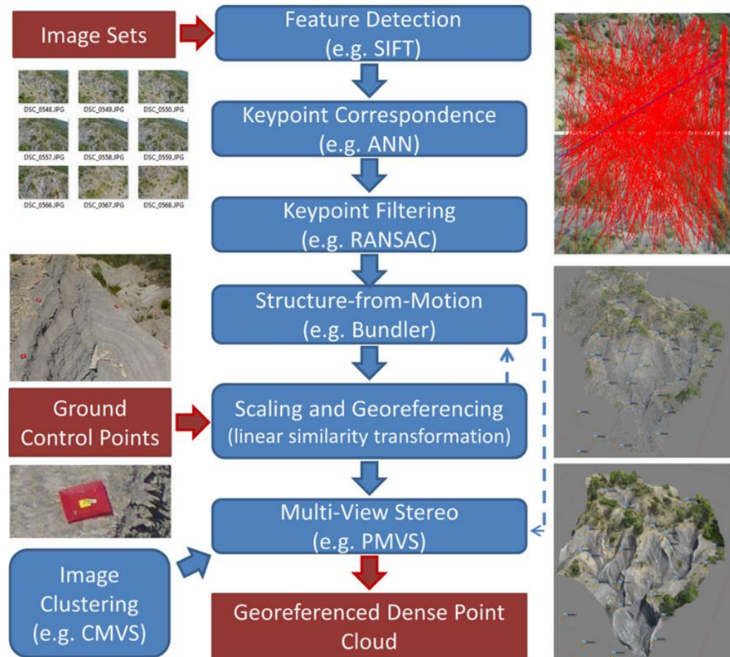
Figure 1.4: Standard Structure-from-Motion workflow for the production of georeferenced dense point clouds. Inputs and outputs are shown in red. From the top right to bottom right: valid image matches generated from key point correspondence, sparse point cloud, dense point cloud. Image extracted from Smith et al. (2016).
