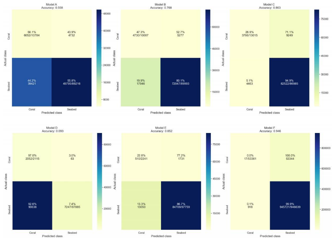
Figure 2.8: Confusion matrices representing the CGC classification results for each dense cloud reconstruction. The “Actual class” on the y-axis refers to the manually annotated data, whereas the “Predicted class” on the x-axis relates to the classification output. The main diagonal of the matrices lists the correctly classified percentage of points per class. The colour scale bar on the right of each confusion matrix represents the number of points.
