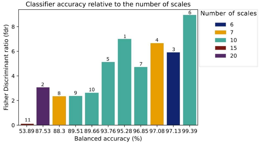
Figure 2.4: Classifier accuracy in relation to the number of scales. The classifier ID is placed on the top of each bar. In the MGC method, scale is defined as the neighbourhood size of pixels to which the classifiers compute each metrics.
