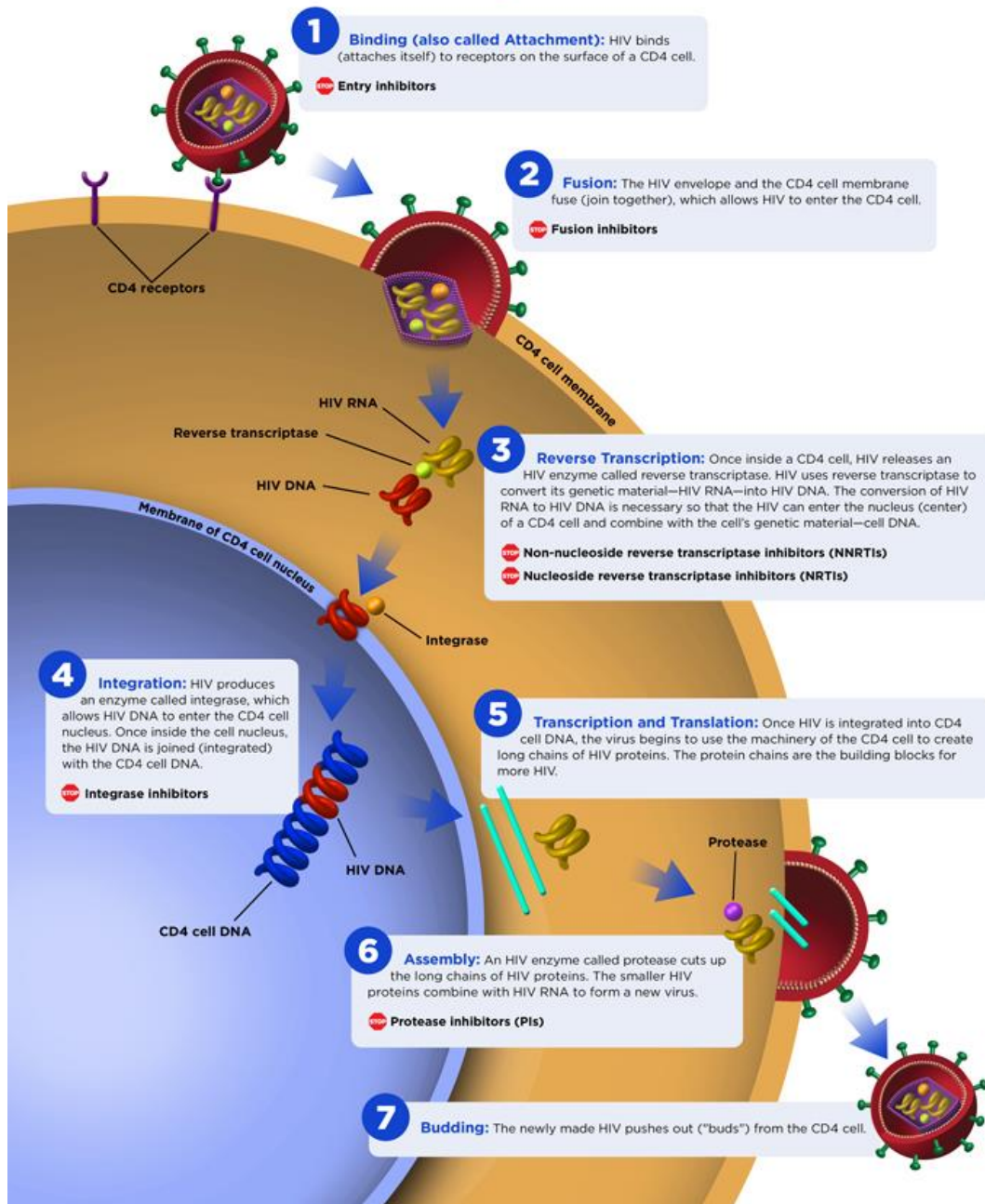
Figure 1-5. Life cycle of HIV virus and anti-retroviral treatment targets [43]
