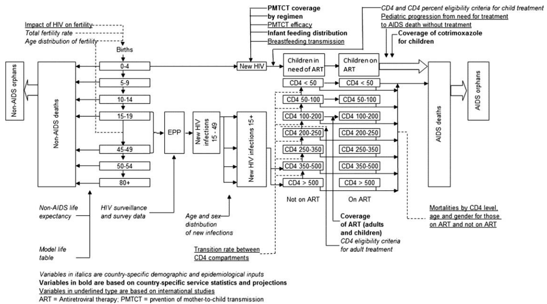
Figure 2-4. Diagram of Spectrum/Estimation and Projection Package (EPP) model [192].
