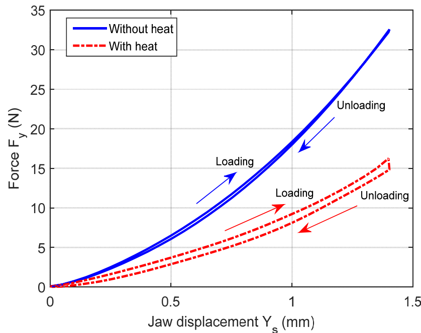
Figure 3. Testing results of the jaw mechanism with and without heat.
