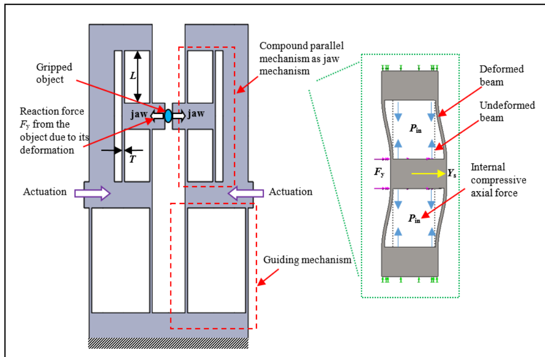
Figure 1. Schematic design of the proposed monolithic symmetrical gripper.
