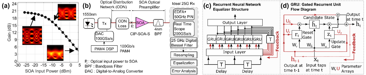
Fig. 1: (a) CIP-SOA-S gain curve with eye diagrams (inset) showing extent of inter-symbol interference (ISI), (b) experimental setup, (c) RNN equalizer structure with (d) Gated Recurrent Units making up recurrent hidden layer.
