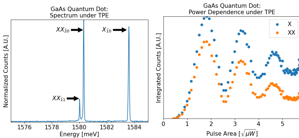
Figure 3.19: (Left) Typical GaAs QD spectrum under Two Photon Excitation (Right) Power dependence of 2X_{\bar{1}1} and X_{\bar{1}0} states under Two Photon Excitation, showing Rabi oscillations up to 7\pi .
