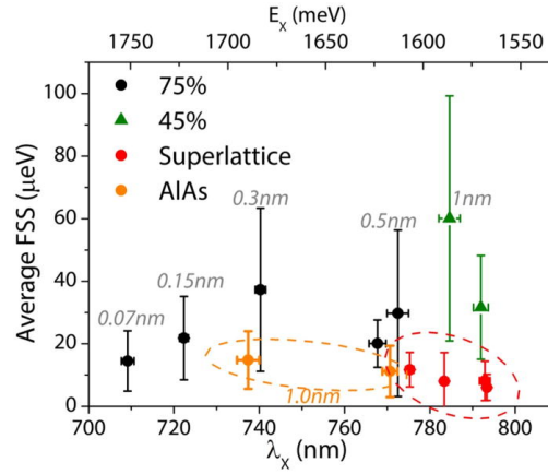
Figure 4.4: Average Fine Structure Splitting for different generations of QDs grown by the EPN group in Tyndall. In black (green) GaAs QDs with Al_{0.75}Ga_{0.25}As ( Al_{0.45}Ga_{0.55}As ) barriers, in orange GaAs QDs in AlAs barriers, and in red GaAs QDs in Al_{0.45}Ga_{0.55}As barriers with superlattice. The sample analysed in this thesis is among the ones of the most blueshifted data point of the superlattice series. Image taken from [1].
