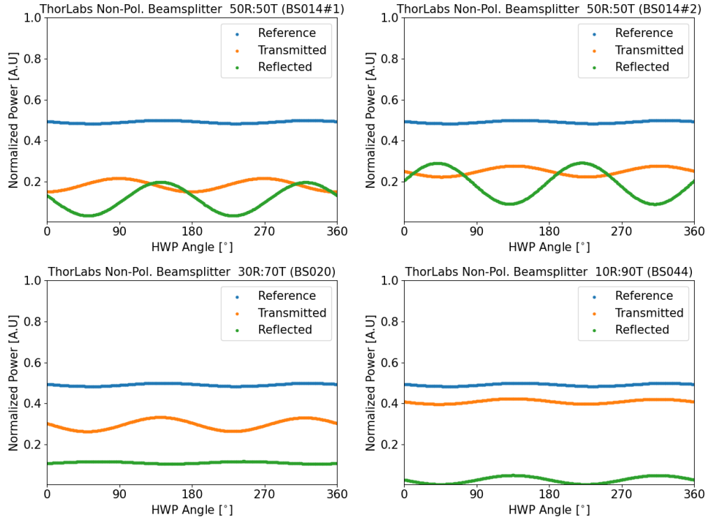
Figure 2.10: Characterization of four beam splitters available in the laboratory, 2 50R : 50T , 30R : 70T and 10R : 90T using circular polarized light as input and a rotating HWP and fixed polarizer as analyser.
