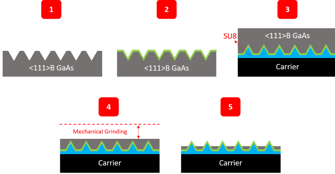
Figure 2.3: Backetch process, image taken from [8]. Steps: 1) Recesses are patterned on a (111)B GaAs substrate, 2) the QDs are grown inside the recesses in the MOVPE reactor, 3) as-grown sample is flipped and attached with SU8 to a (100) GaAs carrier, 4) excess substrate material is mechanically removed, down to a thickness of \sim 30\mu\text{m} , 5) the leftover substrate is removed using a chemical back-etching process until the pyramid's tips are exposed.
