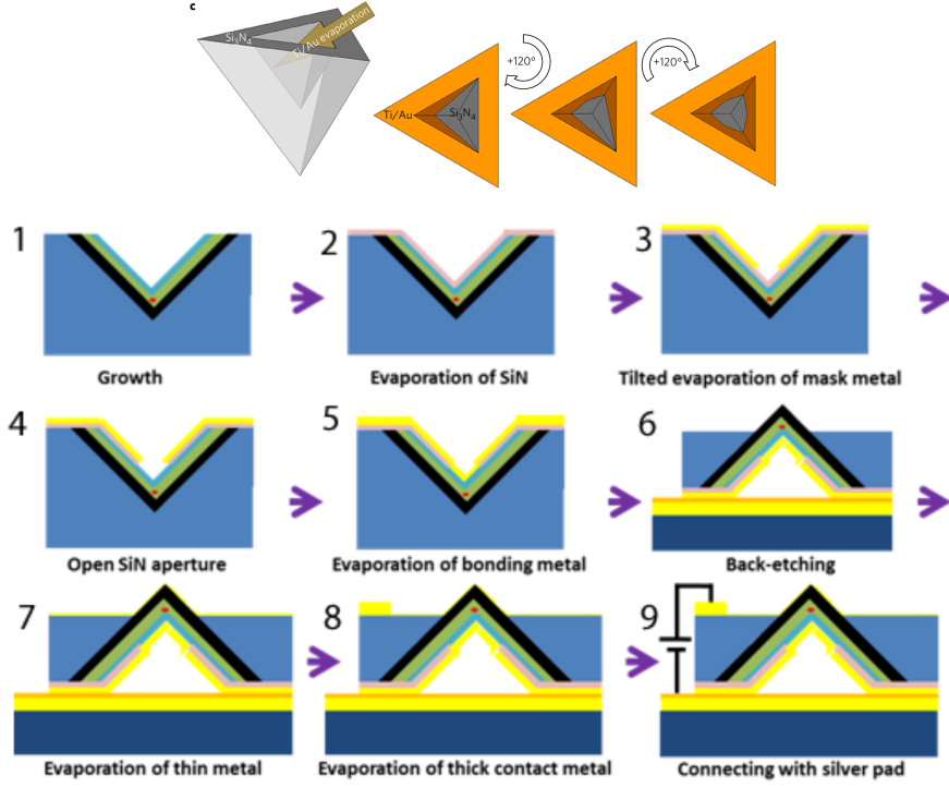
Figure 4.30: p-i-n diode structure for GaAs QDs: gold evaporation steps (top) full processing steps (bottom). Images taken from [18]
