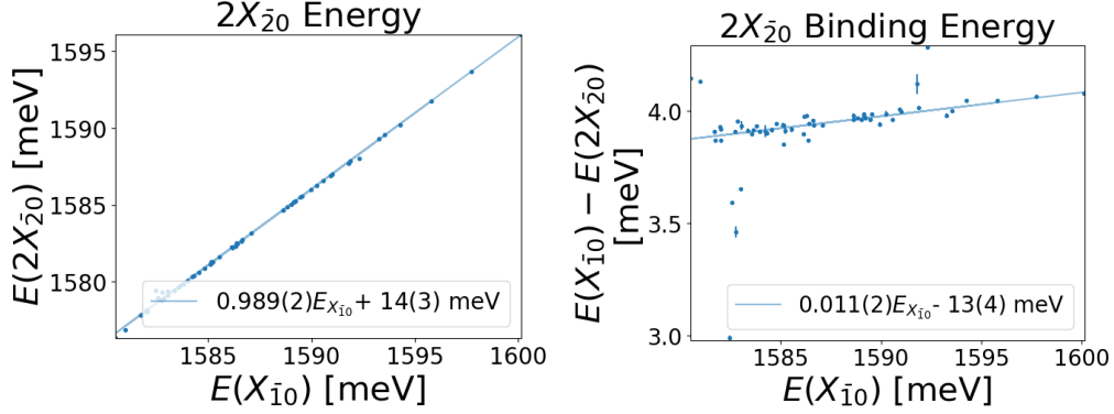
Figure 4.5: Energy of the biexciton (left) and the binding energy (right) of GaAs QDs as function of the X_{10} energy.
