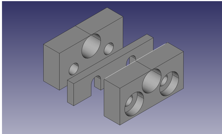
Figure 2.7: 3D model of the custom built magnet holder. The cylindrical magnets, of 3\text{mm} radius, are inserted in the two round holes at the center of the left and right pieces. The magnets holder are 10\text{mm} tall, 5\text{mm} wide and 20\text{mm} long. The sample, up to 2\text{mm} in length, is attached in the central part. The whole unit is kept together by M3 bolts.
