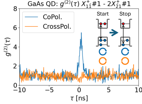
Figure 4.24: g^{(2)}(\tau) : recombination cascade 2X_{21}^+ \rightarrow X_{11}^+ .
