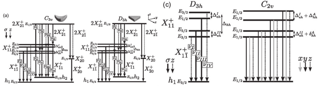
Figure 1.14: Recombination cascade of 2X_{21}^+ (left side) and 2X_{11}^+ (right side) with symmetries C_{3v} , D_{3h} and C_{2v} . Taken from [36]
