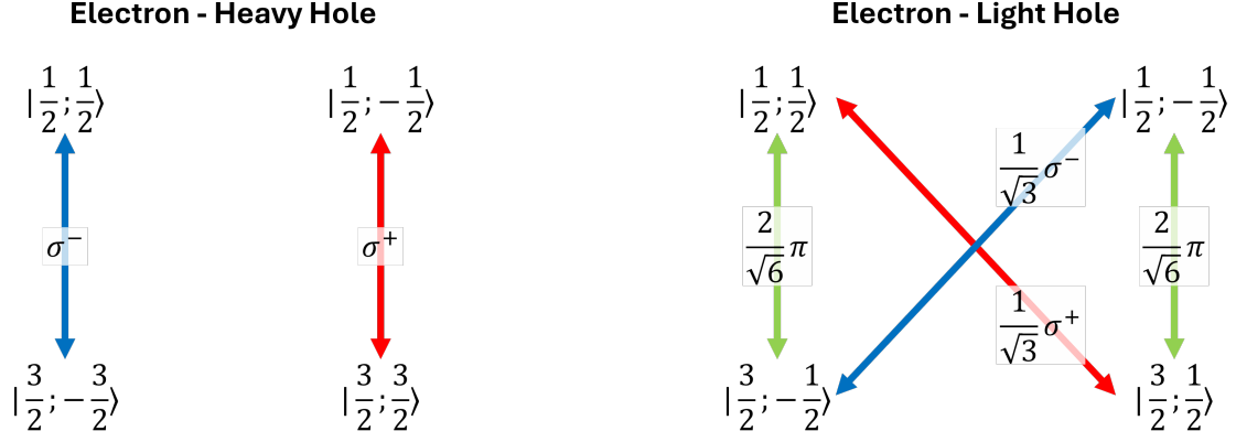
Figure 1.9: Selection rules for electron - hole recombination from different bands.
