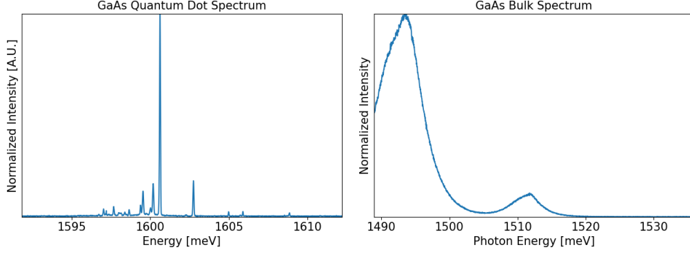
Figure 3.1: (Left) Typical spectrum of a GaAs QD in AlGaAs barrier (Right) Typical spectrum of GaAs bulk left from the backetching process
