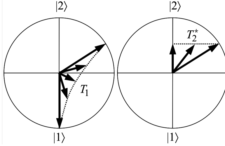
Figure 1.6: Decoherence processes visualized on a Bloch Sphere. Left, a longitudinal relaxation process. Right, a pure dephasing process. Picture adapted from [8]
