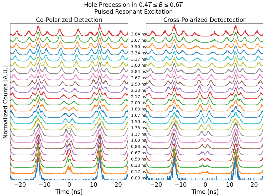
Figure 5.20: Hole precession in phonon-assisted (left) and resonant (right) excitation for variable delays.
