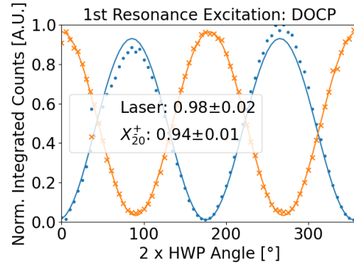
Figure 5.5: Degree of Polarization of laser and X_{20}^+ state under resonant excitation with circularly polarized light at the 1 st resonance.
