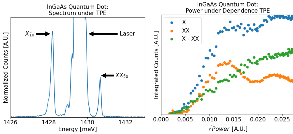
Figure 3.21: (Left) Typical InGaAs QD spectrum under Two Photon Excitation (Right) Power dependence of 2X_{20} and X_{10} states under Two Photon Excitation, showing the phonon assisted component in the emission of the X.
