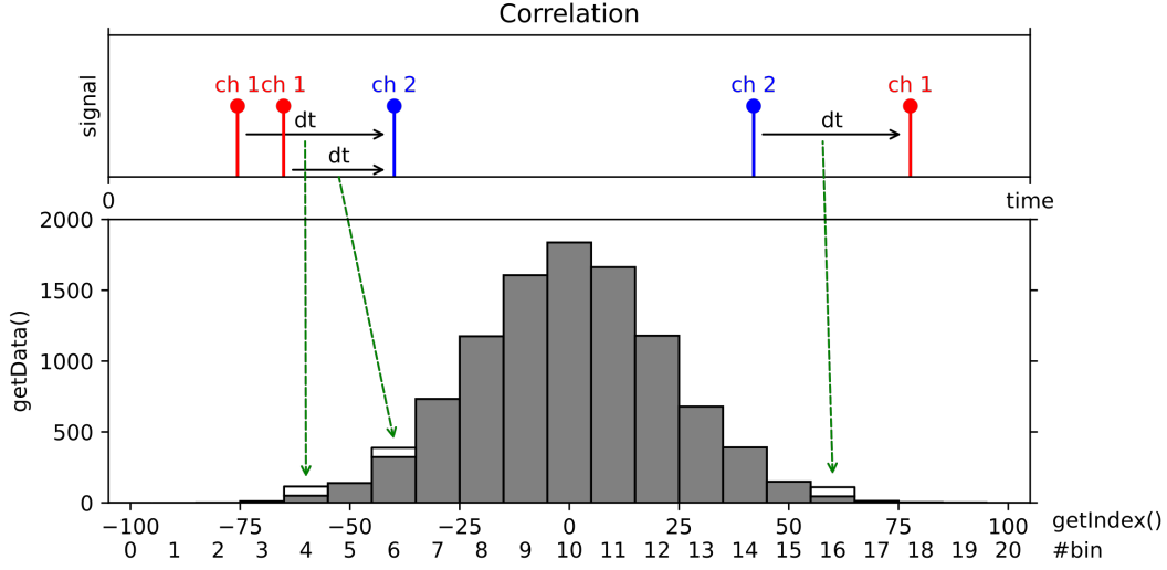
Figure 2.12: Correlation measurement in the Swabian TimeTagger Ultra TCSPC module. Image taken from [15]
