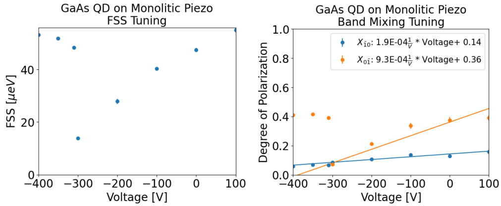
Figure 4.16: Tuning of Fine Structure Splitting (left) and of band mixing (right) as function of the voltage applied to the piezoelectric substrate.
