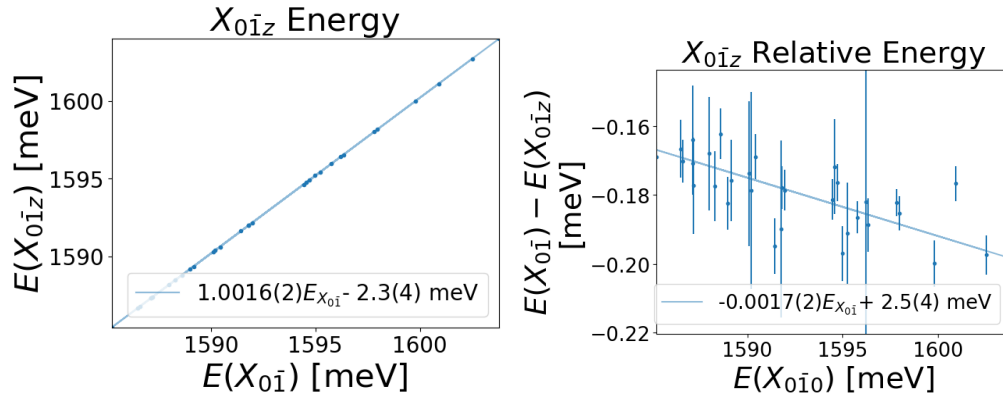
Figure 4.10: Energy of the non-degenerate excited exciton (left) and energy difference with excited exciton (right) of GaAs QDs as function of the X_{0\bar{1}} energy.
