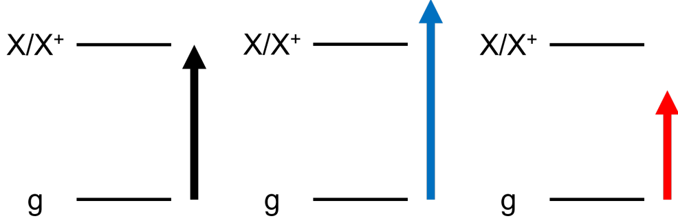
Figure 3.3: Two-Levels System and Laser. (a) Resonant, (b) Blue-Detuned, (c) Red-Detuned
