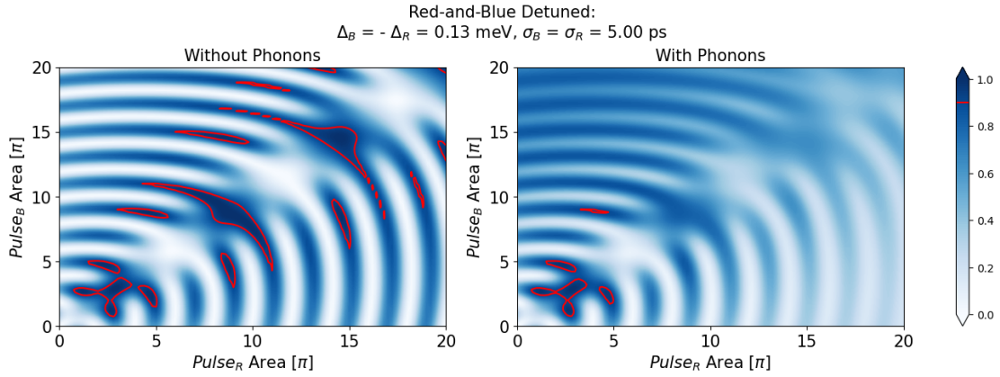
Figure 3.28: Red-and-Blue excitation for \eta = 1
