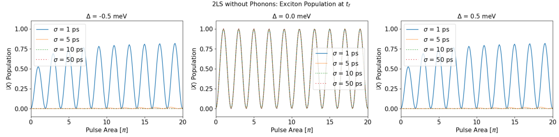
Figure 3.10: Excited State population after a Gaussian Pulse for a 2LS without Phonons, at different pulse length and detuning
