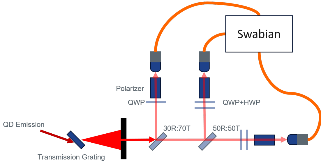
Figure 2.14: Transmission grating spectrometer and three photon correlation setup
