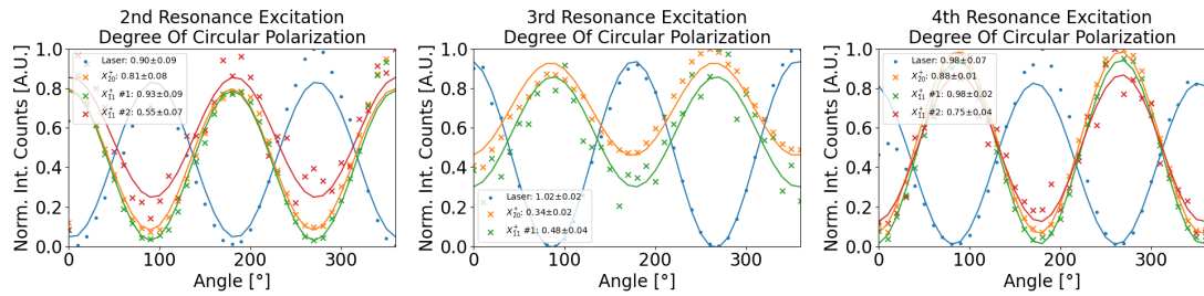
Figure 5.9: Degree of Polarization of laser and trion states under resonant excitation with circularly polarized light at the 2 nd , 3 rd and 4 th resonance.
