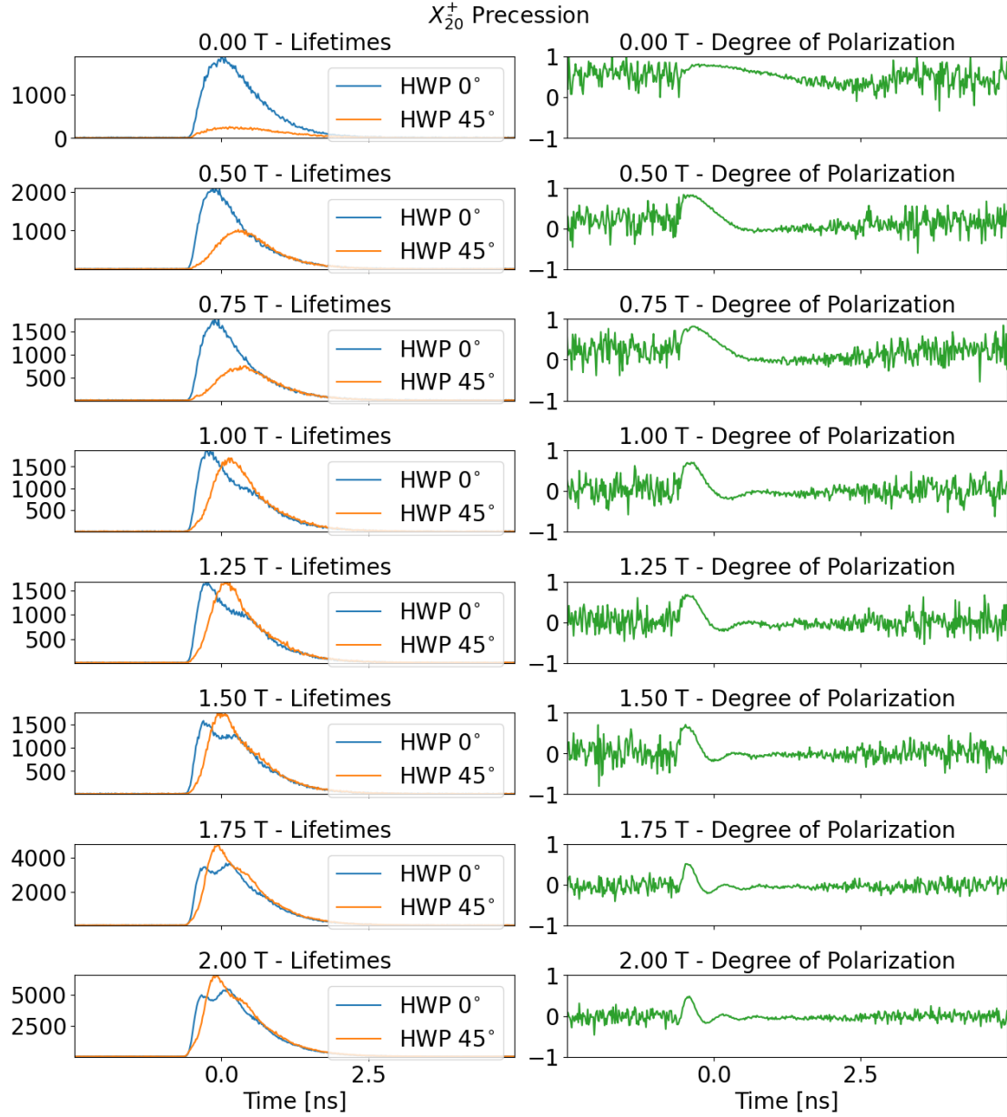
Figure 5.15: Precession of Trion in a strong magnetic field.
