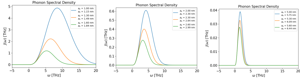
Figure 3.4: Phonon coupling for dots of different size ( a_e = [1, 2, 5]nm )
