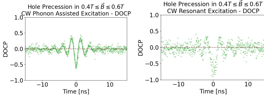
Figure 5.18: Hole precession in phonon-assisted (left) and resonant (right) excitation.
