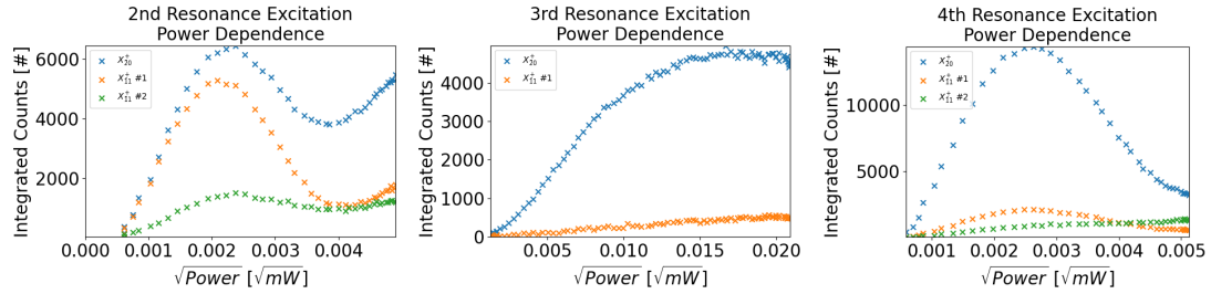
Figure 5.8: Power Dependence the trion states under resonant excitation at the 2 nd , 3 rd and 4 th resonance.
