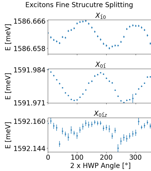
Figure 4.7: Energy of the X_{10} (top), the X_{01} (middle) and the X_{01z} (bottom) states as function of HWP angle.
