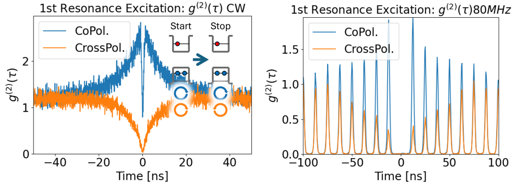
Figure 5.6: g^{(2)}(\tau) of X_{20}^+ state under resonant excitation with linearly polarized light, in CW excitation (left) and pulsed at 80 MHz (right).
