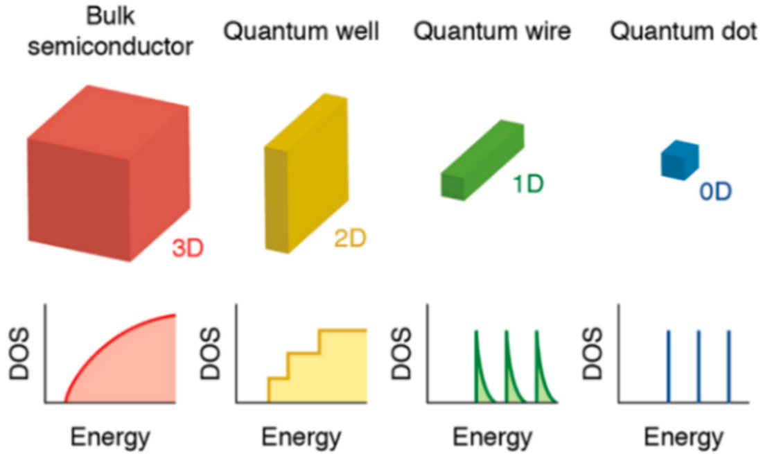
Figure 1.7: Confinement and density of states for different semiconductor structures. Taken from [31]
