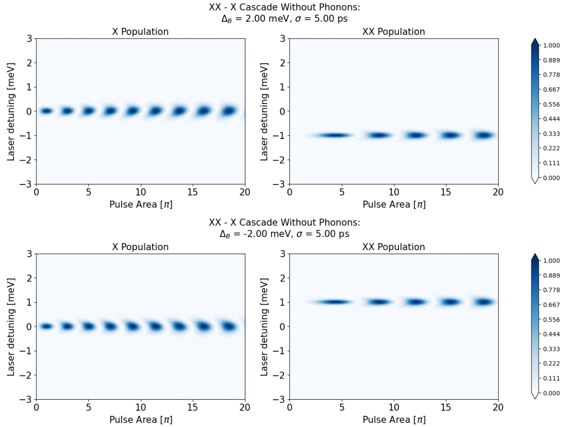
Figure 3.16: |XX\rangle and |X\rangle Population after a Gaussian pulse as function of pulse area and detuning for a cascade, binding (upper half) and antibinding (lower half), without Phonon interaction. Due to the lack of a decay operator for the 2X_{\bar{2}0} \rightarrow X_{\bar{1}0} cascade the X_{\bar{1}0} is populated only when the pulse is on resonance with the transition, \Delta = 0 \text{ meV} . If a decay operator was introduced in the simulation the X_{\bar{1}0} population would should a second resonance that maps the 2X_{\bar{2}0} population when the pulse detuning is at TPE condition, \Delta = \pm 1 \text{ meV} .
