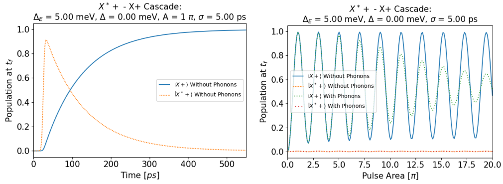
Figure 3.24: Time evolution of the |X_{11}^+\rangle and |X_{20}^+\rangle Populations during a Gaussian pulse and decay, final states population as function of pulse area for a cascade
