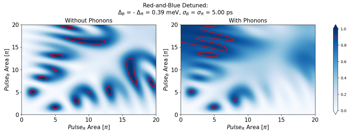
Figure 3.29: Red-and-Blue excitation for \eta = 3
