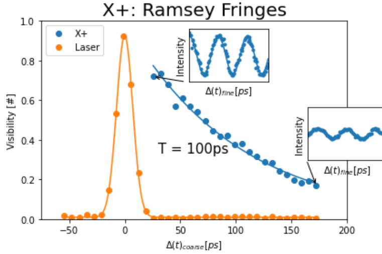
Figure 3.26: Ramsey fringes visibility for laser and X_{20}^+ state as function of the coarse delay
