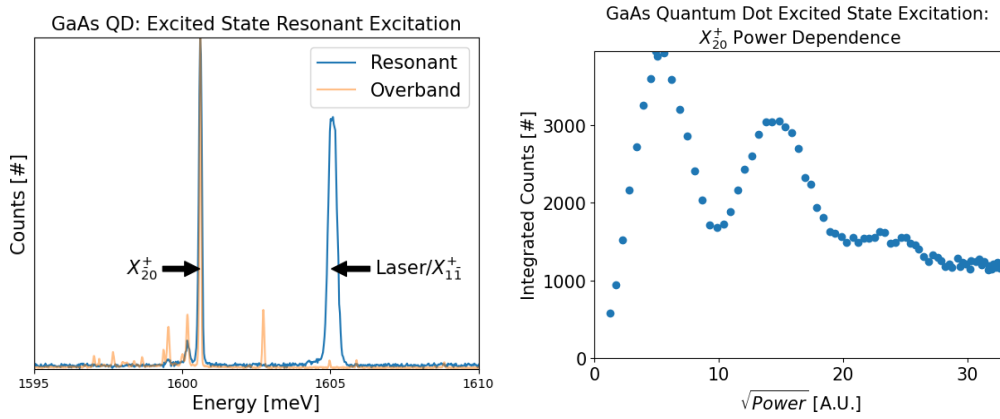
Figure 3.25: Spectrum and power dependence of trion population under resonant excitation of one of its excited states.
