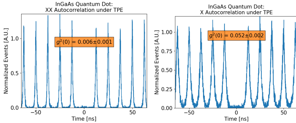
Figure 3.22: Autocorrelation measurement of the 2X_{20} and X_{10} transitions under Two Photon Excitation highlighting single photon emission.
