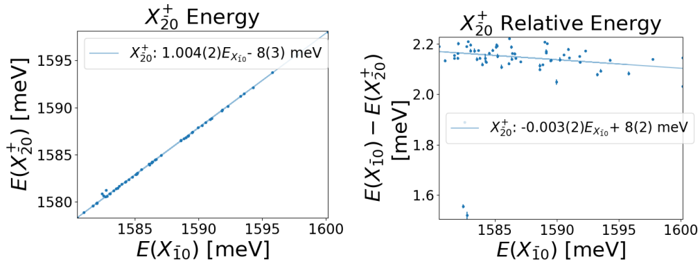
Figure 4.18: Energy (left) and relative energy (right) of the ground trion state as function of the X_{10} energy.
