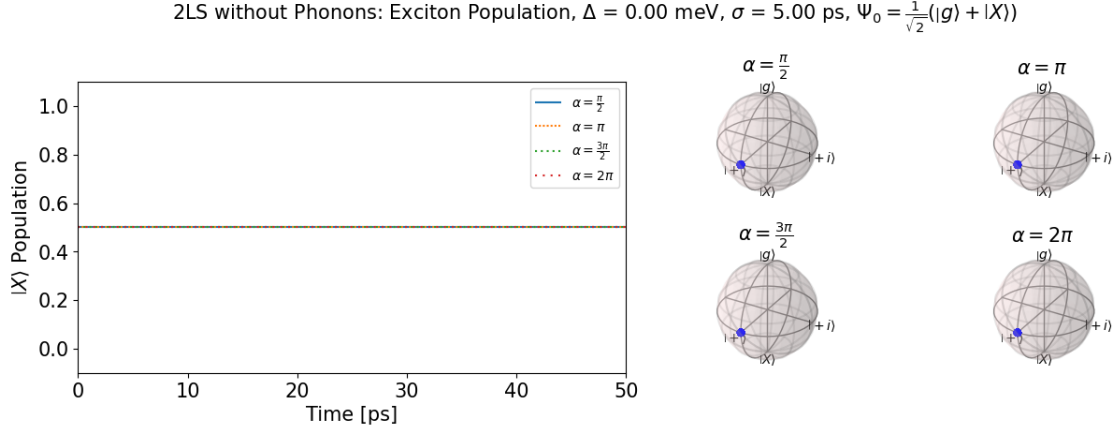
Figure 3.8: 2LS without phonons excited by a Gaussian pulse of different pulse areas ( \Psi_0 = \frac{1}{\sqrt{2}}(|g\rangle + |X\rangle) ): time dynamics and evolution on Bloch Sphere
