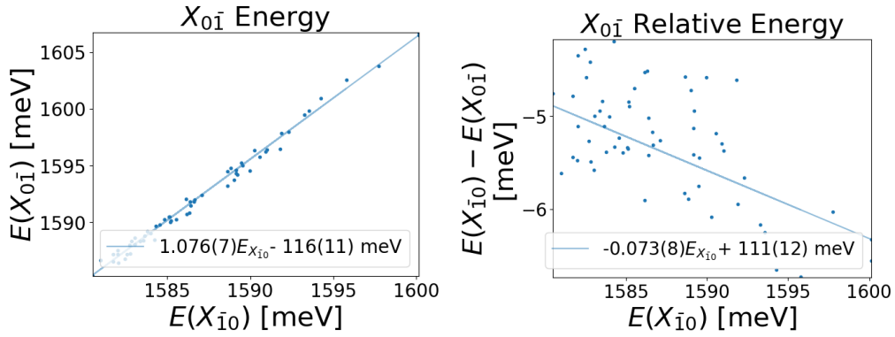
Figure 4.9: Energy of the excited exciton (left) and energy difference with ground exciton (right) of GaAs QDs as function of the X_{10} energy.
