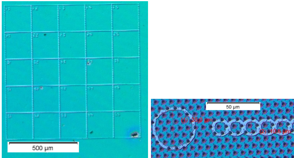
Figure 2.5: Test patterns written with the scratch built lithography setup. The scale bars for reference are (left) 500\mu m , (right) 50\mu m .
