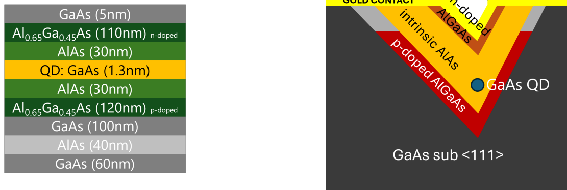
Figure 4.29: p-i-n diode structure for GaAs QDs: epitaxial structure (left) sketch showing the non planar geometry of the sample which would cause the short circuit condition if a gold contact was directly evaporated on top without the trenches (right)
