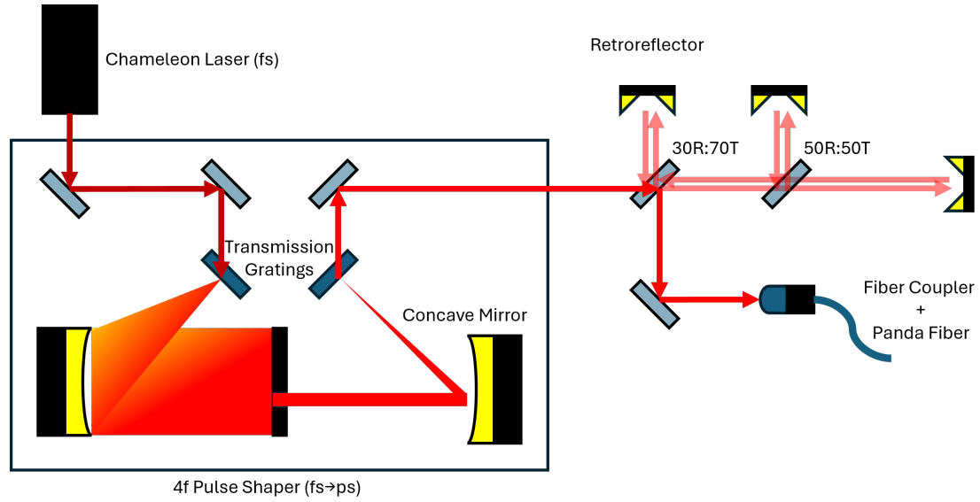
Figure 2.13: Laser multiplexing setup to generate time-tuned pulses.
