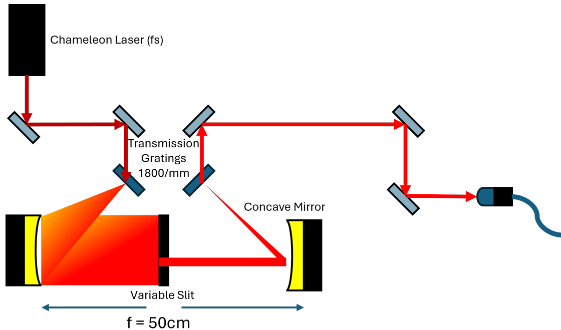
Figure 2.8: 4f Pulse Shaper to convert a fs pulse to ps
