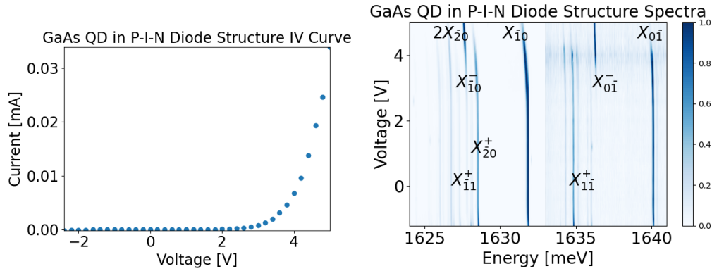
Figure 4.31: p-i-n diode structure for GaAs QDs: measured IV curve showing the expected diode behaviour (left) PL spectra as function of the applied voltage showing very weak Stark shift and charge tuning under forward bias, the spectra has been divided in two ranges, ground and excited states, and each range normalized to highlight the relative intensity of the states (right).
