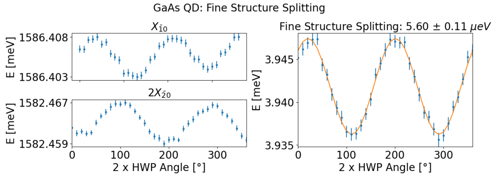
Figure 4.2: Energy of X_{\bar{1}0} (top left) and 2X_{\bar{2}0} (bottom left) states as function of HWP angle and Fine Structure Splitting of a GaAs QD (right)
