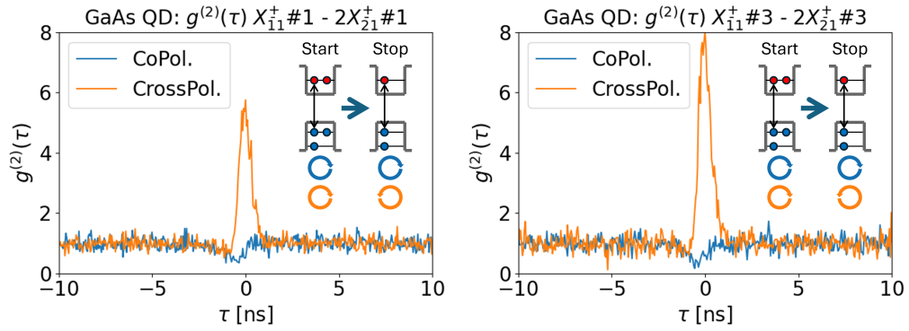
Figure 4.23: g^{(2)}(\tau) : recombination cascade 2X_{21}^+ \rightarrow X_{11}^+ .
