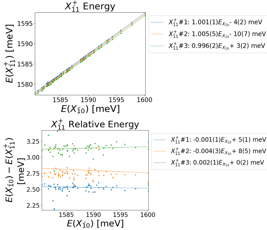
Figure 4.19: Energy (top) and relative energy (bottom) of trions in which the heavy-hole recombines with the electron.
