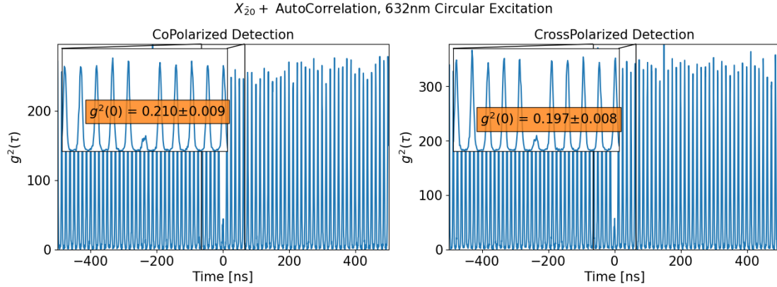
Figure 3.2: Autocorrelation curves of the X_{20}^+ peak under above-band circular excitation
