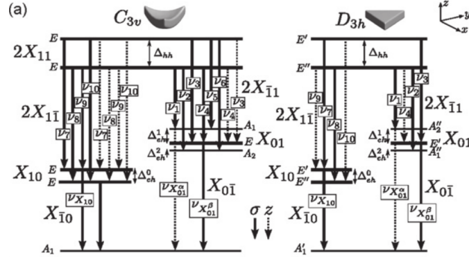
Figure 1.12: Decay of 2X_{11} and 2X_{1\bar{1}} with symmetries C_{3v} and D_{3h} . Taken from [36]
