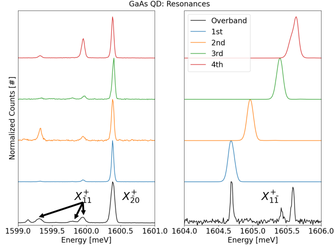
Figure 5.3: Spectrum of a GaAs QD under resonant excitation of the 4 resonances of trion states.
