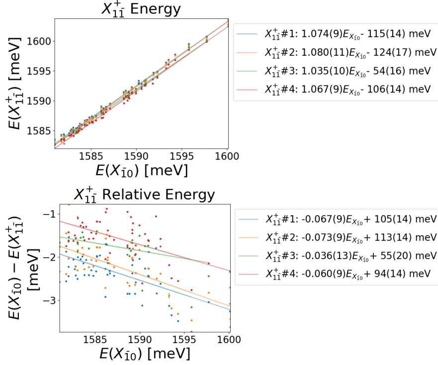
Figure 4.20: Energy (top) and relative energy (bottom) of trions in which the light-hole recombines with the electron.
