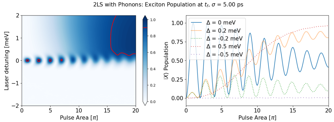
Figure 3.11: Exciton Population after a Gaussian pulse as function of pulse area and detuning for a 2LS with Phonon interaction
