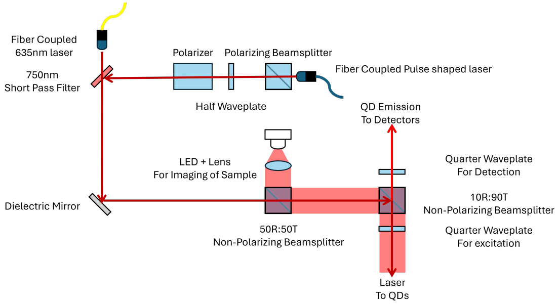
Figure 2.11: Beam path of lasers and imaging system. If the QWP for excitation is inserted, the QWP for detection is removed.
