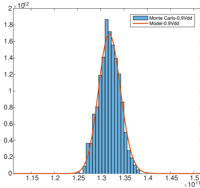
(c) V_{dd} = 0.9 \text{ V}
