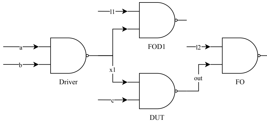
Figure 4.24: The simulated NAND-chain circuit
