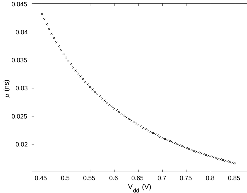
(a) \mu vs. V_{dd}
