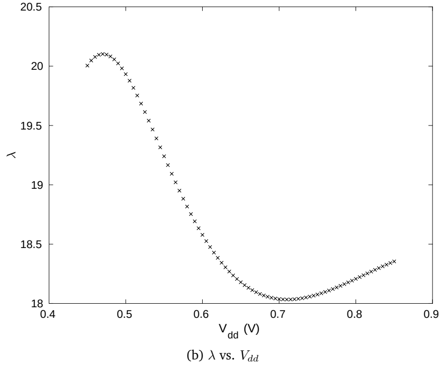
Figure 4.20: Function of \mu and \lambda against V_{dd}
