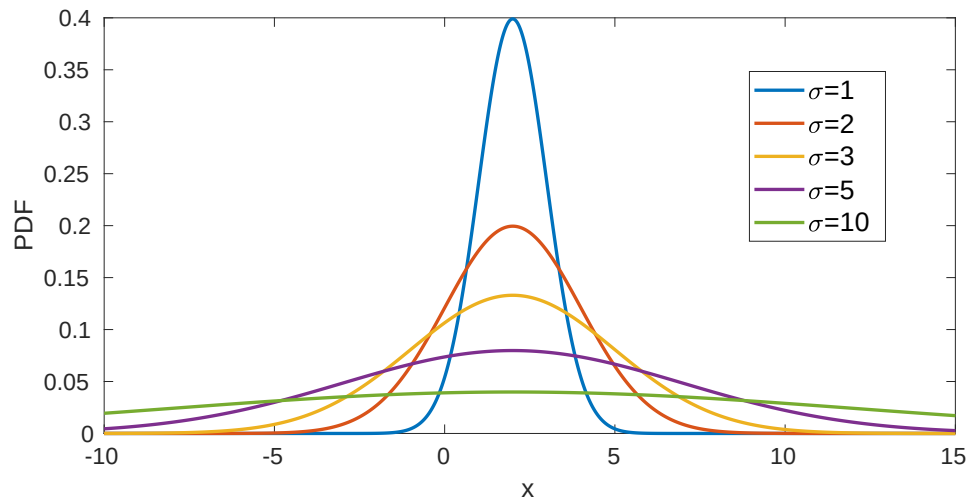
Figure 2.4: GD curves with \mu = 2 and different \sigma
