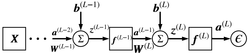
Figure A.1: Compact ANN model for BP demonstration
