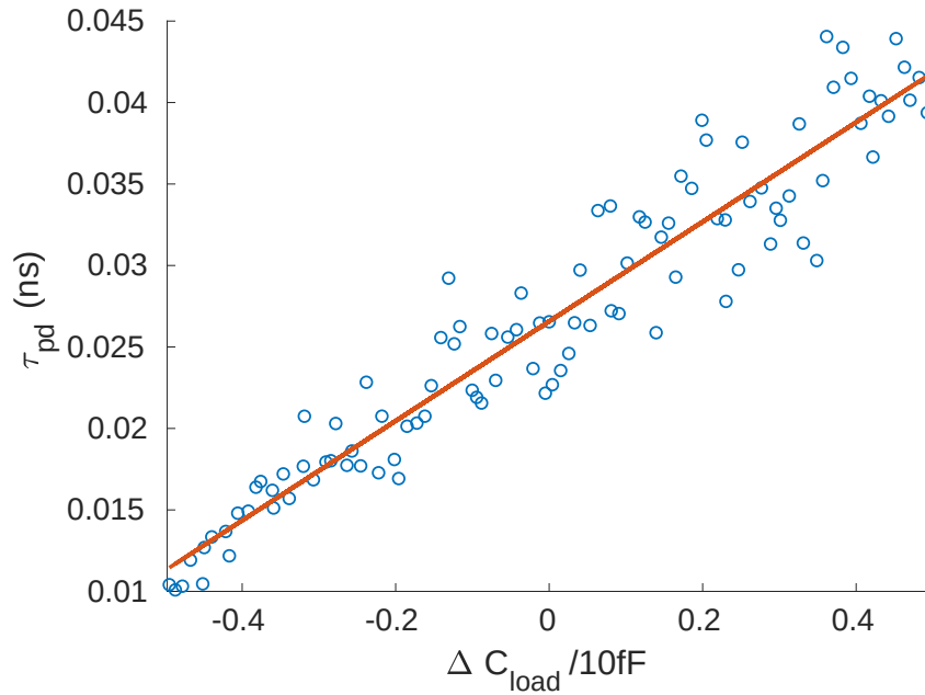
Figure 2.7: Scatter plot of \tau_{\text{pd}} against C_{\text{load}} demonstrating a linear correlation
