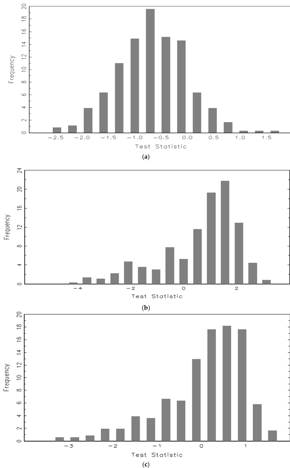
Figure 1. Distribution of the Unconditional Market-Timing Test Statistic. (a) Test Statistic of Unconditional Nonparametric Market Timing; (b) Test Statistic of Unconditional TM Market Timing; (c) Test Statistic of Unconditional HM Market Timing.
