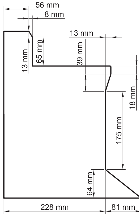
Figure 4: Cross-section of the Dawlish seawall at a 1:20 scale.
