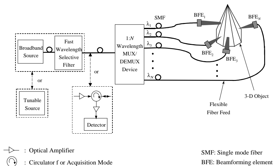
Fig. 5 Basic structure of our fiber-remoted W-MOS.
