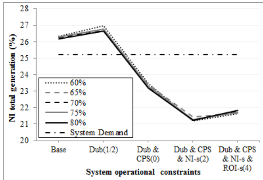
Figure 7.8: Total NI generation as a percentage of total AI generation for at different SNSP percentage limits and minimum number of large conventional generators on-line constraints relaxed in cumulative combination from left to right
