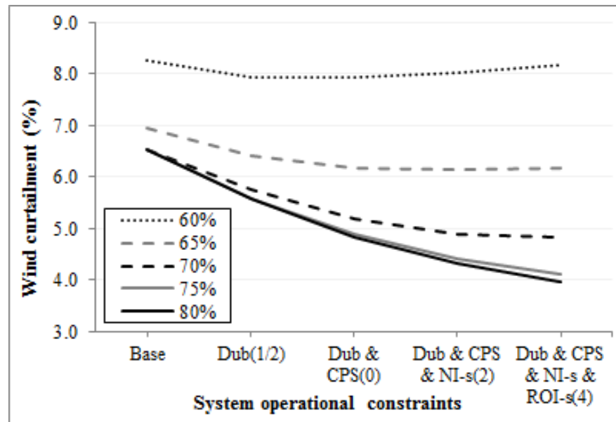
Figure 7.5: The percentage of wind curtailment for AI at different SNSP percentage limits and minimum number of large conventional generator on-line constraints relaxed in cumulative combination from left to right
