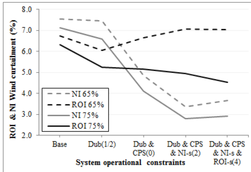
Figure 7.6: The percentage of wind curtailment in NI and ROI at 65% and 75% SNSP percentage limits and minimum number of large conventional generators on-line constraints relaxed in cumulative combination from left to right
