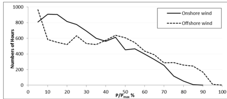
Figure 5.3: Wind generation duration curves for aggregated onshore and offshore power, net of curtailment, with a SNSP limit of 70%.
