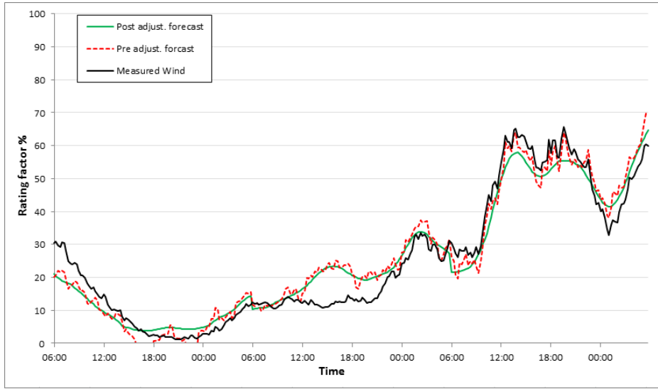
Figure 4.8: Wind forecast adjustment for the 6% MAE scenario and measured wind profile for the 21 st to 23 rd February of the test year.
