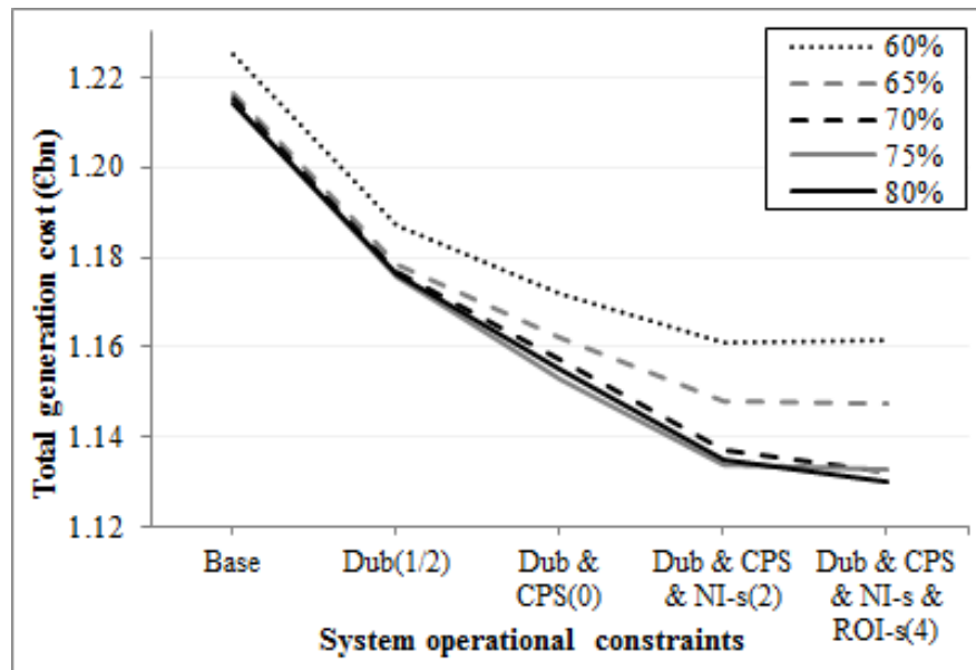
Figure 7.4: Total AI generation costs (€m) at different SNSP percentage limits and minimum number of large conventional generator on-line constraints relaxed in cumulative combination from left to right
