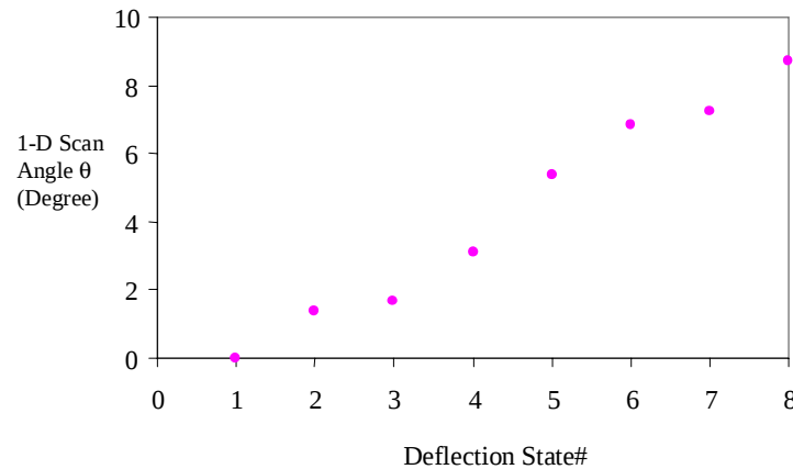
Fig. 3: Designed deflection angles for a 3-stage coarse 1-D P-MOS scanner. \alpha_1=4.95^\circ , \alpha_2=14.95^\circ and \alpha_3=-4.95^\circ using Rutile ( n_e=2.454 , n_o=2.71 @ \lambda=1529.6 nm).
