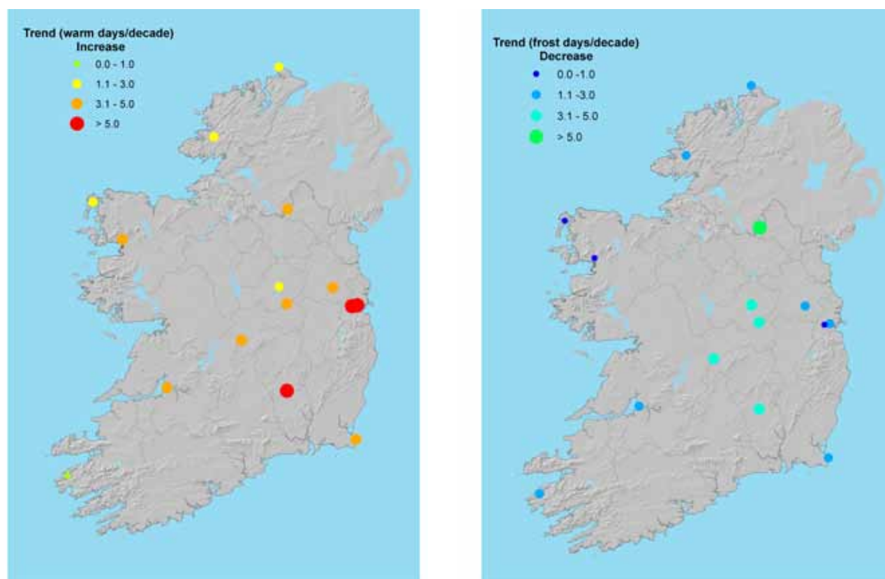
Figure 2.3. Trend in number of warm days per decade 4 (left) and number of frost days per decade 4 (right) (1961–2010).
