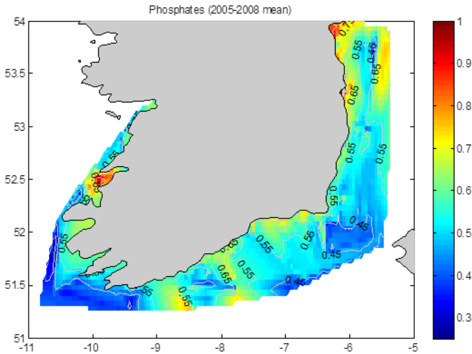
Figure 3.17. Mean surface phosphate concentrations ( \mu\text{M} ), 2005–2008.
