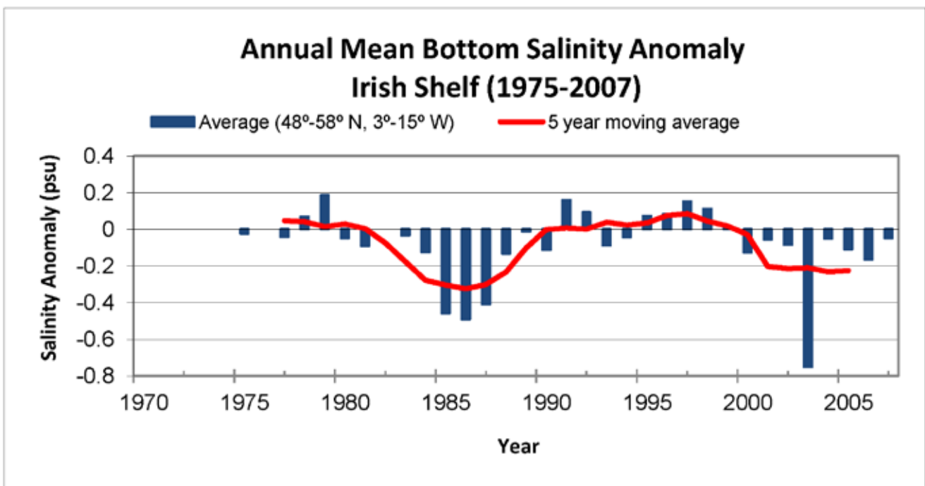
Figure 3.4. Annual mean salinity anomalies on Irish shelf (1975–2007).
