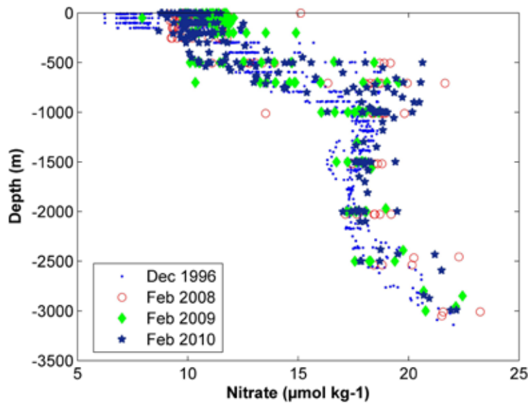
Figure 3.18. Sub-surface nitrate concentrations ((mM) from WOCE (1996) and more recent surveys in the Rockall Trough.
