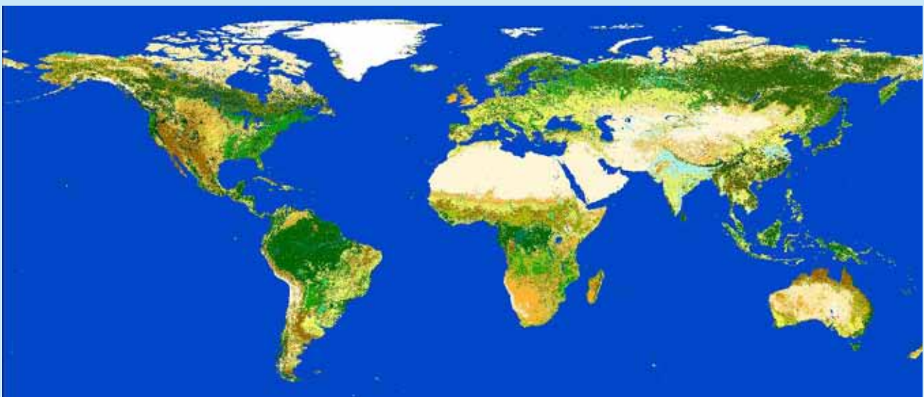
Figure SB7.1. Global land cover derived from data collected in 2009 from Envisat's Medium Resolution Imaging Spectrometer (MERIS) instrument. © ESA and UCLouvain.
