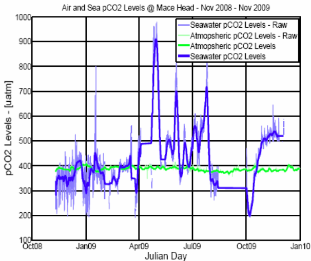
Figure 3.7. Variability in water \text{CO}_2 concentration ( \text{pCO}_2 ), November 2008–November 2009, as measured at a buoy near Mace Head (blue). Atmospheric \text{CO}_2 concentration is also shown (green).
