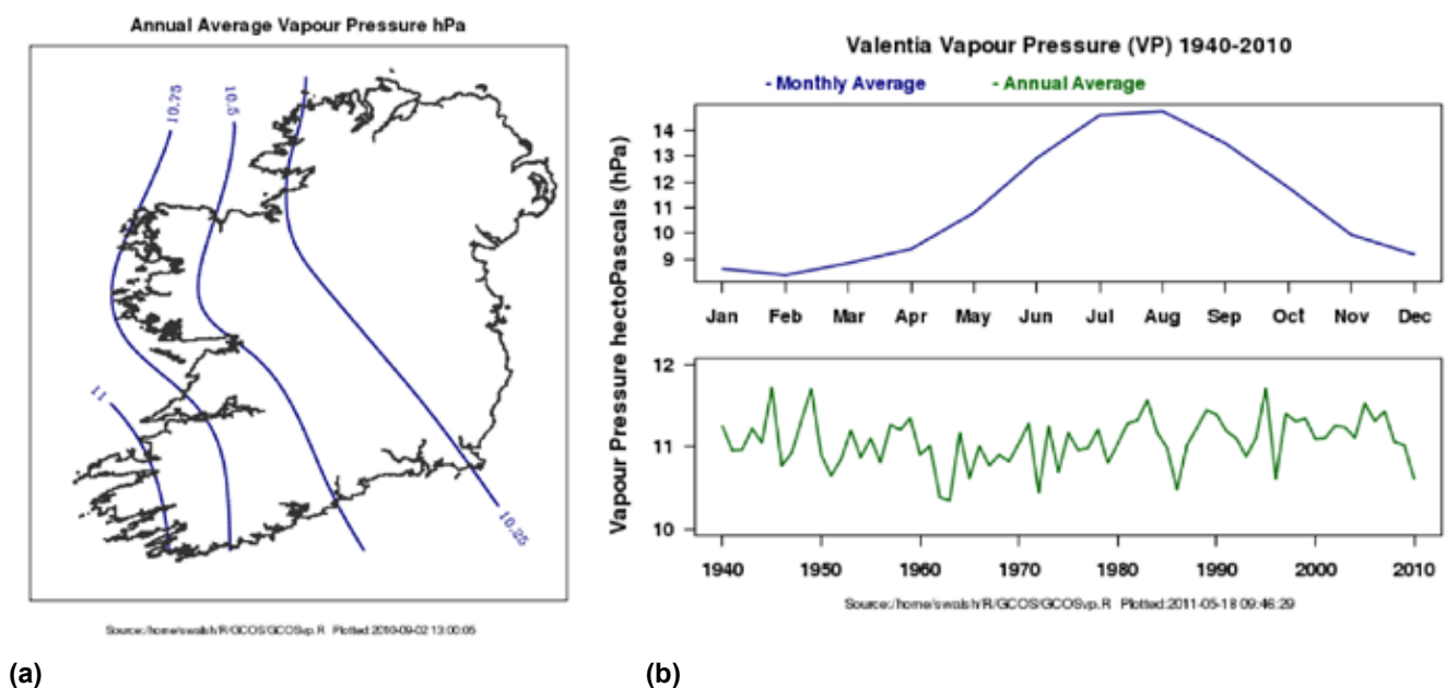
Figure 2.9. Annual average water vapour pressure across Ireland (a) and monthly and annual average water vapour pressure at Valentia Observatory (b) (1940–2010).
