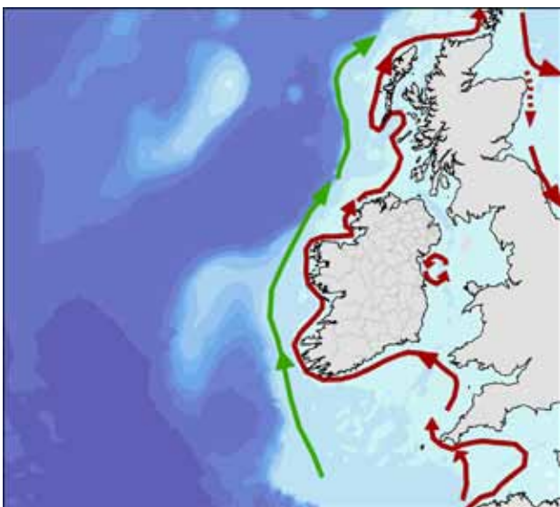
Figure 3.13. Main ocean current pathways around Ireland.
