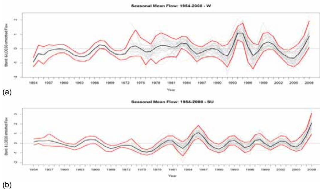
Figure 4.17. Seasonal mean flows for winter (a) and summer (b) from river flow meters in the reference network (1954–2008).
