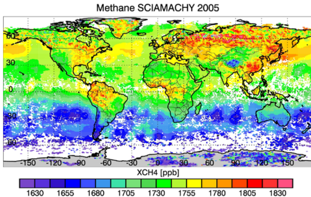
Figure 2.18. Example of annual global mean methane concentration for 2005 as derived from satellite observations.
