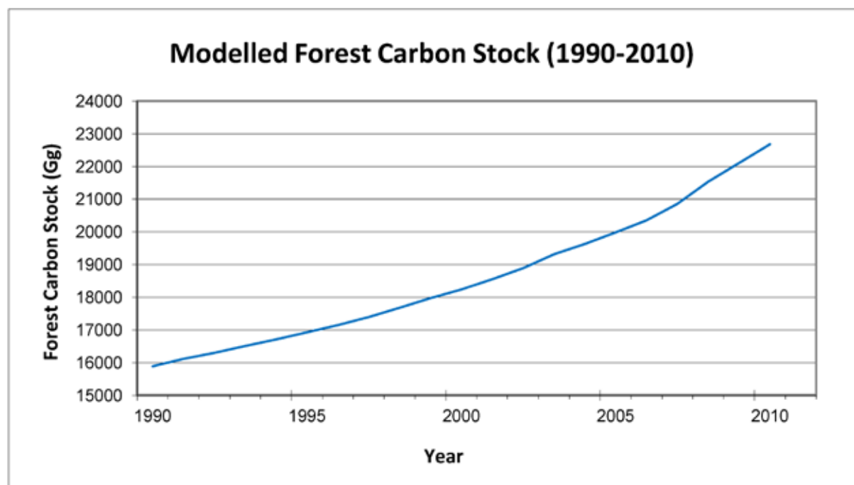
Figure 4.9. Modelled annual total forest carbon stock (1990–2010).
