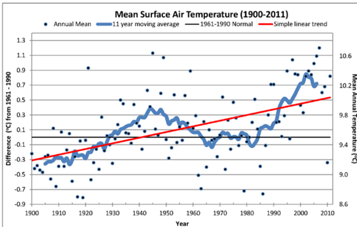
Figure 2.1. Annual mean surface air temperature (1900–2011).
