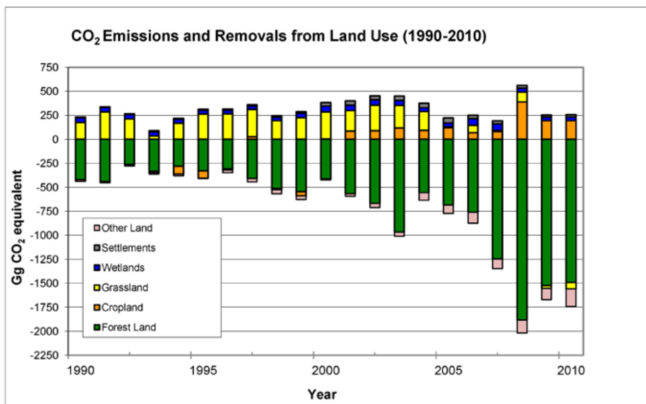
Figure 4.2. Emissions (+) and removals (-) of carbon associated with the management and use of land (1990–2010).
