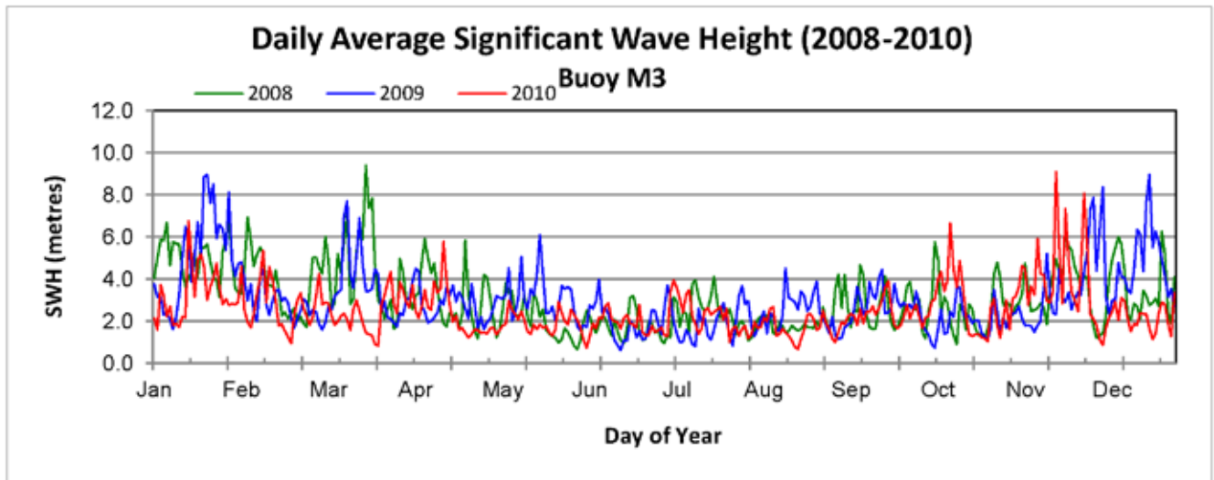
Figure 3.8. Daily averaged significant wave height at Buoy M3 (2008–2010).
