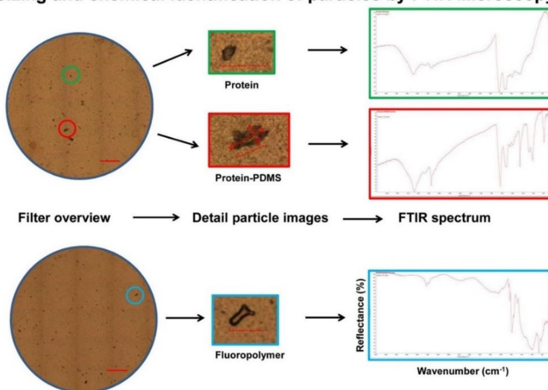
Figure 2.6: Sizing and chemical identification of particles produced from pharmaceutical vial stoppers analysed by FTIR microscopy. Sizing identified particles of \geq 25 \mu\text{m} in length suitable for chemical analysis (rectangular boxes), scale bar 100 \mu\text{m} . FTIR analysis identified protein, protein-PDMS and fluoropolymer particles. The figure is reprinted from the reference with permission of the publisher. 90
