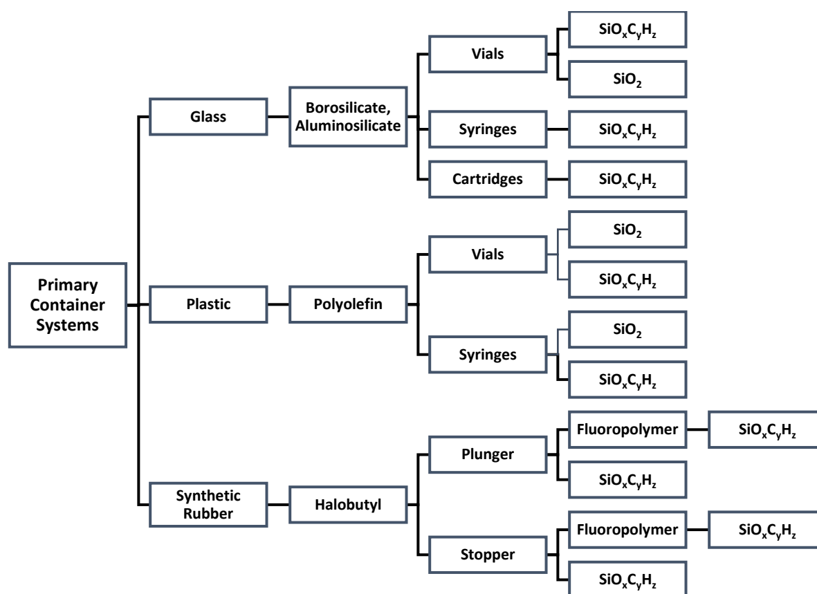
Figure 2.4: The most common primary packaging and container systems used for liquid parenteral protein formulations and their associated surface coatings. 65,69 SiO 2 : silicon dioxide; SiO x C y H z : siloxane.
