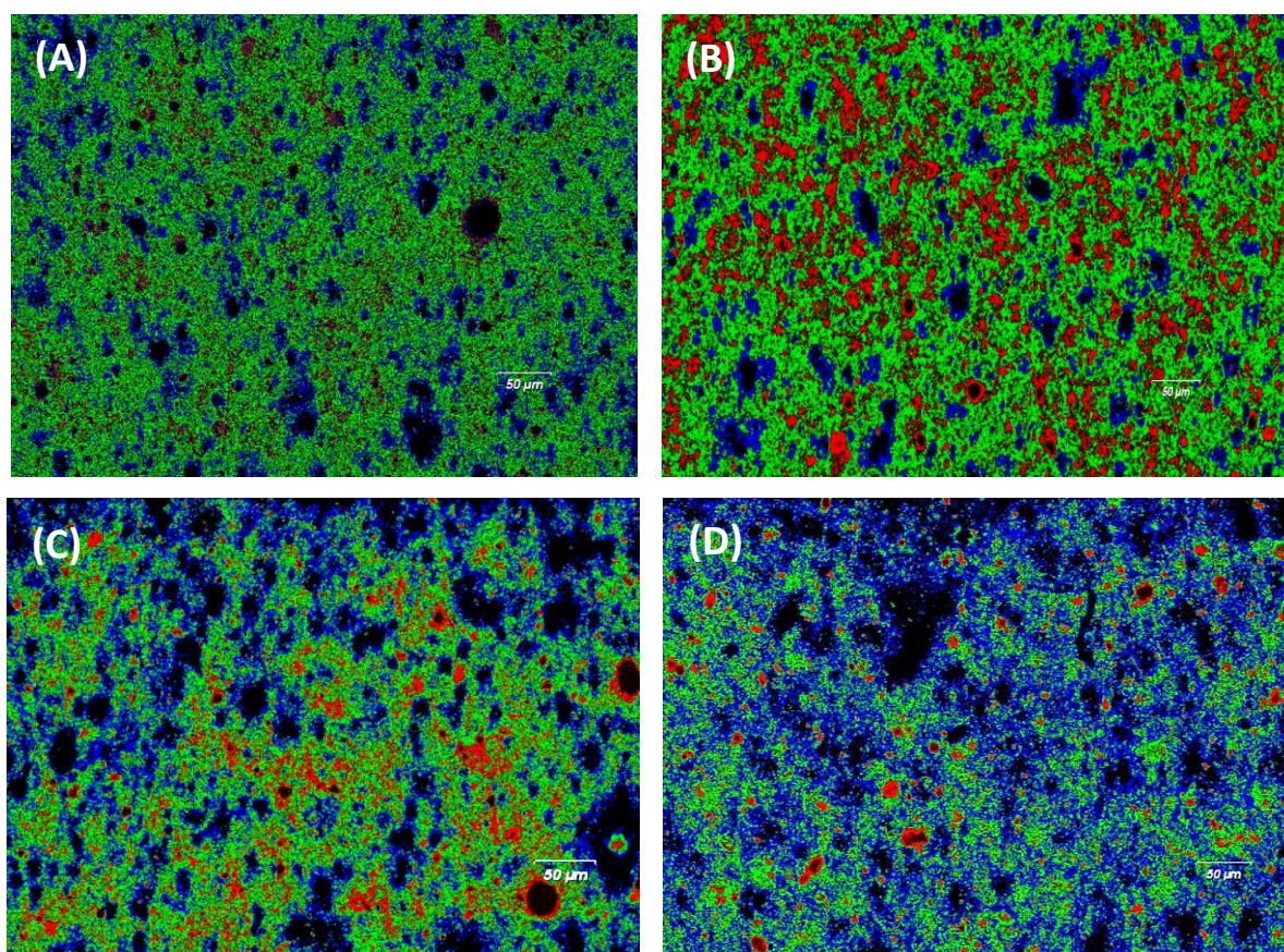
Figure 5.8: Raman hyperspectral image of the reference stopper plug (A), after autoclavation at 121°C for 15 minutes (B), immersion in water for 24 hours (C), and 4 weeks exposure to a placebo formulation under thermal agitation stress (D). Red colouring indicates the signal of \text{TiO}_2 near the surface, green is the \text{TiO}_2 signal at the midpoint, and blue is the signal at the lowest depth measured (2 μm). The black represents areas where the Raman signal was oversaturated due to intense autofluorescence. Scale bar 50 μm in all images.
