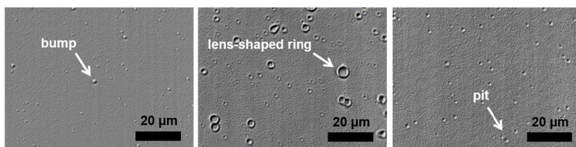
Figure 1.4: C-laser differential interference contrast images of commercial glass primary packaging after different processing conditions which can result in defects on the glass surface. The figure is reprinted from the reference with permission of the publisher. 81
