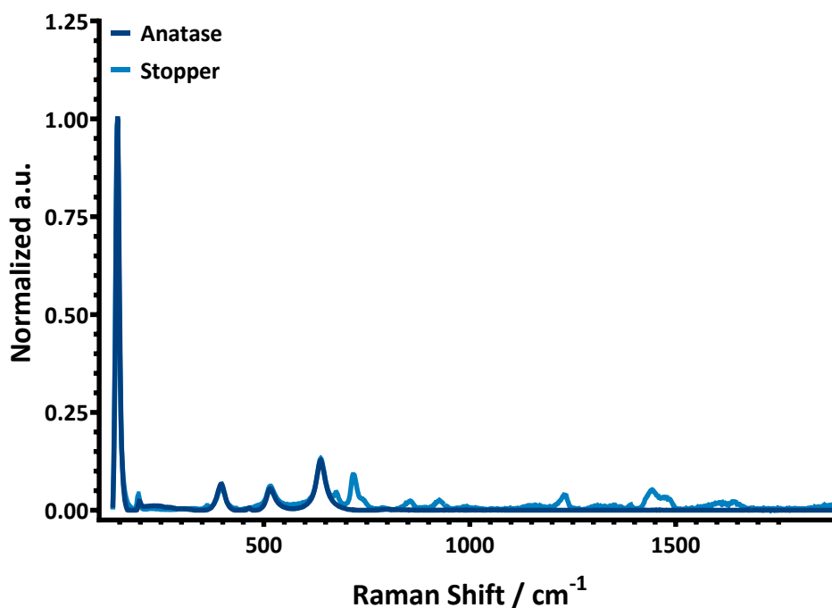
Figure S5.7: Raman spectra of titanium dioxide (TiO 2 , Anatase) reference vs TiO 2 signal obtained from an uncoated stopper. The component was generated by reviewing <400,000 spectra using Renishaw's Empty Modelling™ algorithm.
