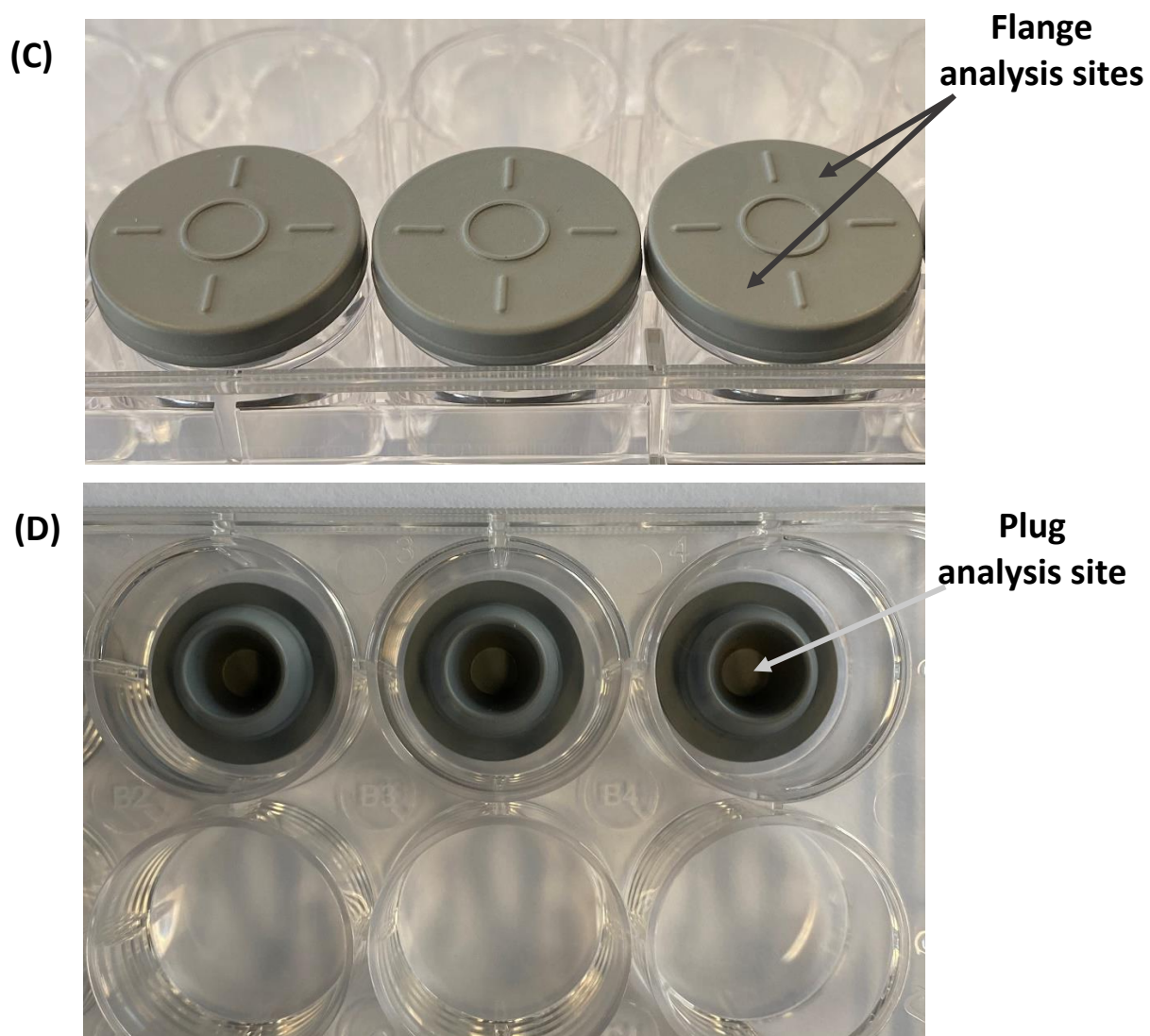
Figure S5.2: Schematic diagram of plasma deposition system (A), substrate set-up for the DoE (B), close-up view of the top of the stoppers showing flange sites analysed (C) and substrate set-up used in the study to coat the drug contact side (plug) of the stopper vial (D).
