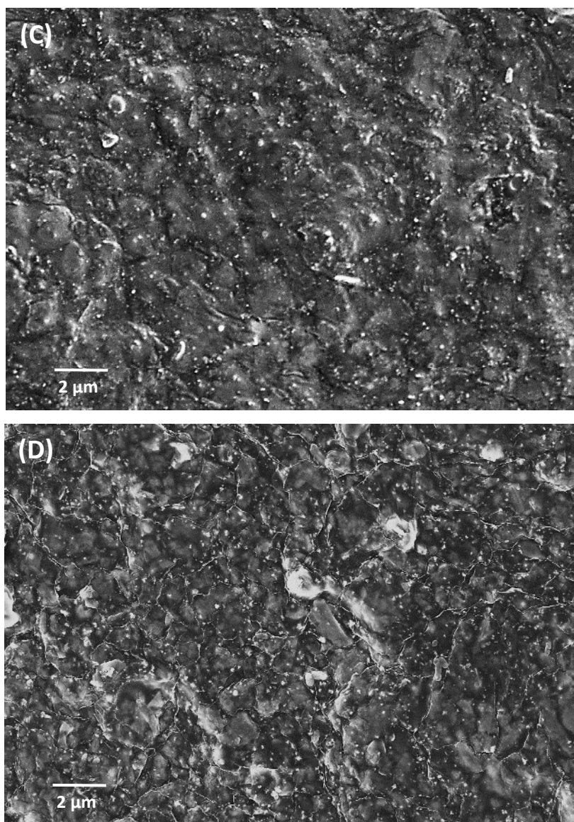
Figure 5.3: SEM images of stopper surfaces. Uncoated (A) and poly(MPC-co-BMA)-coated stopper (B), scale bar 10 μm. Higher magnification images of uncoated (C) and poly(MPC-co-BMA)-coated (D) stoppers, scale bar 2 μm.
