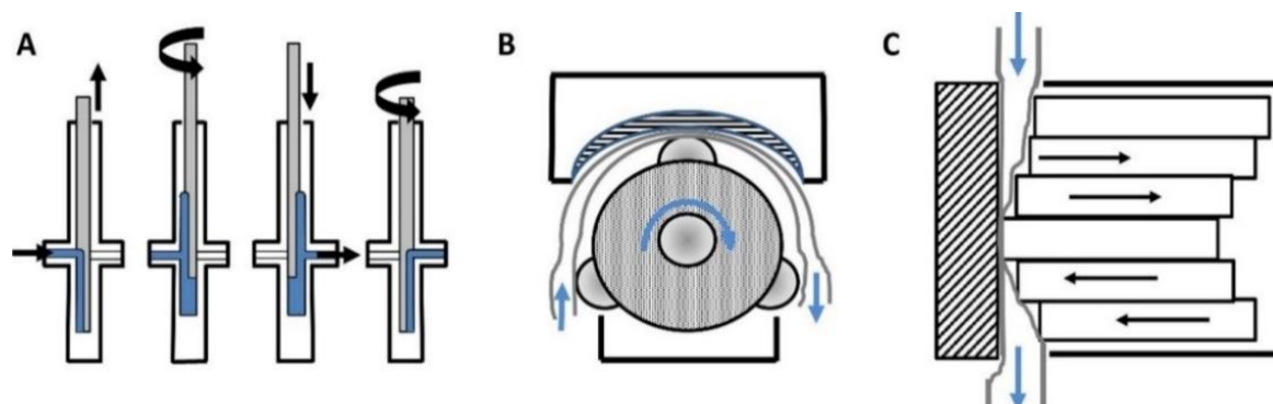
Figure 2.3: Schematic presentation of select biopharmaceutical fill pumping systems: rotary piston pump (A), radial peristaltic pump (B) and linear peristaltic pump (C). The figure is reprinted from the reference with permission of the publisher. 190
