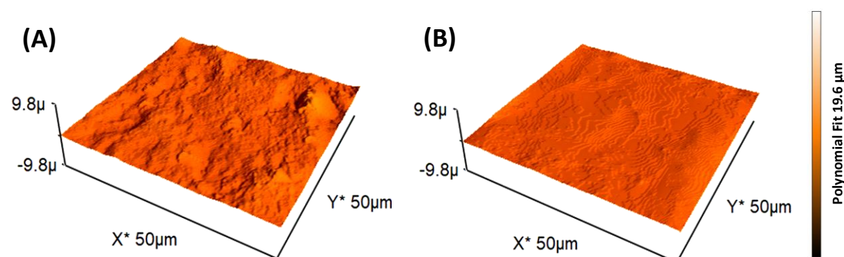
Figure 5.5: Representative AFM images showing 50 x 50 \mu\text{m} area on the uncoated (A) and poly(MPC-co-BMA)-coated (B) surfaces. Each sample was evaluated in duplicate and n=3 independent samples were analysed for the uncoated and coated halobutyl rubber flange septas.
