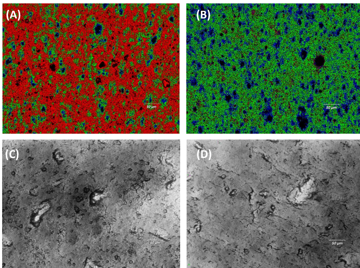
Figure 5.7: Raman hyperspectral images of the drug contact area of uncoated (A) and poly(MPC-co-BMA)-coated (B) stopper plugs. Red colouring indicates the signal of \text{TiO}_2 near the surface, green represents the \text{TiO}_2 signal at the midpoint, and blue denotes the signal at the lowest depth measured ( 2\ \mu\text{m} ). The black represents areas where the Raman signal was oversaturated due to intense autofluorescence. Topographic images of uncoated (C) and poly(MPC-co-BMA)-coated (D) stopper plugs. Scale bar 50\ \mu\text{m} in all images.
