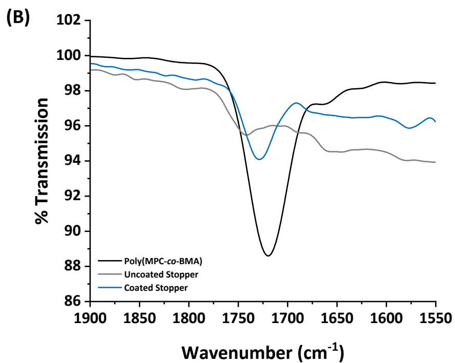
Figure 5.6: Representative FTIR spectra of poly(MPC-co-BMA) raw material and coatings produced on NaCl discs by wet and plasma deposition methods (A) and poly(MPC-co-BMA) immobilised on the stopper surface (B). Three independent samples were evaluated for each coating process to the NaCl discs.
