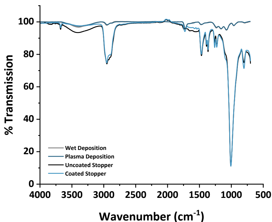
Figure S5.4: FTIR spectra of uncoated stopper, poly(MPC-co-BMA)-coated stopper and coatings produced on NaCl discs by wet and plasma deposition methods.
