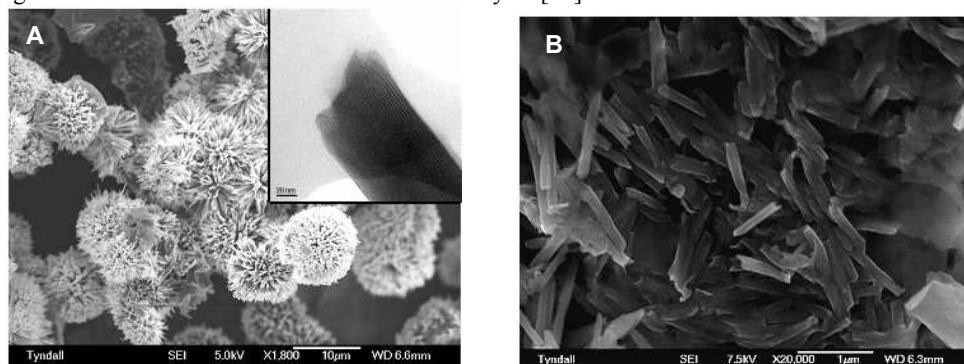
Fig. 1 (a) FESEM image of the nano-urchin of vanadium oxide (inset) HRTEM image of a nano-urchin tube with uniform hollow core and open ended. (b) FESEM image of nanorods of vanadium oxide.
