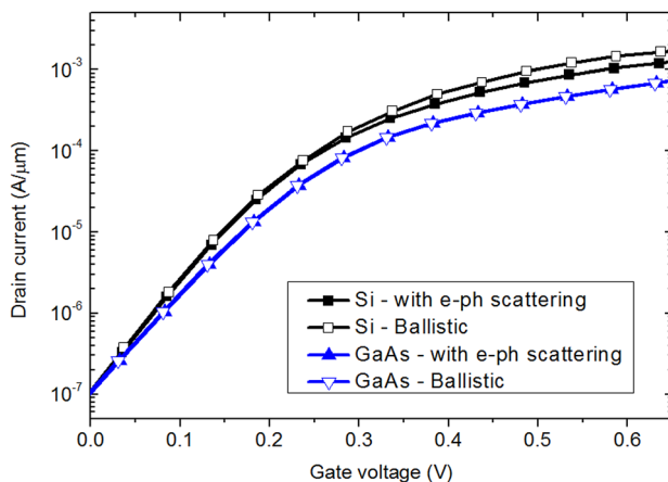
FIG. 2. Transfer characteristics of Si and GaAs channels ( L_{gate} = 10 \text{ nm} ).
