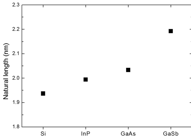
FIG. 4. Natural length of Si and other III-V compound materials for the simulated nanowire device.
