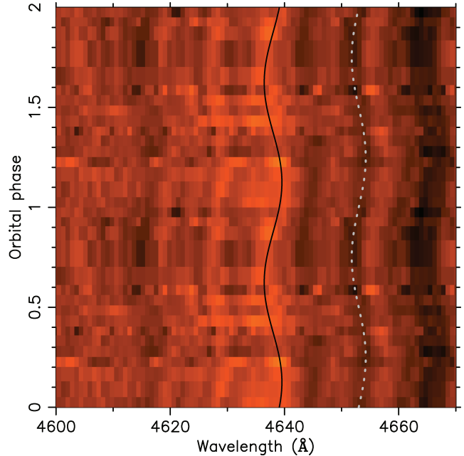
Figure 8. Trailed spectrogram of the data near the N III \lambda 4640.64 emission line. The systemic velocity has not been removed, so the N III \lambda 4640.64 line is near \lambda 4638 . The solid line marks the S-wave from N III \lambda 4640.64 emission, while the dotted line marks one of the nearby secondary absorption lines.
