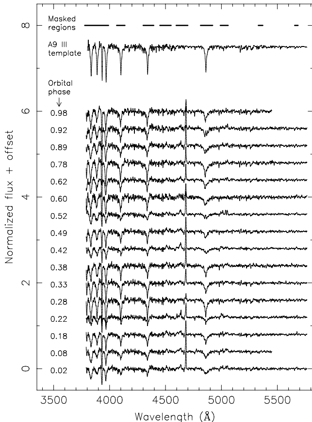
Figure 1. 16 normalized spectra from 2006 September and October. The A9 III template spectrum is also shown. The wavelength regions masked from the cross-correlation are also marked. The spectra have been boxcar smoothed.
