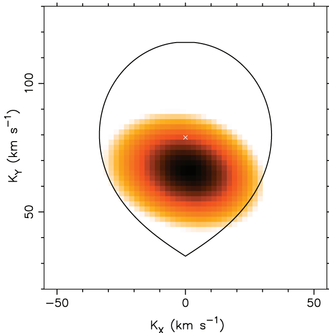
Figure 7. Doppler tomogram of the He II \lambda 4686 emission line, focused on the region of the secondary star. The Roche lobe of the secondary is overplotted for K_2 = 79 \text{ km s}^{-1} and q = 0.42 .
