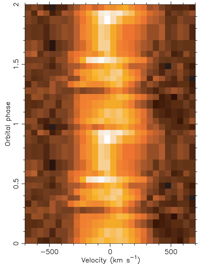
Figure 5. Trailed spectrogram of the data used to construct the He II Doppler tomograms.
