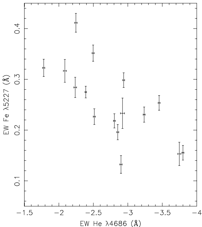
Figure 10. EW of the Fe I \lambda 5227.15 absorption line versus the EW of the He II \lambda 4686 emission line. Assuming that the EW of the He II \lambda 4686 emission line is correlated with the intensity of the X-rays intercepted by the secondary star, this relationship shows that the EW of the Fe I \lambda 5227.15 absorption line decreases with increasing X-ray flux.
