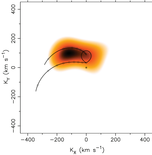
Figure 9. Doppler tomogram of the N III \lambda 4640.64 emission line. The gas stream and Roche lobe of the secondary are overplotted for K_2 = 79 \text{ km s}^{-1} and q = 0.42 .
