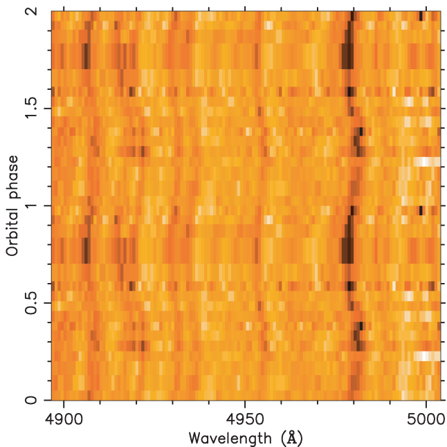
Figure 3. Trailed spectrogram for the data between \lambda\lambda 4900 and 5000, showing some of the narrow absorption lines from the secondary.
