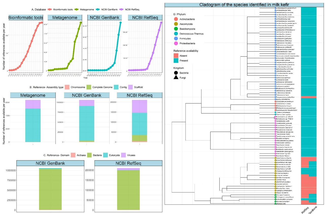
Figure 2: Annual growth and availability in reference data available for the interpretation of metagenomic data including reference genomes in the NCBI database ( https://www.ncbi.nlm.nih.gov/ ). (A.) Annual growth (from 2005 to 2021) in reviewed research papers introducing novel and improved tools designed for the interpretation of metagenomic data, metagenomes available in the NCBI GenBank database and reference genomes in the NCBI GenBank and NCBI RefSeq [63, 64]; (B.) Available Metagenome, NCBI Genbank and NCBI Refseq reference data separated by assembly level. (C.) Available Metagenome, NCBI Genbank and NCBI Refseq reference data separated by domain. (D.) Cladogram of bacterial and fungal species found in milk kefir, species information obtained from [65]. Tip labels represent the species detected, e.g., Lentilactobacillus parabuchneri , tip colour represents the phylum, and shape represents the kingdom of the species. Presence/absence heatmap displays the availability of reference genomes for each of the listed species in both NCBI RefSeq and NCBI GenBank databases. Metagenome, Refseq and Genbank derived data was generated and analysed in R using the Biomart package [66]. Visualisation was performed using the ggplot2 package [67] and ggtree package [68].
