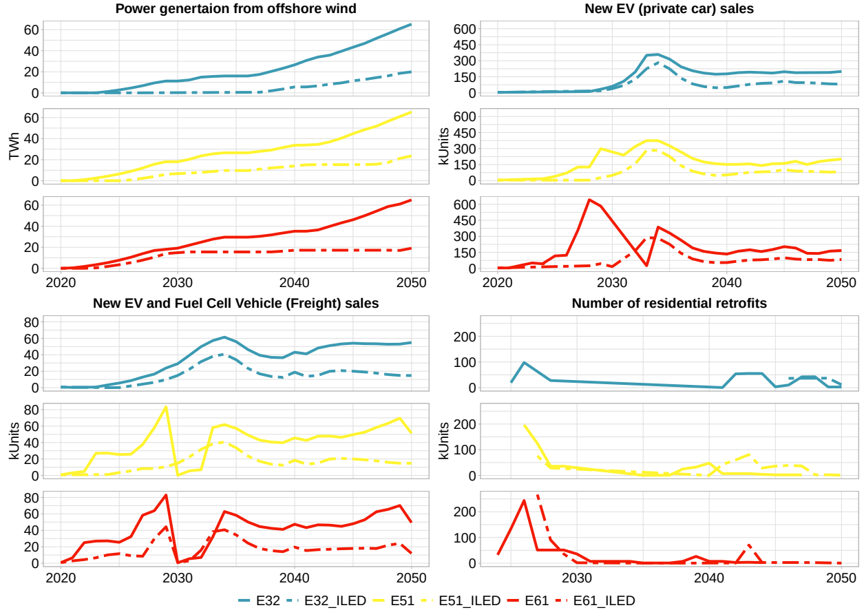
Figure 3.16: Novel technology uptake between 2020 and 2050
