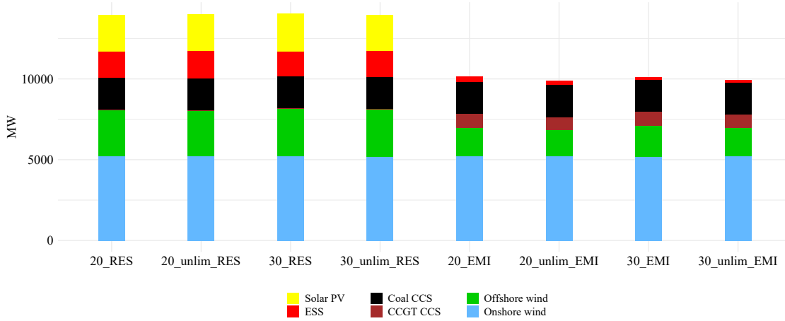
Figure 5.12: Generation mix in 2030
