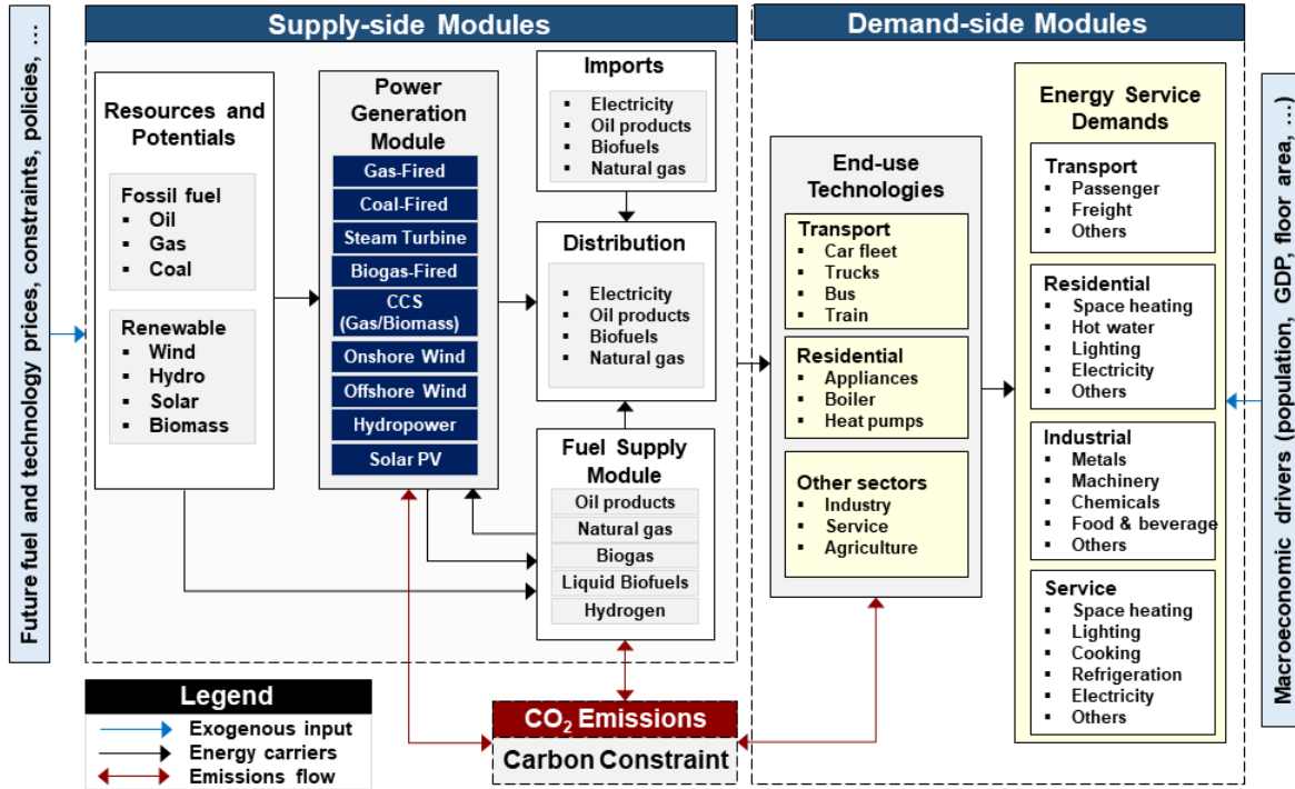
Figure 2.1: Simplified representation of reference energy system in TIM
