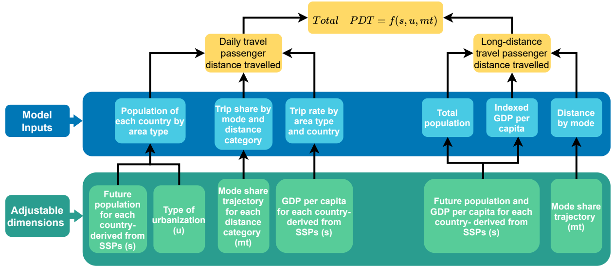
Figure 6.2: Passenger mobility demand model inputs and the adjustable dimensions
