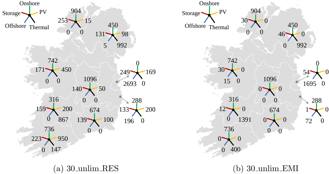
Figure 5.15: Regional distribution of generation capacity in RES-E and emission target cases in 2030
