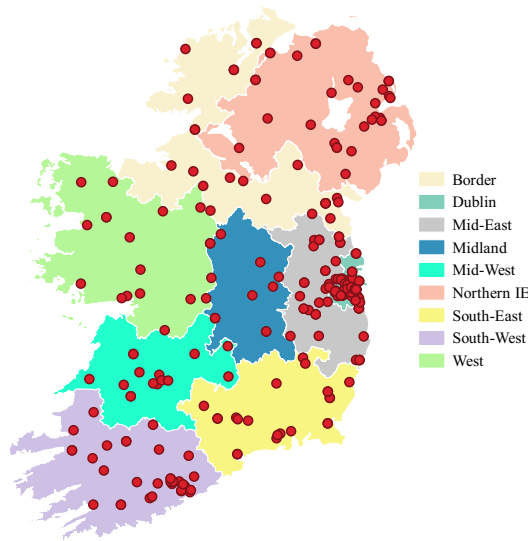
Figure 5.2: Candidate connection nodes of renewable and storage investment
