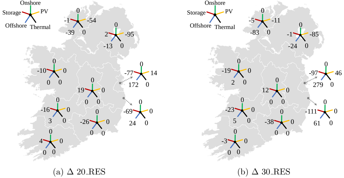
Figure 5.4: Change in regional generation mix (MW) with respect to Base_RES in 2030
