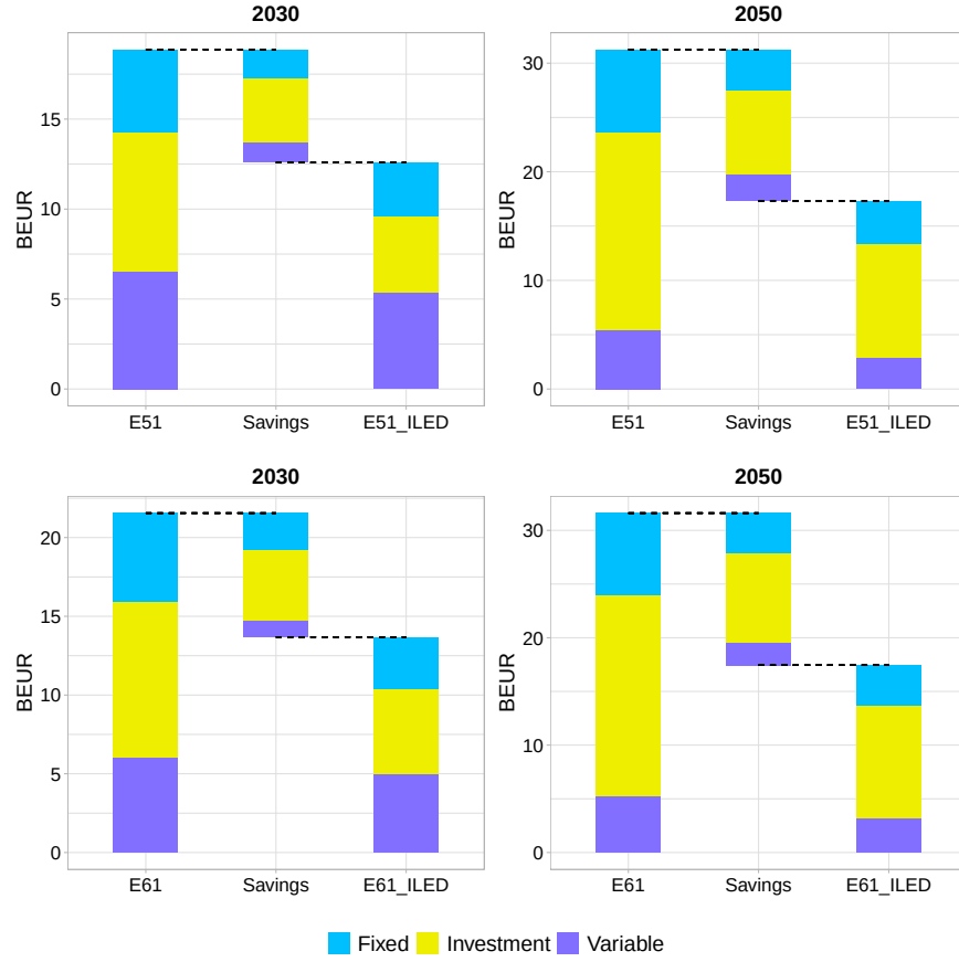
Figure 3.13: Difference in energy system costs (fixed, investment and variable) between BAU ESD and ILED pathways in 2030 and 2050
