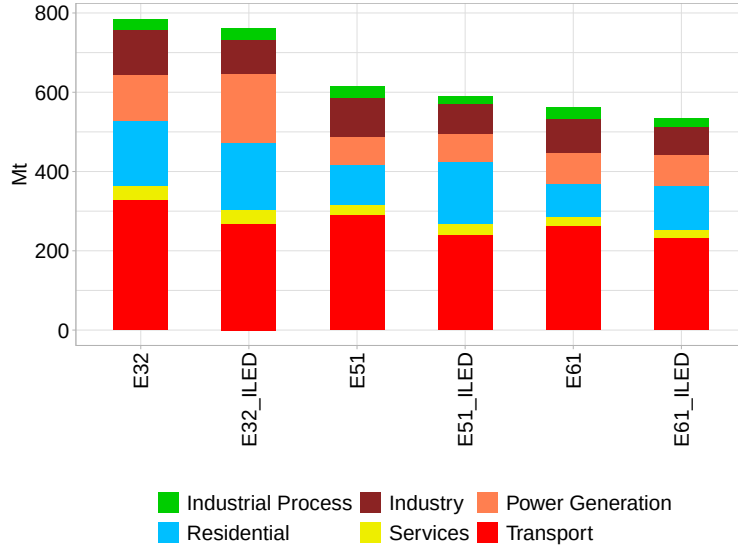
Figure 3.17: Cumulative sectoral CO 2 emissions between 2020 and 2050
