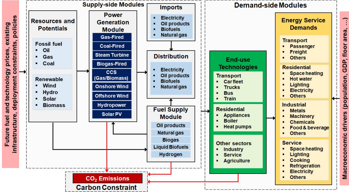
Figure 3.5: Schematic representation of reference energy system (RES) in the newly developed TIMES-Ireland Model (TIM)
