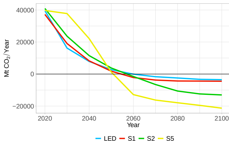
Figure 3.1: Evolution of CO 2 emissions in the illustrative pathways featured in SR 1.5 where S1, S2 and S5 are based on Shared Socioeconomic Pathways (SSPs) SSP1, SSP2 and SSP5 respectively (Riahi et al., 2017; Rogelj et al., 2018; Gidden et al., 2019)
