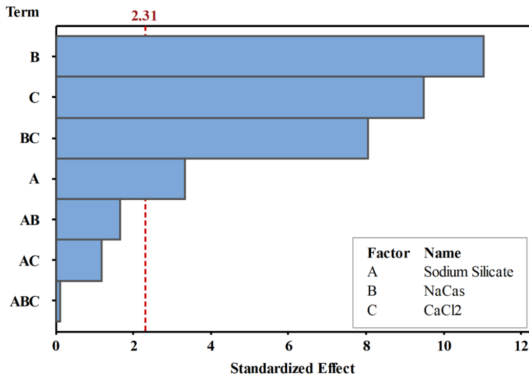
Figure 4.6 Pareto chart of standardised effects (response is particle size, \alpha = 0.05 ). Significant effects are those that extend beyond the reference line (2.31).
