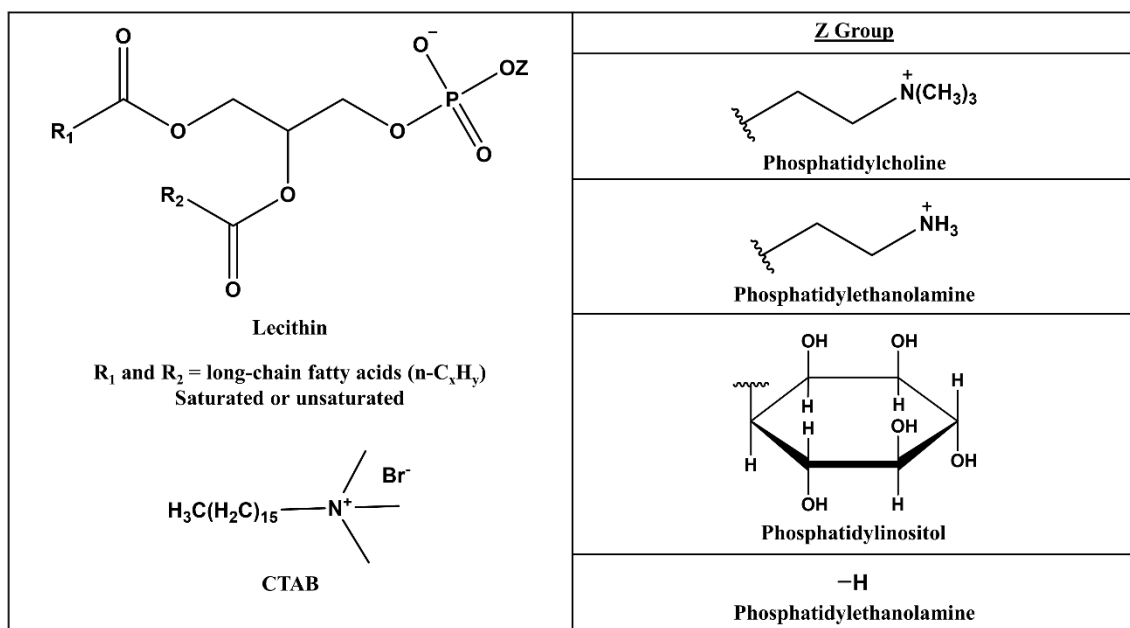
Figure 1.6 General structure of lecithin (top left) and it's variations (right column). R_1 and R_2 = fatty acid residues. CTAB is shown (bottom left) for structural comparison. Notice the similarities between the quaternary ammonium headgroups of phosphatidylcholine and phosphatidylethanolamine and that of CTAB. The long-chain fatty acid residues of lecithin are also structurally and chemically similar to the long carbon tail of CTAB.
