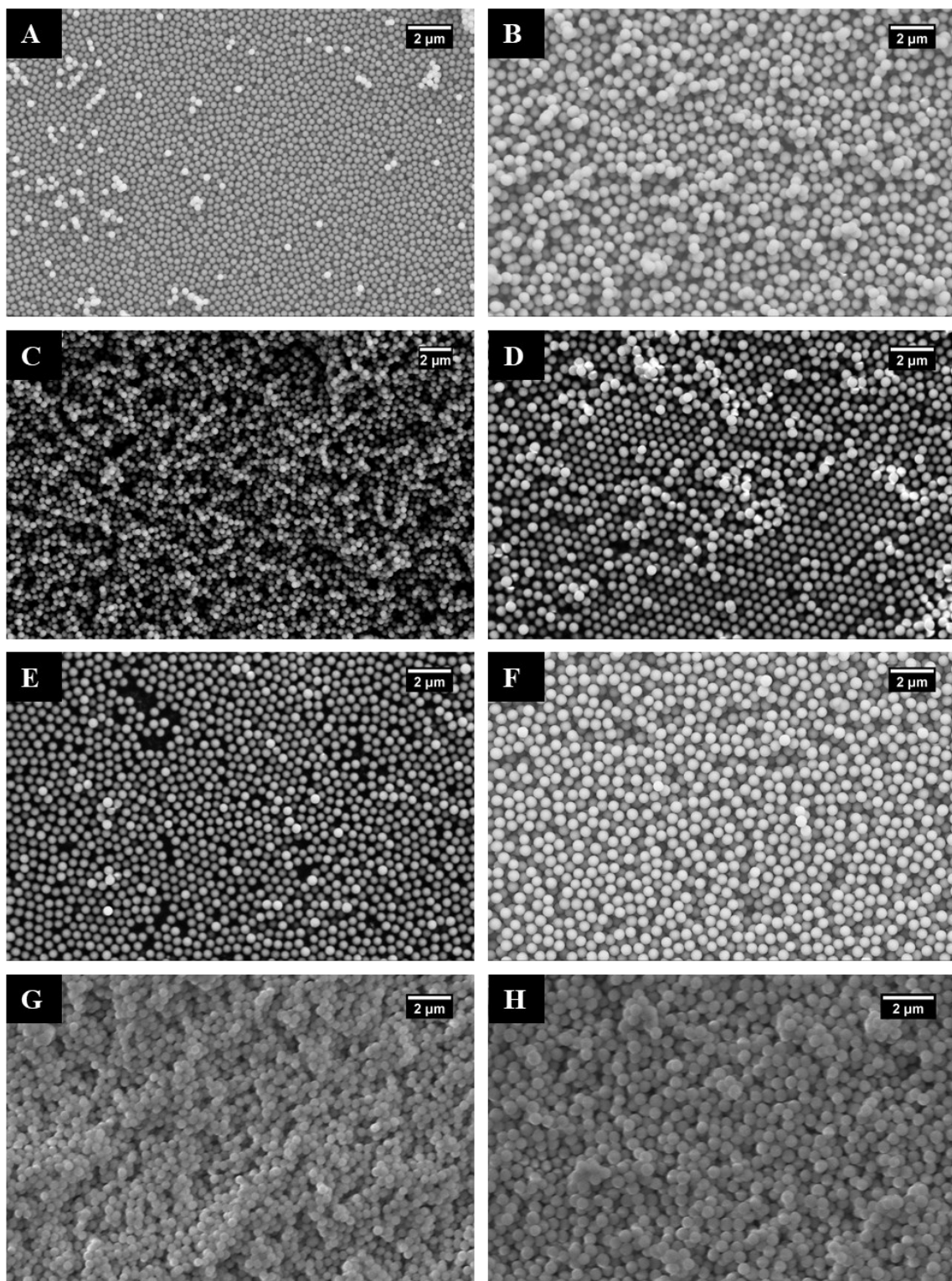
Figure 2.1 SEM images of silica nanoparticles synthesised by varying amount of ethanol. (a) 1 ml EtOH, (b) 2 ml EtOH, (c) 3 ml EtOH, (d) 4 ml EtOH, (e) 5 ml EtOH, (f) 6 ml EtOH, (g) 7 ml EtOH, and (h) 8 ml EtOH. All other reactants kept constant.
