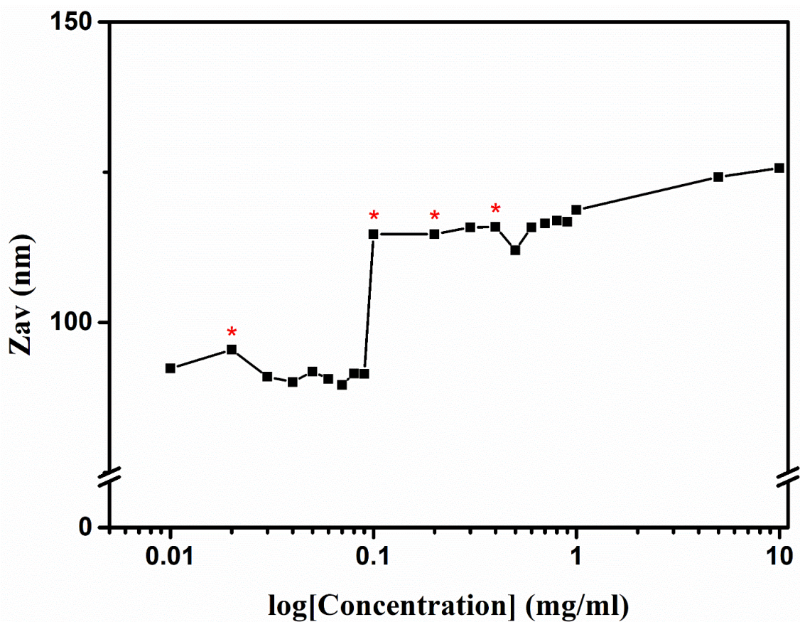
Figure A3.2 Z-average for PC in acetate buffer (0.05M, pH 5.92) over a wider concentration range. PC1, PC2, PC3, and PC4 are marked with (*).
