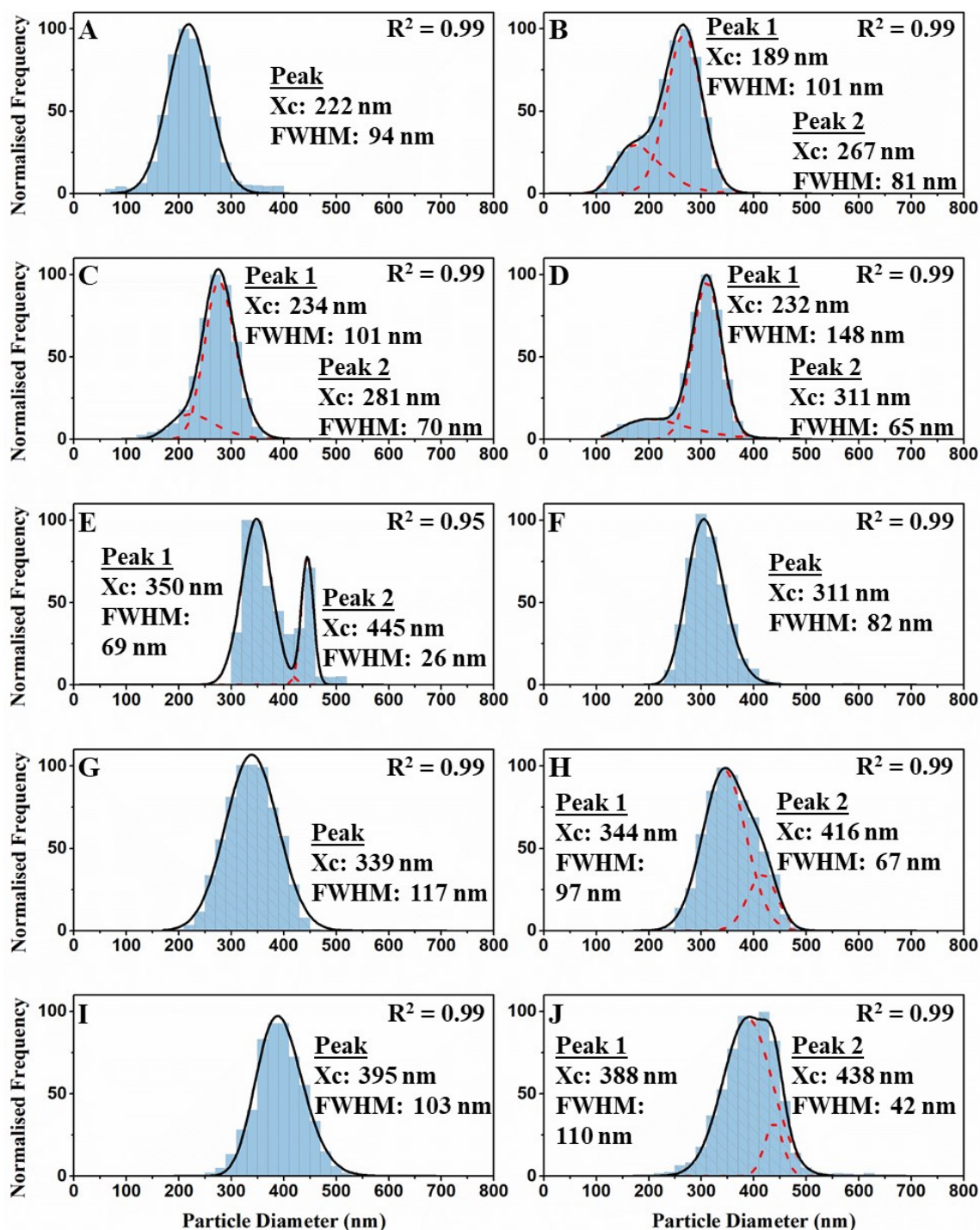
Figure 2.5 PSDs of silica nanoparticles synthesised by varying amount of TEOS. (a) 0.2 ml TEOS, (b) 0.3 ml TEOS, (c) 0.4 ml TEOS, (d) 0.5 ml TEOS, (e) 0.6 ml TEOS, (f) 0.7 ml TEOS, (g) 0.8 ml TEOS, (h) 0.9 ml TEOS, (i) 1 ml TEOS, and (j) 1.1 ml TEOS. All other reactants kept constant.
