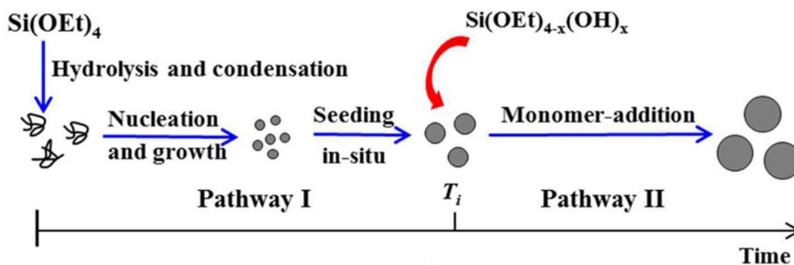
Figure 1.2 From Han et al. 59 Particle growth can be divided into two consecutive stages, Pathway I (nucleation-growth) and Pathway II (monomer addition) at high ammonia concentration ( \geq 0.95 M); or Pathway I (nucleation-growth), Pathway I+II (continuous nucleation and monomer addition) at low ammonia concentration ( < 0.95 M).
