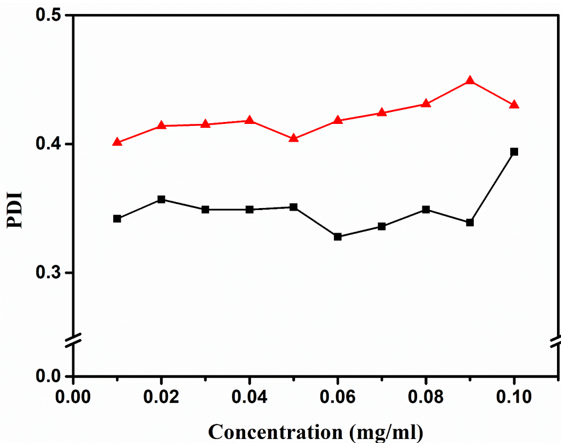
Figure A3.3 PDI for PC (■) and SL (▲) in acetate buffer (0.05M, pH 5.92) at various concentrations (from DLS data).
