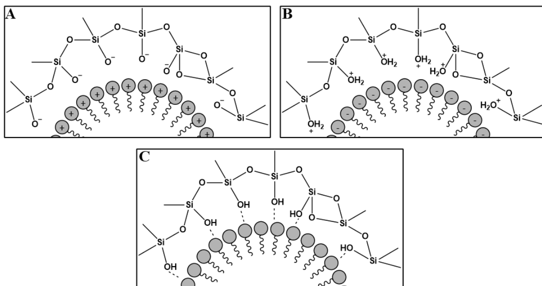
Figure 1.1 Example of (a) interaction of cationic surfactant with negatively charged silicate species in basic conditions, (b) interaction of anionic surfactant with positively charged silicate species in acidic conditions and (c) interaction of non-ionic surfactant with silica through hydrogen bonding. Note: other types of interactions exist, shown here are the three most common. Adapted from Alothman. 49
