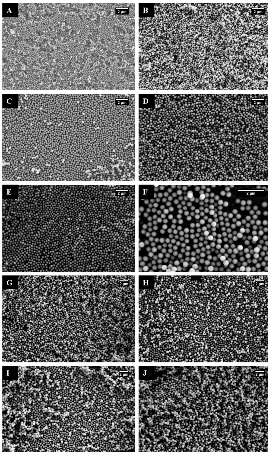
Figure 2.4 SEM images of silica nanoparticles synthesised by varying amount of TEOS. (a) 0.2 ml TEOS, (b) 0.3 ml TEOS, (c) 0.4 ml TEOS, (d) 0.5 ml TEOS, (e) 0.6 ml TEOS, (f) 0.7 ml TEOS, (g) 0.8 ml TEOS, (h) 0.9 ml TEOS, (i) 1 ml TEOS, and (j) 1.1 ml TEOS. All other reactants kept constant.
