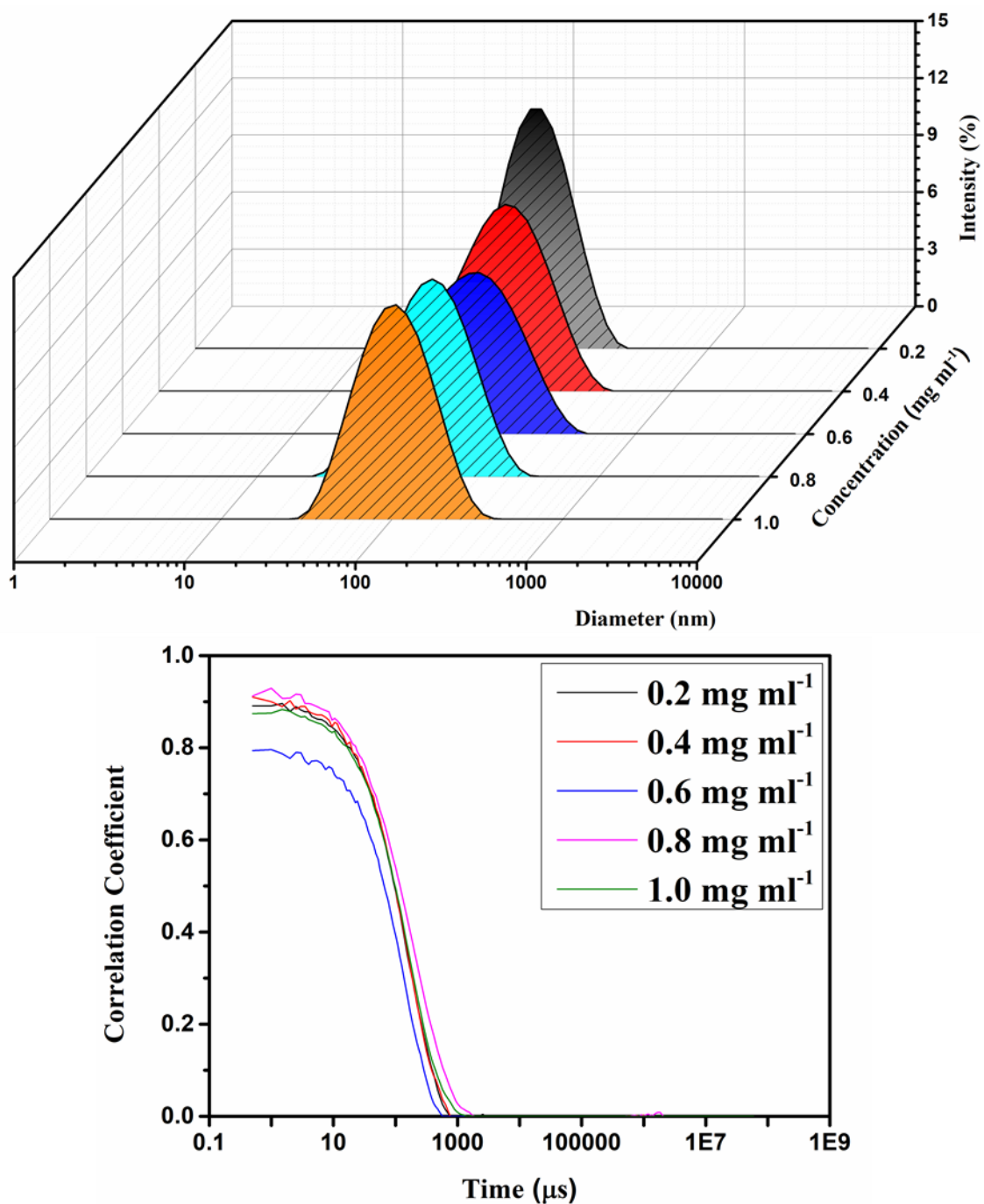
Figure 4.5 Distribution data from DLS measurements of sodium caseinate at various concentrations with 8 mM CaCl 2 in acetate buffer (0.05 M, pH 5.94) (top). Correlograms (bottom).
