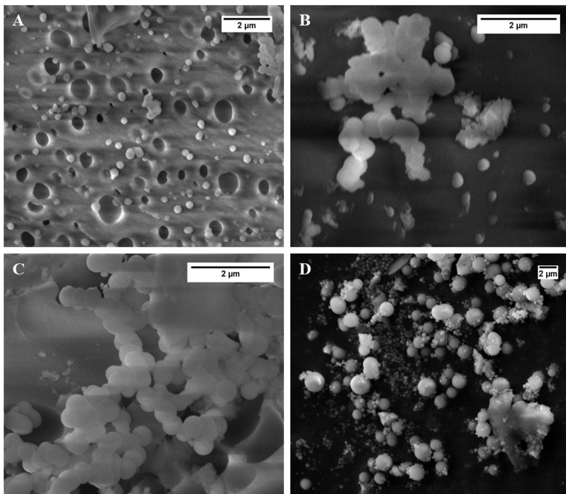
Figure 3.4 SEM micrographs of silica particles produced when using SL with various aliquots of SL (a) 0.004 \text{ mg ml}^{-1} SL (SL1), (b) 0.04 \text{ mg ml}^{-1} SL (SL2), (c) 0.08 \text{ mg ml}^{-1} PC (SL3), and (d) 1.8 \text{ mg ml}^{-1} SL (SL4). All reactions done in 50 ml acetate buffer ( 0.05\text{M} , pH 5.92) with 820 \text{ } \mu\text{L} sodium silicate at room temperature. Scale bars are 2 \mu\text{m} . Background in (a) is carbon tape.
