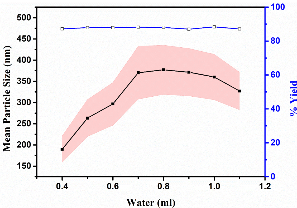
Figure 2.12 Effect of water volume on mean particle size (—■—) and percent yield (—□—). Red shaded area is the standard deviation of mean particle size.
