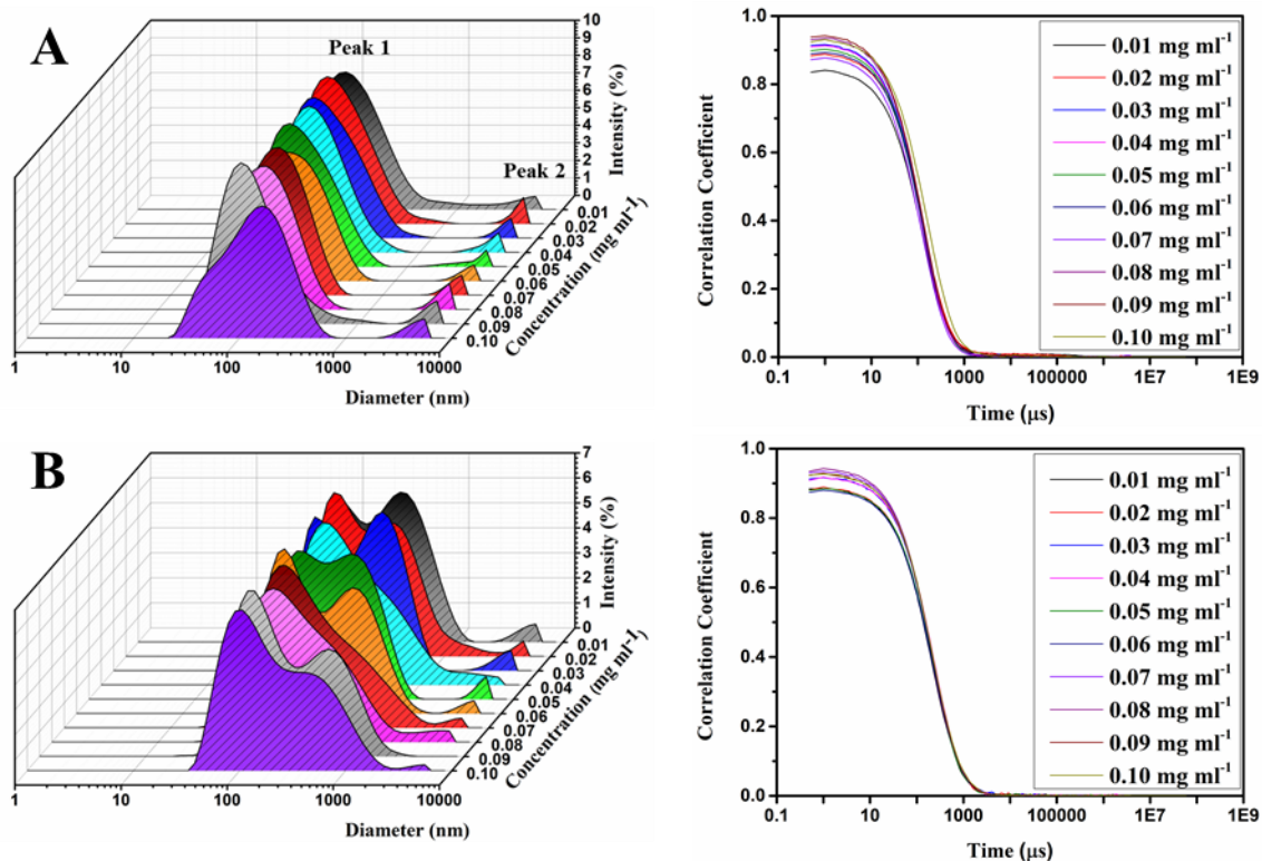
Figure 3.1 PSD data and correlograms from DLS measurements of (a) phosphatidylcholine in acetate buffer (0.05 M, pH 5.92) and (b) soy lecithin in acetate buffer (0.05 M, pH 5.92) at various concentrations.
