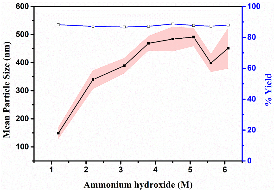
Figure 2.9 Effect of ammonium hydroxide concentration on mean particle size (—■—) and percent yield (—□—). Red shaded area is the standard deviation of mean particle size.
