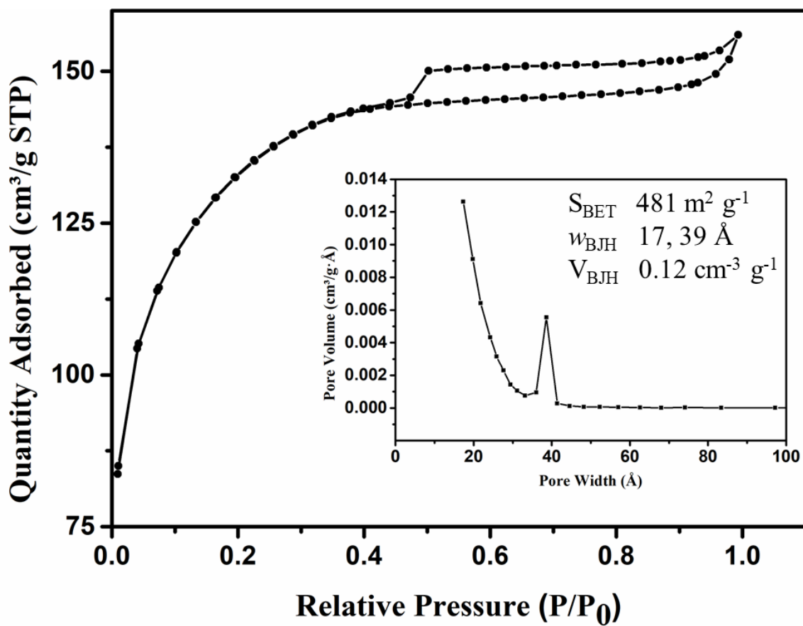
Figure A3.4 N_2 sorption isotherm and pore size distribution (inset) of silica particles produced with 0.08 mg ml -1 SL (SL3).
