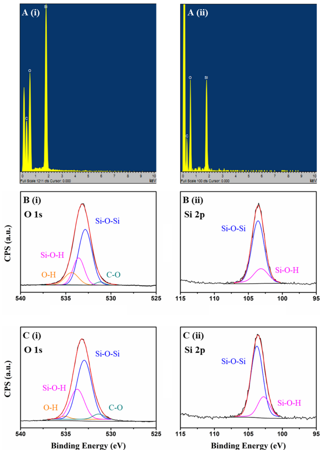
Figure 3.6 Energy-dispersive x-ray spectra (a(i)) of PC2 (0.1 mg ml -1 PC), and (a(ii)) SL4 (1.8 mg ml -1 SL), (b) XPS spectra of O 1s and Si 2p peaks of PC2 (0.1 mg ml -1 PC). Red curve is the cumulative fitting, and (c) XPS spectra of O 1s and Si 2p peaks of SL4 (1.8 mg ml -1 SL). Red curve is the cumulative fitting.
