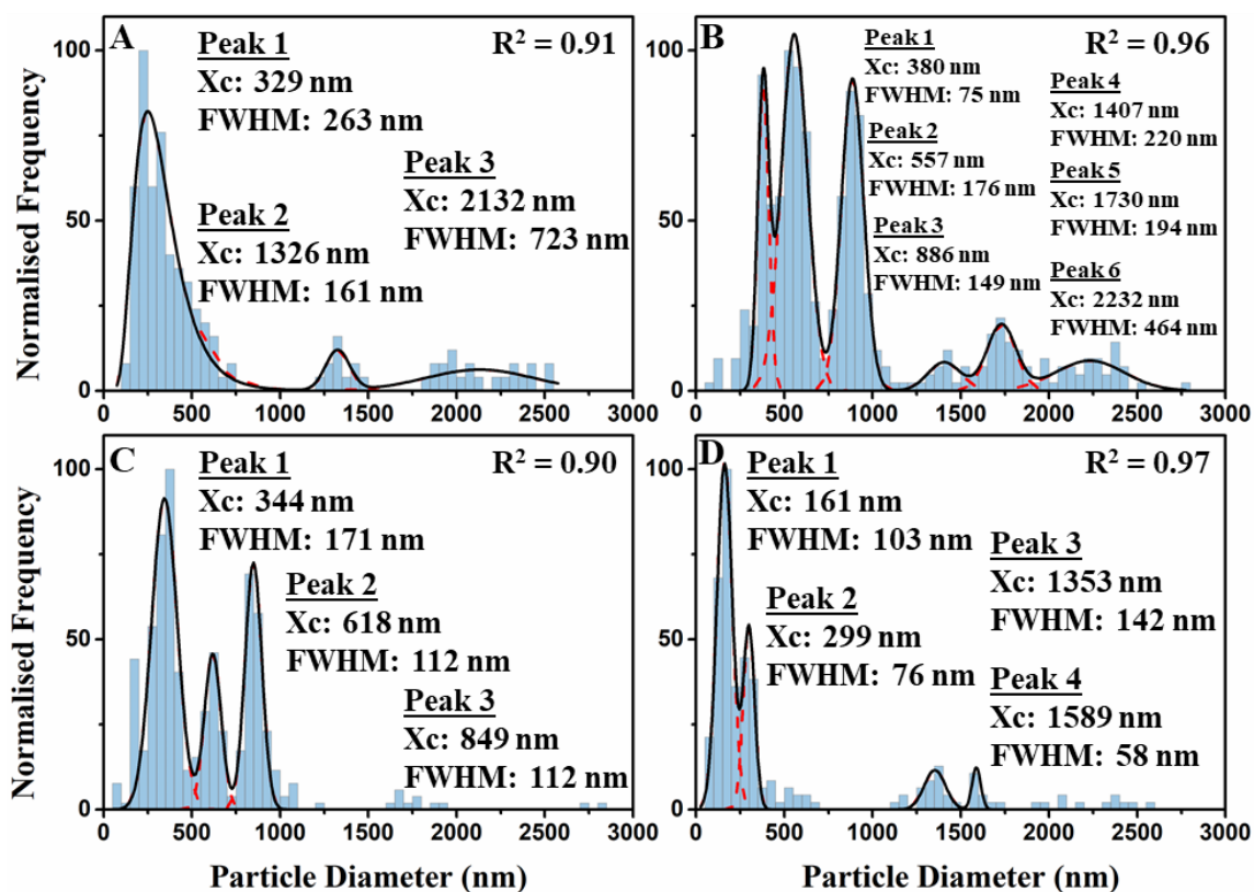
Figure 3.3 PSDs of silica particles produced when using PC (a) 0.02 mg ml -1 PC (PC1), (b) 0.1 mg ml -1 PC (PC2), (c) 0.2 mg ml -1 PC (PC3), and (d) 0.4 mg ml -1 PC (PC4). All reactions done in 50 ml soybean oil with 500 \mu l sodium silicate at room temperature.
