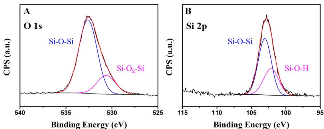
Figure 4.10 XPS spectra of (a) O 1s and (b) Si 2p peaks of R1 (486 \mu L sodium silicate, 20 mg NaCas, and 8 mM \text{CaCl}_2 ). Red curve is the cumulative fitting.
