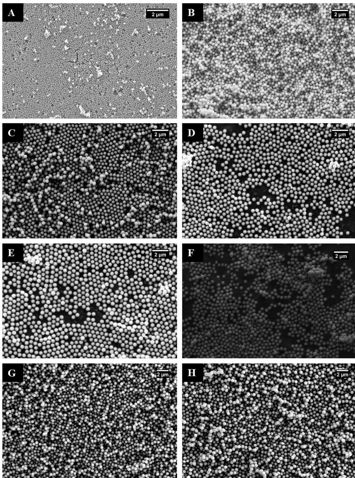
Figure 2.7 SEM images of silica nanoparticles synthesised by varying ammonium hydroxide concentration. (a) 1.2 M \text{NH}_4\text{OH} , (b) 2.2 M \text{NH}_4\text{OH} , (c) 3.1 M \text{NH}_4\text{OH} , (d) 3.8 M \text{NH}_4\text{OH} , (e) 4.5 M \text{NH}_4\text{OH} , (f) 5.1 M \text{NH}_4\text{OH} , (g) 5.6 M \text{NH}_4\text{OH} , and (h) 6.1 M \text{NH}_4\text{OH} .
