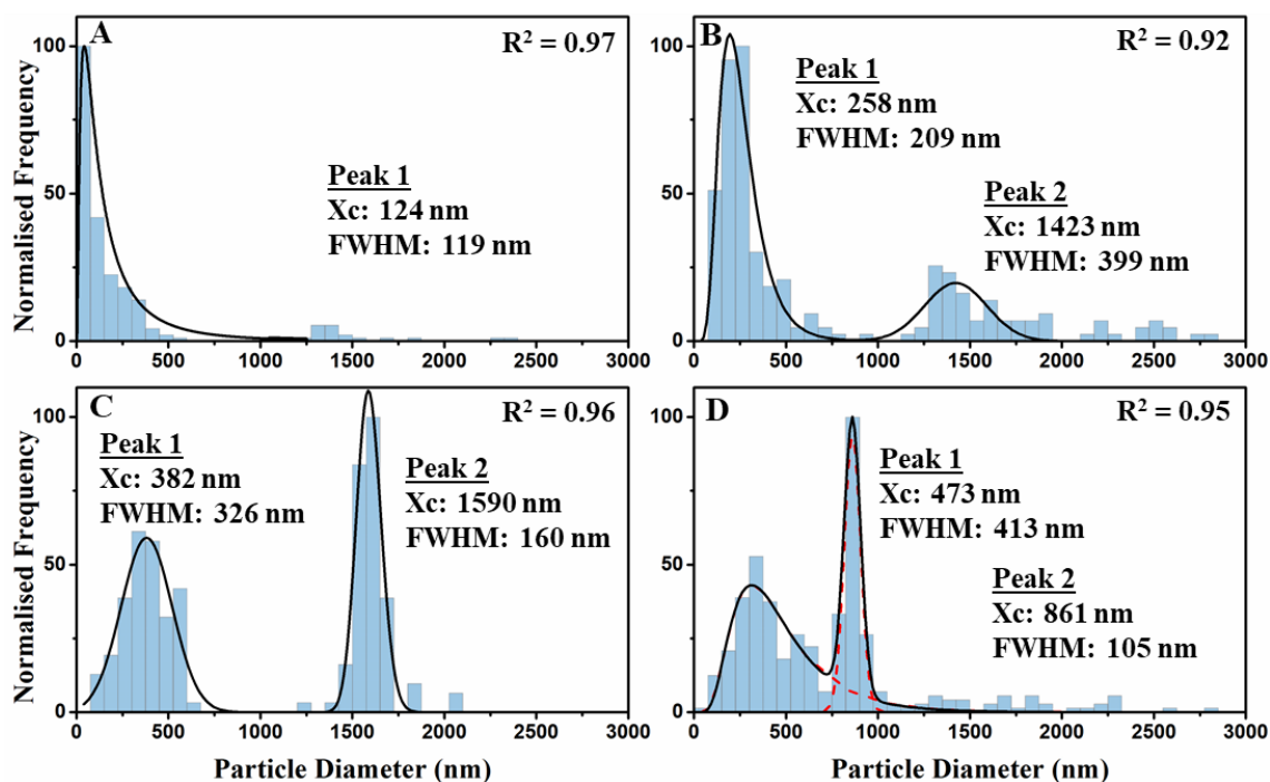
Figure 4.4 PSDs of particles prepared with (a) 0.2 \text{ mg ml}^{-1} NaCas (BF1), and (b) 0.4 \text{ mg ml}^{-1} NaCas (BF2), (c) 162 \text{ }\mu\text{L} sodium silicate (BF3), and (d) 810 \text{ }\mu\text{L} sodium silicate (BF4).
