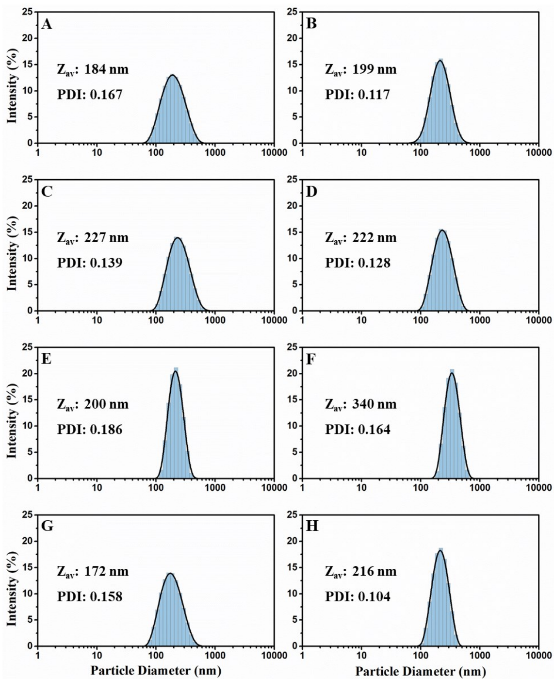
Figure A4.8 DLS measurements of particles synthesised in factorial analysis (see Table A4.1). (a) Run 11, (b) Run 12, (c) Run 13, (d) Run 14, (e) Run 15, (f) Run 16, (g) Run 17, and (h) Run 18.
