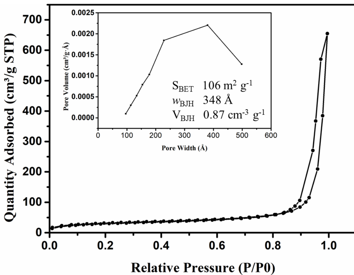
Figure A4.6 N 2 sorption isotherm and pore size distribution (inset) of R1 silica particles.
