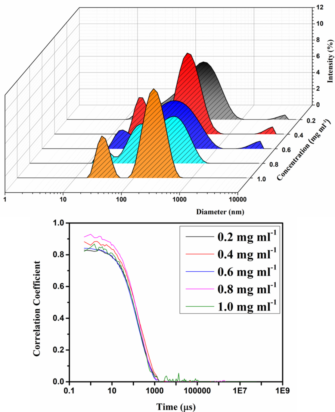
Figure 4.2 DLS measurements of sodium caseinate in acetate buffer (0.05 M, pH 5.94) at various concentrations (top). Correlograms (bottom).
