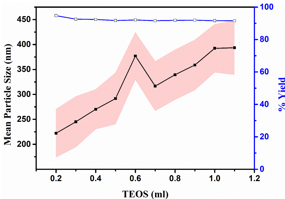
Figure 2.6 Effect of TEOS volume on mean particle size (—■—) and percent yield (—□—). Red shaded area is the standard deviation of mean particle size.
