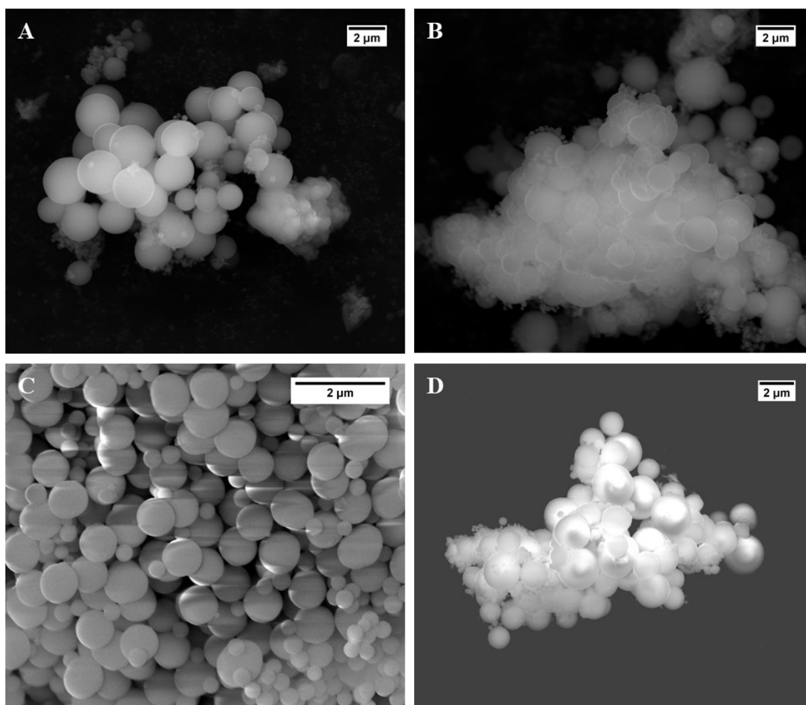
Figure 3.2 SEM micrographs of silica particles produced using phosphatidylcholine. (a) 0.02 \text{ mg ml}^{-1} PC (PC1), (b) 0.1 \text{ mg ml}^{-1} PC (PC2), (c) 0.2 \text{ mg ml}^{-1} PC (PC3), and (d) 0.4 \text{ mg ml}^{-1} PC (PC4). All reactions done in 50 ml soybean oil with 500 \mu\text{L} sodium silicate at room temperature. Scale bars are 2 \mu\text{m} .
