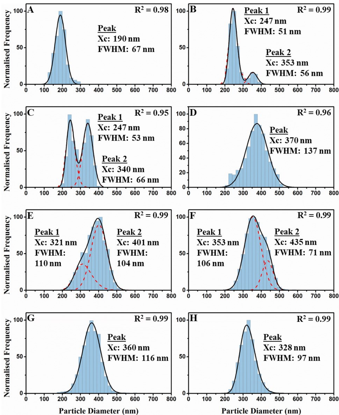
Figure 2.11 PSDs of silica nanoparticles synthesised by varying amount of water. (a) 0.4 ml H 2 O, (b) 0.5 ml H 2 O, (c) 0.6 ml H 2 O, (d) 0.7 ml H 2 O, (e) 0.8 ml H 2 O, (f) 0.9 ml H 2 O, (g) 1 ml H 2 O, and (h) 1.1 ml H 2 O.
