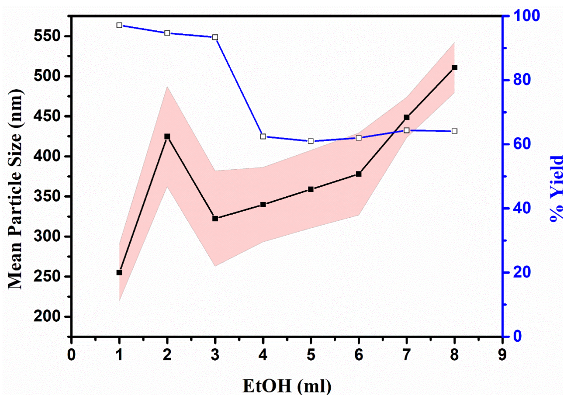
Figure 2.3 Effect of ethanol volume on mean particle size (—■—) and percent yield (—□—). Red shaded area is the standard deviation of mean particle size.
