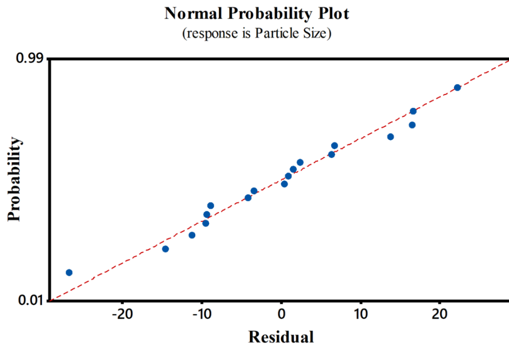
Figure A4.4 Normal probability plot of residuals (response is particle size).
