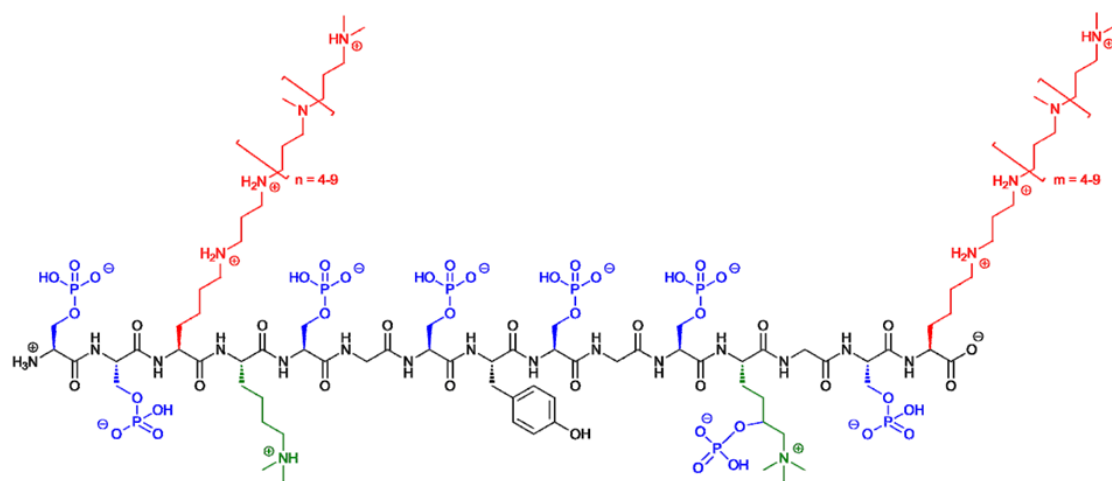
Figure 1.5 Chemical structure of native silaffin-1A 1 from C. fusiformis . Reproduced from Kröger et al. 106
