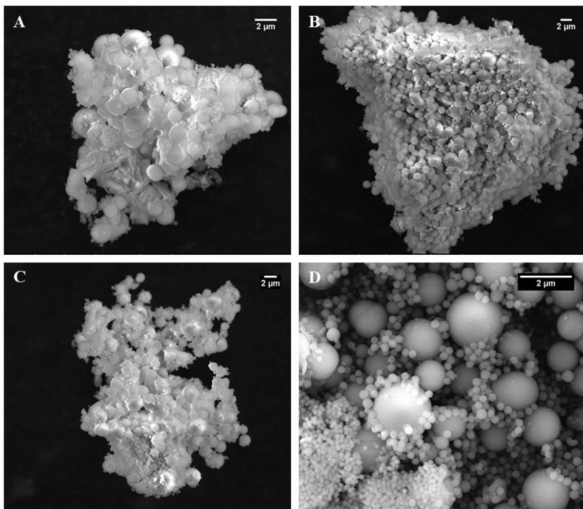
Figure 4.1 SEM micrographs (a) NC1 and (b) NC2, (c) NC3, and (d) NC4. T = 50^{\circ}\text{C} .
