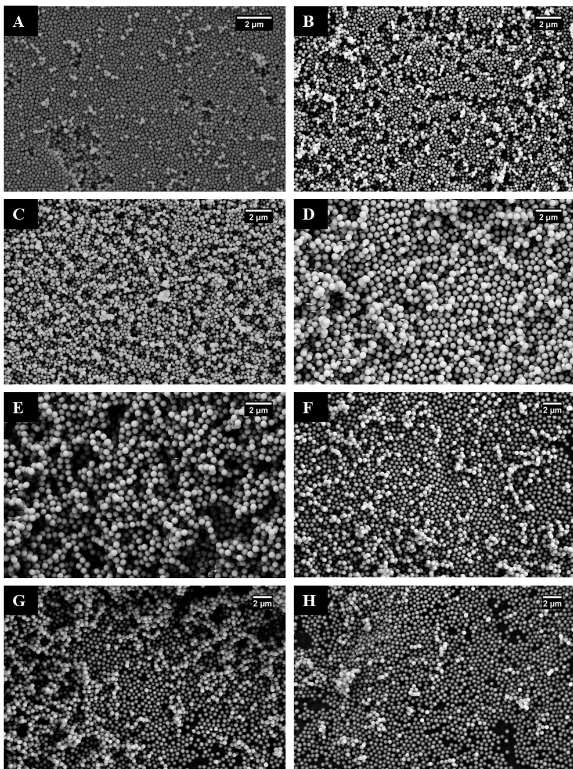
Figure 2.10 SEM images of silica nanoparticles synthesised by varying amount of water. (a) 0.4 ml H_2O , (b) 0.5 ml H_2O , (c) 0.6 ml H_2O , (d) 0.7 ml H_2O , (e) 0.8 ml H_2O , (f) 0.9 ml H_2O , (g) 1 ml H_2O , and (h) 1.1 ml H_2O .
