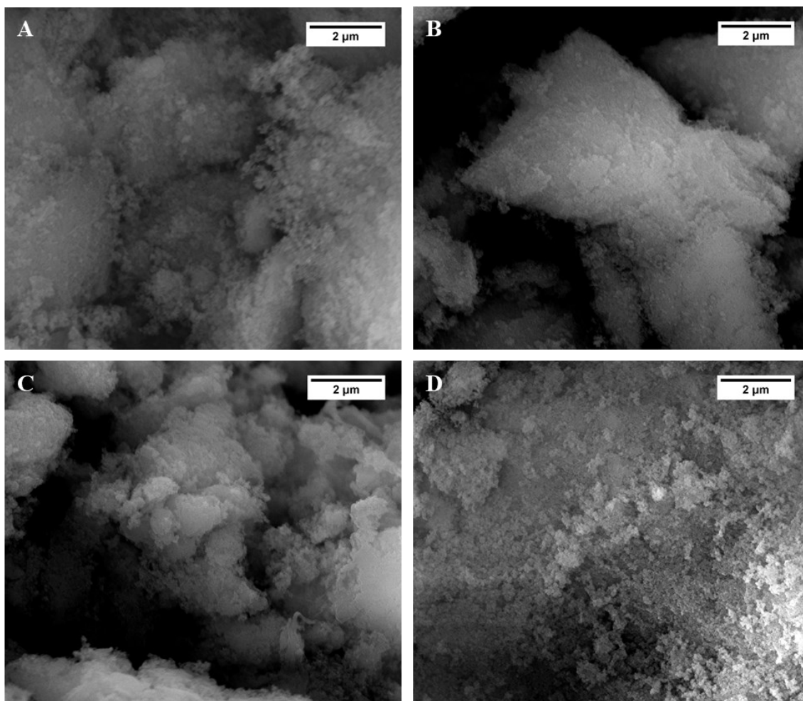
Figure 4.11 SEM micrographs of silica prepared with (a) 40 mg NaCas (BC1), and (b) 80 mg NaCas (BC2), (c) 120 mg NaCas (BC3), and (d) 160 mg NaCas (BC4). Scale bars = 2 \mu m. All other reactants kept constant.
