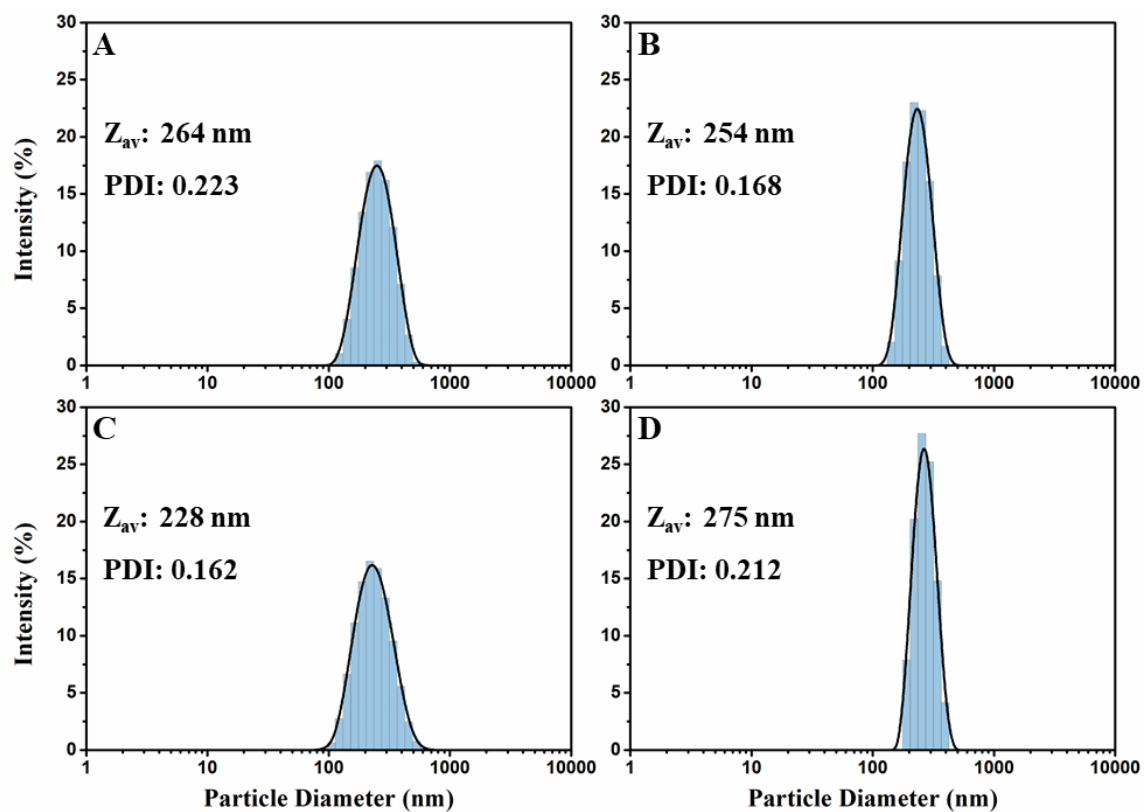
Figure 4.12 PSDs from DLS measurements of silica prepared with (a) 40 mg NaCas (BC1), and (b) 80 mg NaCas (BC2), (c) 120 mg NaCas (BC3), and (d) 160 mg NaCas (BC4). All reactions used 729 \mu\text{L} sodium silicate and 8 mM \text{CaCl}_2 , in 50 ml acetate buffer (0.05 M, pH 4.94).
