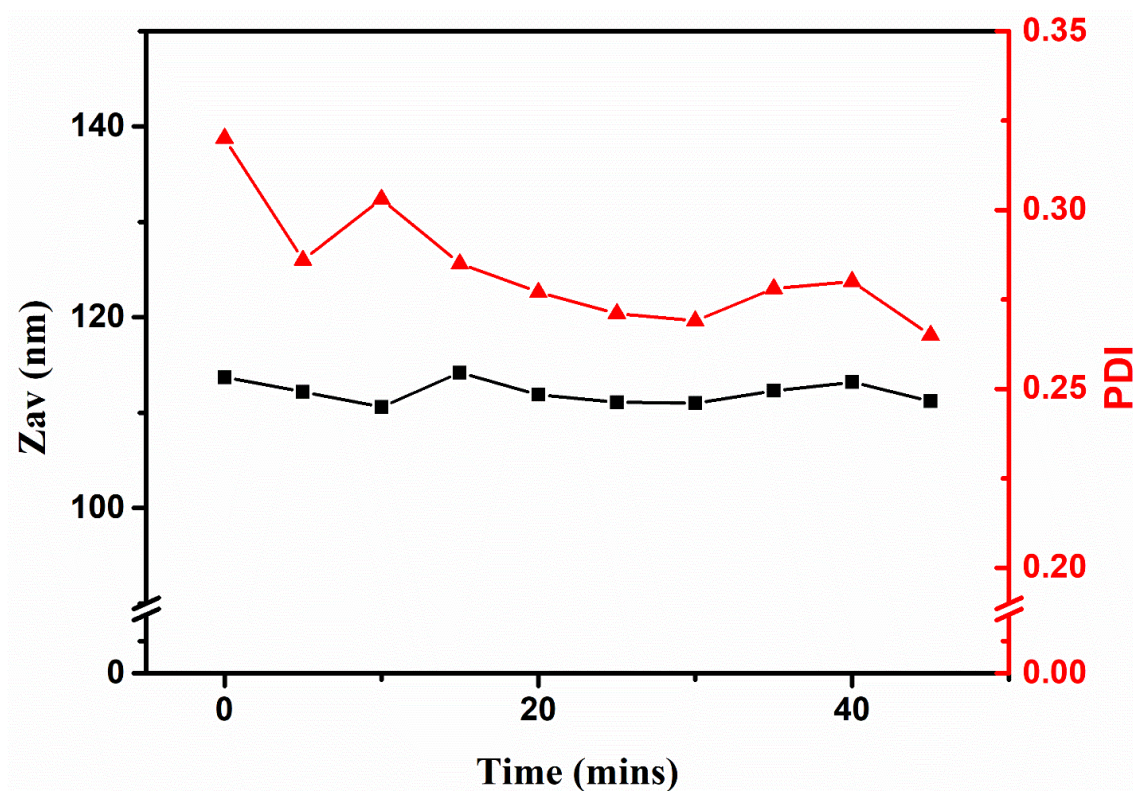
Figure A3.5 Temporal evolution of Z-average (■) and PDI (▲) of 0.1 \text{ mg ml}^{-1} SL in acetate buffer ( 0.05\text{M} , \text{pH } 5.92 ) with 10 \mu\text{L} sodium silicate.
