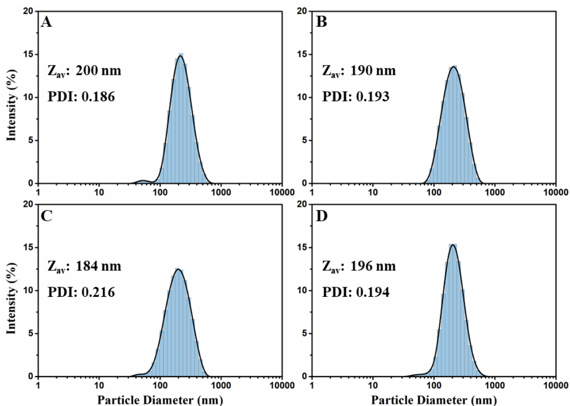
Figure 4.9 PSDs from DLS measurements of silica particles prepared with (a) 486 \mu L sodium silicate (R1), (b) 567 \mu L sodium silicate (R2), (c) 648 \mu L sodium silicate (R3), and (d) 729 \mu L sodium silicate (R4). All reactions used 20 mg NaCas and 8 mM \text{CaCl}_2 , in 50 ml acetate buffer (0.05 M, pH 5.94).
