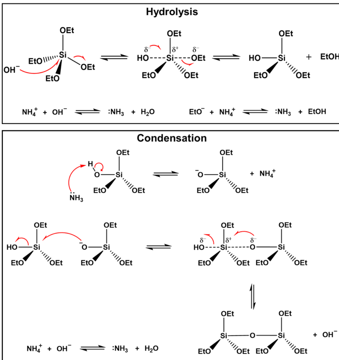
Scheme 1.1 Mechanism of hydrolysis and condensation of TEOS in the presence of ammonia (Stöber process). TEOS is hydrolysed to give the oligomeric precursor species. Note that the hydrolysed precursor shown here is only one of the possible structures formed. For a more detailed description of these intermediaries, see Trinh et al. 54 Condensation of these oligomers leads to the generation of small primary seed/sub-particles. These nucleation events precede the formation of the final particles. The final particles are formed typically via coalescence and/or Ostwald ripening of the seed particles. Mechanism adapted from Ghimire et al. 53
