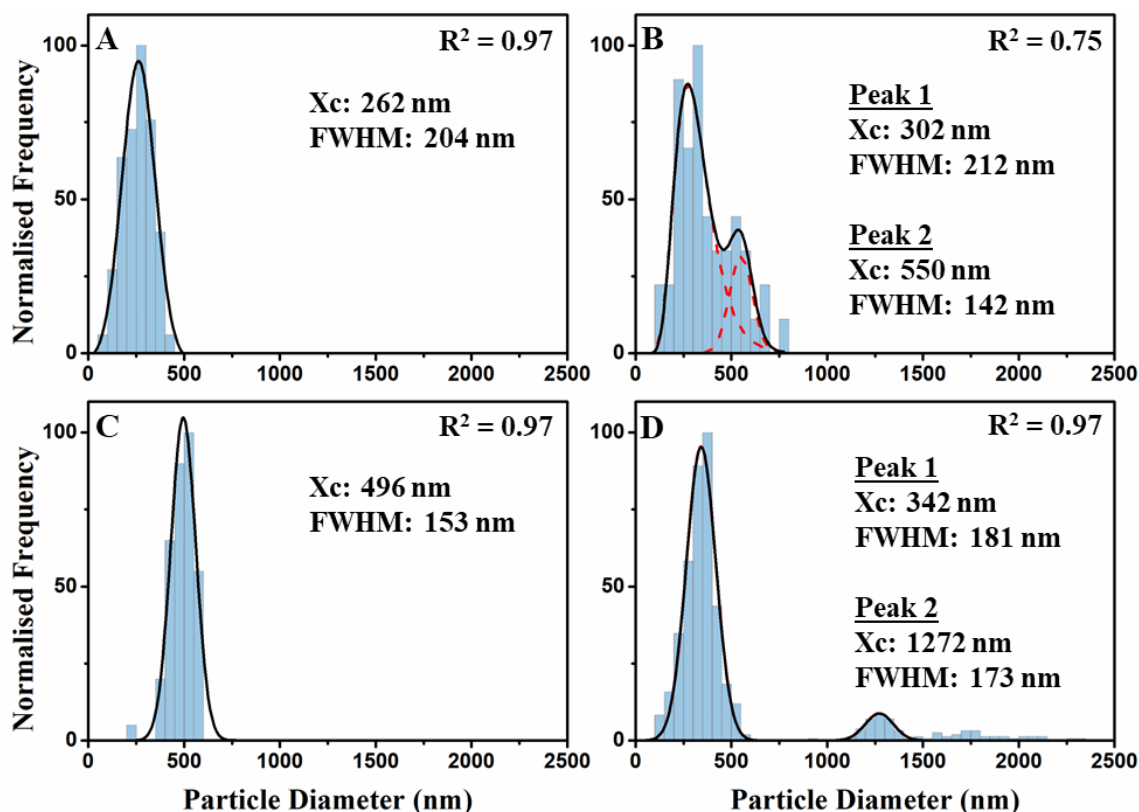
Figure 3.5 PSDs of silica particles produced using soy lecithin (a) 0.004 \text{ mg mL}^{-1} SL (SL1), (b) 0.04 \text{ mg mL}^{-1} SL (SL2), (c) 0.08 \text{ mg mL}^{-1} PC (SL3), and (d) 1.8 \text{ mg mL}^{-1} SL (SL4). All reactions done in 50 ml acetate buffer (0.05M, pH 5.92) with 820 \mu\text{L} sodium silicate at room temperature.
