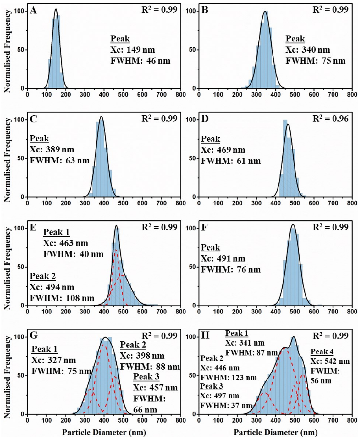
Figure 2.8 PSDs of silica nanoparticles prepared by varying amount of ammonia. (a) 1.2 M \text{NH}_4\text{OH} , (b) 2.2 M \text{NH}_4\text{OH} , (c) 3.1 M \text{NH}_4\text{OH} , (d) 3.8 M \text{NH}_4\text{OH} , (e) 4.5 M \text{NH}_4\text{OH} , (f) 5.1 M \text{NH}_4\text{OH} , (g) 5.6 M \text{NH}_4\text{OH} , and (h) 6.1 M \text{NH}_4\text{OH} . All other reactants kept constant.
