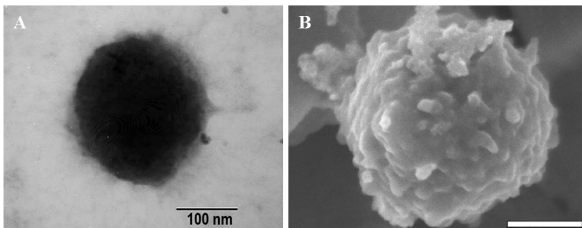
Figure A4.1 Structure of casein micelle. (a) Transmission electron micrograph of freeze-dried poly-L-lysine immobilised casein micelle fixed with glutaraldehyde (from McMahon et al. 46 ) (b) Electron micrograph of an individual casein micelle, scale bar = 100 nm. (from Dagleish et al. 47 )
