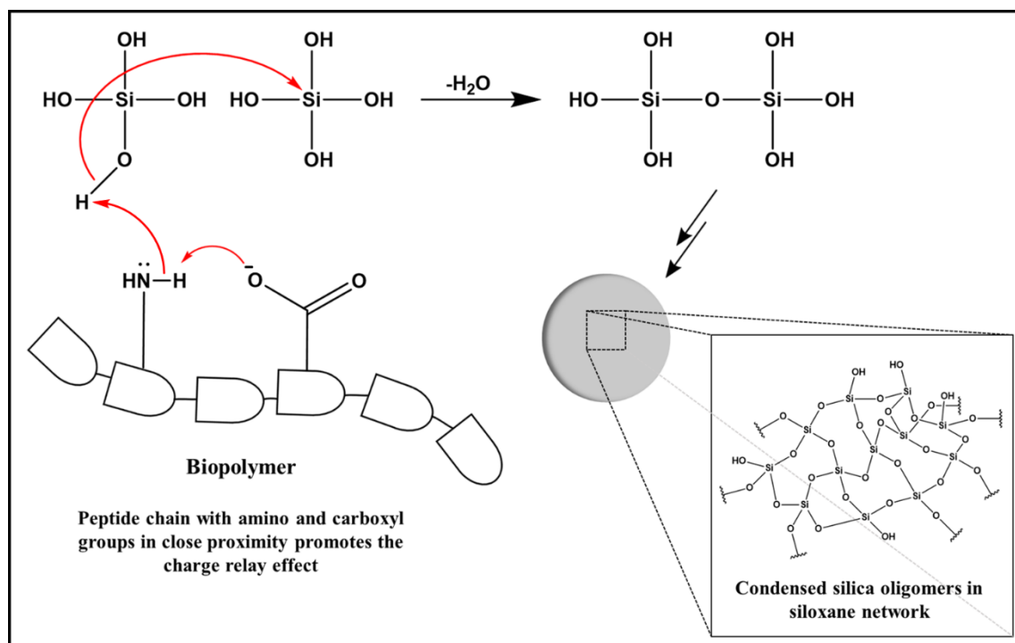
Scheme 1.2 Charge relay effect in biosilica synthesis. Here the peptide chain of the biopolymer has amino and carboxyl groups in close proximity, which is the case for many biopolymers. The oxygen of the carboxyl group hydrogen bonds to the hydrogen of the amino acid group. This pulls electron density away from the nitrogen. The lone pair on the nitrogen then activates the nucleophile, in this case a silicic acid molecule. This starts the condensation process. The silicic acid monomers condense to form a siloxane network which results in the formation of silica. The biopolymer can also act as an SDA, which can promote the formation of spherical silica particles, represented here by the grey sphere.
