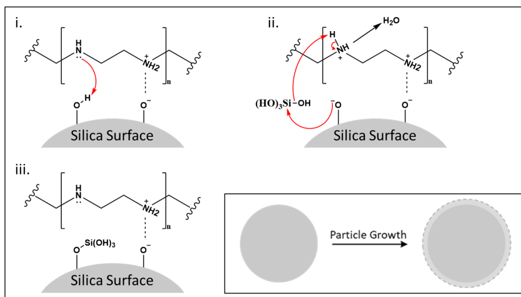
Scheme 1.3 Simplified mechanism of silica particle growth in the presence of polyamines. Polyamine is attracted to the silica surface electrostatically (represented by dashed line). (i) Lone pair of electrons on uncharged amine deprotonates a silanol in close proximity. (ii) This deprotonated silanol attacks a free silicic acid molecule via S_N2 mechanism, with OH^- as the leaving group. The OH^- then attacks the protonated amine group, releasing water and reforming the uncharged amine. (iii.) Silicic acid derivative is attached to the surface. The process repeats, adding more silicate to the surface and the particle grows. Image on lower right represents this surface growth. Dark grey is the original particle, light grey is additional silica added by growth process. Dashed line around particle illustrates an increased diameter.
