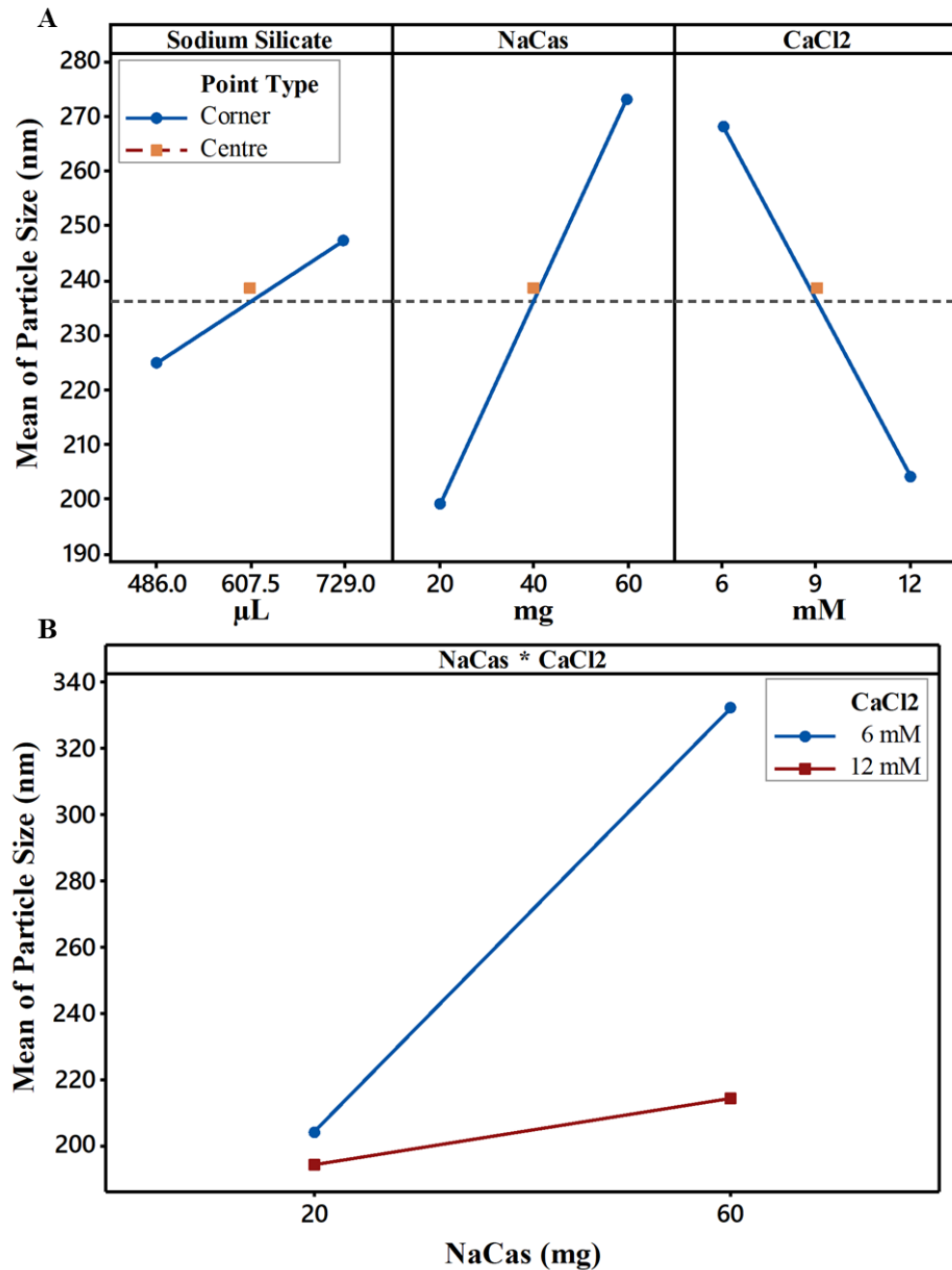
Figure 4.7 (a) Main effects plots of sodium silicate, sodium caseinate, and calcium chloride and their effect on particle size. Differences between level means are shown for each factor level and are connected by a line. Orange squares are the mean response for the centre point runs. A non-horizontal line indicates a main effect is present. Dashed horizontal line shows the mean particle size for all runs (b) Interaction plot for particle size (fitted means). Non-parallel lines indicate that an interaction effect is occurring. The relationship between particle size and sodium caseinate depends on the concentration of calcium chloride.
