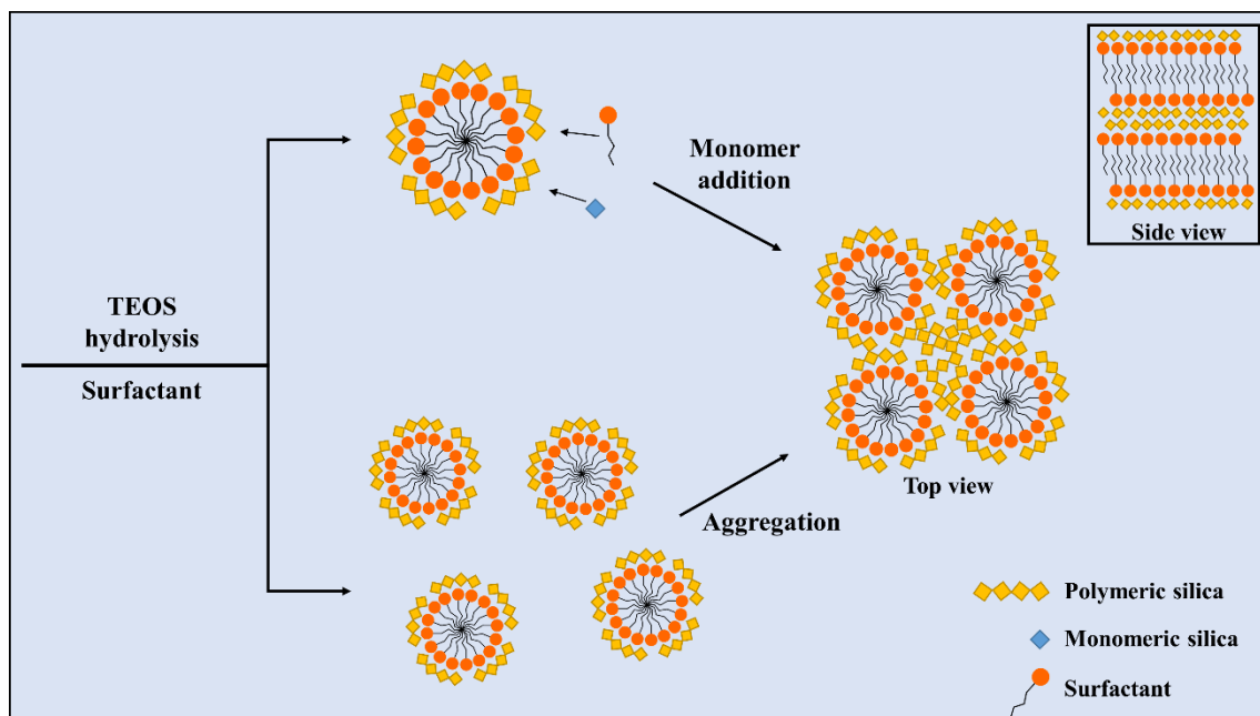
Figure 1.3 Proposed mechanisms for the formation of surfactant-templated silica. The upper pathway corresponds to a monomeric silica addition mechanism. The lower pathway corresponds to aggregation of seed particles to form larger particles. Adapted from Nooney et al. 61
