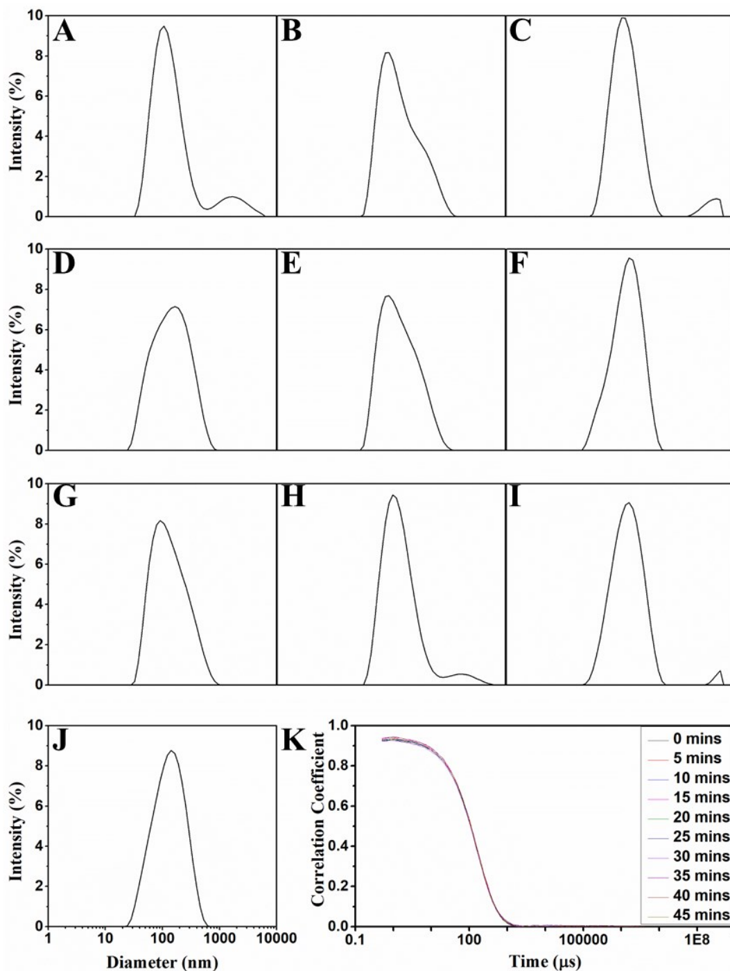
Figure A3.6 Temporal PSD data from DLS measurements of 0.1 \text{ mg ml}^{-1} soy lecithin in acetate buffer ( 0.05 \text{ M} , \text{pH } 5.92 ) with 10 \text{ } \mu\text{L} sodium silicate. (a) 0 mins after sodium silicate addition, (j) 45 mins after sodium silicate addition, increment is 5 mins. (k) Correlograms for a-j. As time increases, the distribution becomes unimodal, showing the effect that added sodium silicate has on the SL stability.
