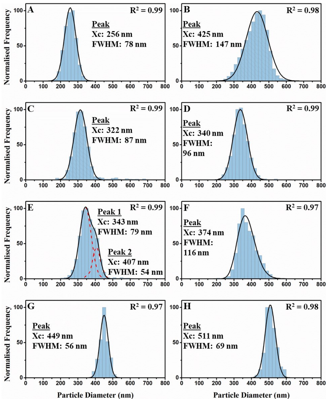
Figure 2.2 PSDs of silica nanoparticles synthesised by varying amount of ethanol. (a) 1 ml EtOH, (b) 2 ml EtOH, (c) 3 ml EtOH, (d) 4 ml EtOH, (e) 5 ml EtOH, (f) 6 ml EtOH, (g) 7 ml EtOH, and (h) 8 ml EtOH. All other reactants kept constant.
