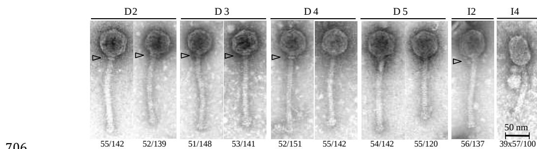
707 Fig. 2. Representative transmission electron micrographs of phages extracted from whey mixtures. 708 All the micrographs except I4 show 936-like phages (I4 is a c2-like phage). Arrowheads indicate 709 neck passage structures (NPS). Numbers below the micrographs are the head dimensions and tail 710 lengths of the phage particles, respectively. Micrographs are shown at identical magnifications 711 (bar=50 nm).
